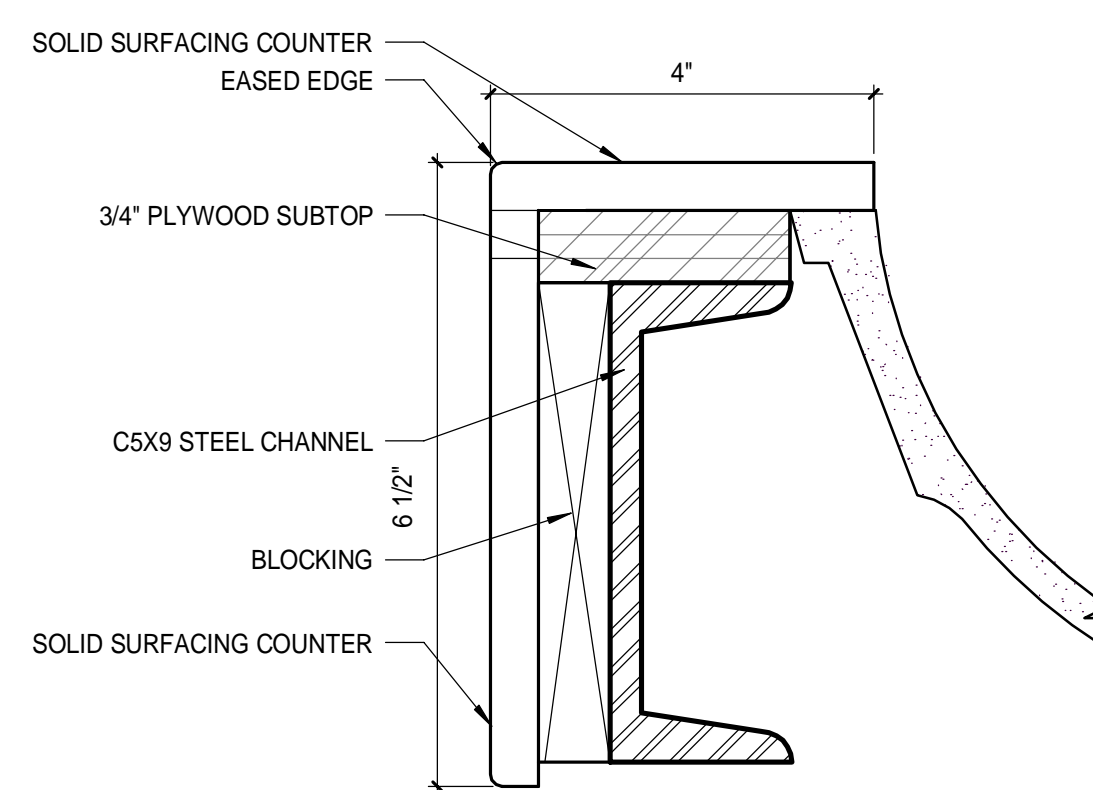
3 COUNTER EDGE DETAIL 6" = 1'-0"
