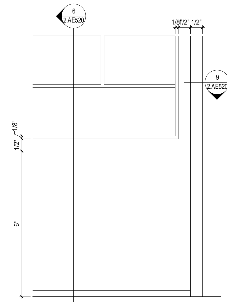
5 ELEV @ METAL BASE @ GLASS TILE 6" = 1'-0"
