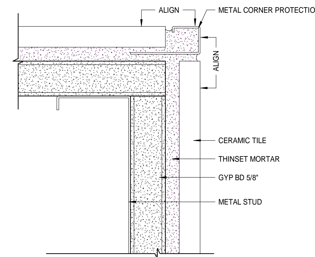
10 PLAN @ CT-02 OUTSIDE CORNER 12" = 1'-0"
