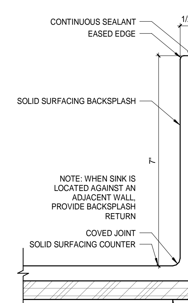
2 BACKSPLASH DETAIL 6" = 1'-0"
