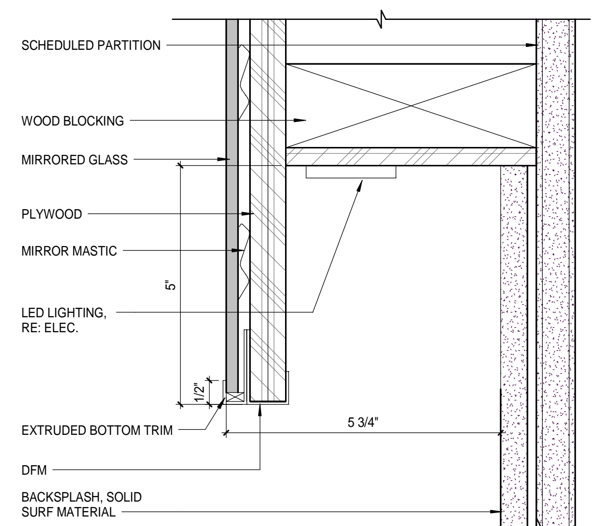
4 DETAIL @ MIRROR BASE 6" = 1'-0"
