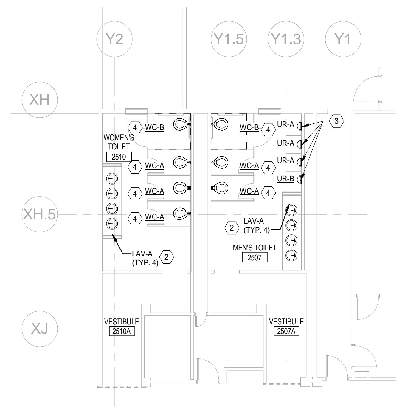
1 2ND FLOOR - PLUMBING RESTROOM PLAN 1/8" = 1'-0"
