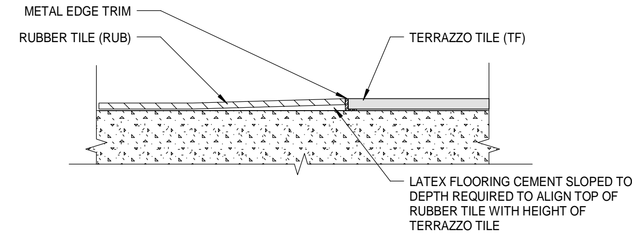
2 DETAIL - FLOORING TRANSITION 6" = 1'-0"
