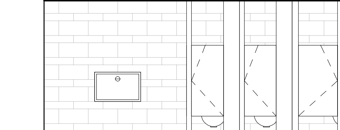
1 2ND FLOOR - MEN'S TOILET - WEST 1/4" = 1'-0"
