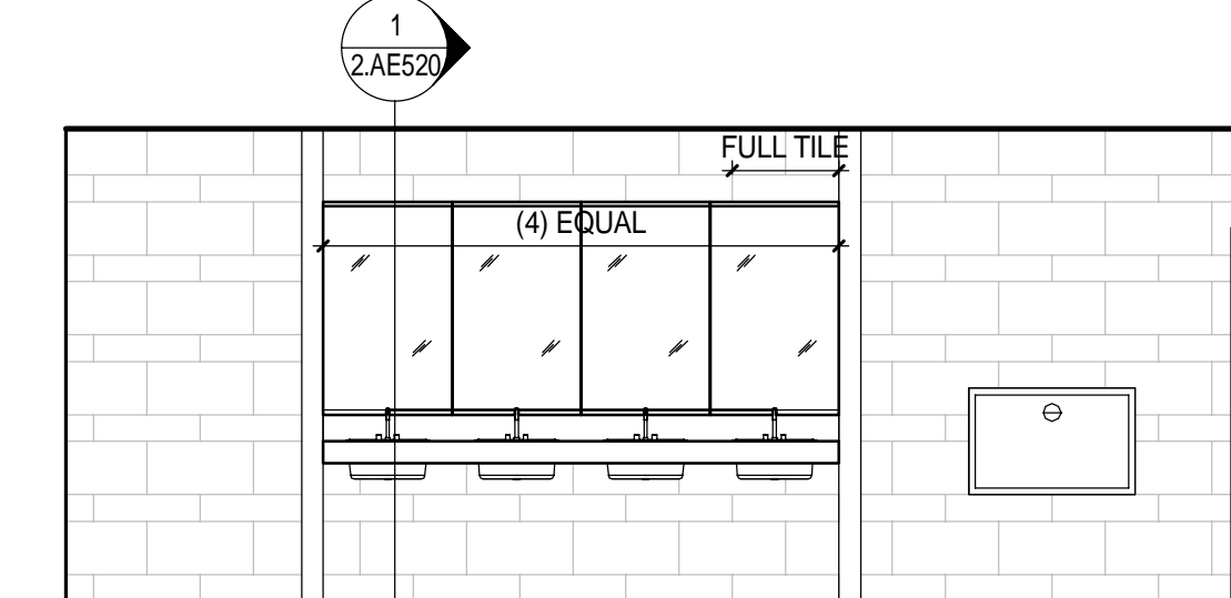
3 2ND FLOOR - WOMEN'S TOILET - WEST 1/4" = 1'-0"
