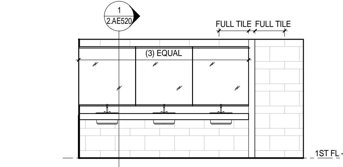
7 1ST FLOOR - WOMEN'S TOILET - EAST 1/4" = 1'-0"
