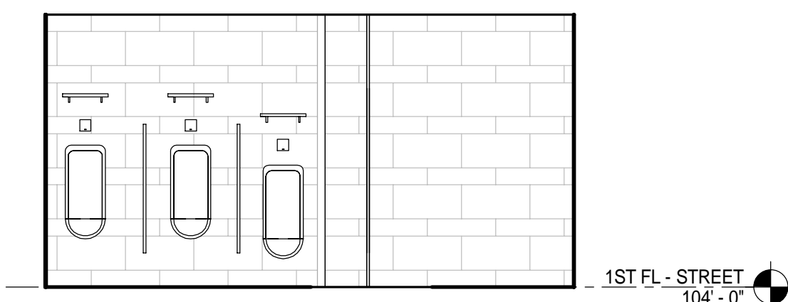
12 1ST FLOOR - MEN'S TOILET - NORTH 1/4" = 1'-0"
