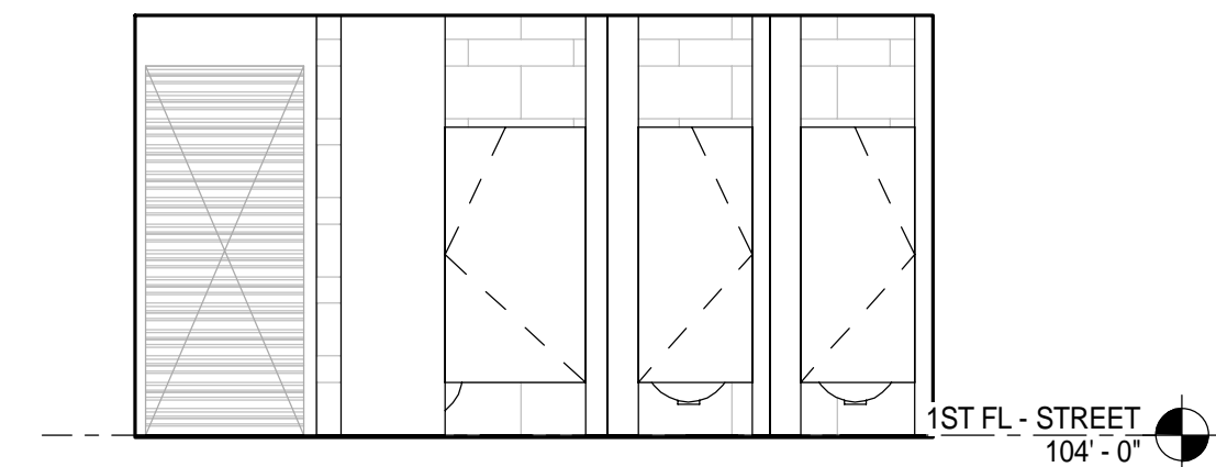
5 1ST FLOOR - WOMEN'S TOILET - WEST 1/4" = 1'-0"
