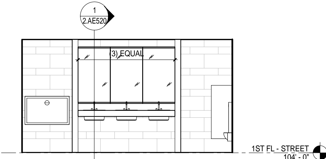
9 1ST FLOOR - MEN'S TOILET - WEST 1/4" = 1'-0"
