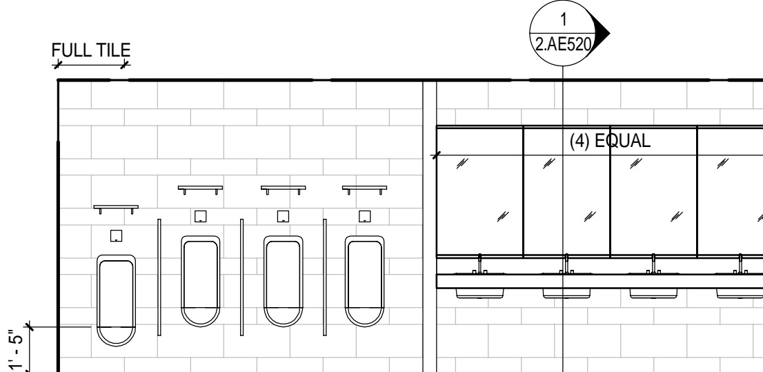
2 2ND FLOOR - MEN'S TOILET - EAST 1/4" = 1'-0"
