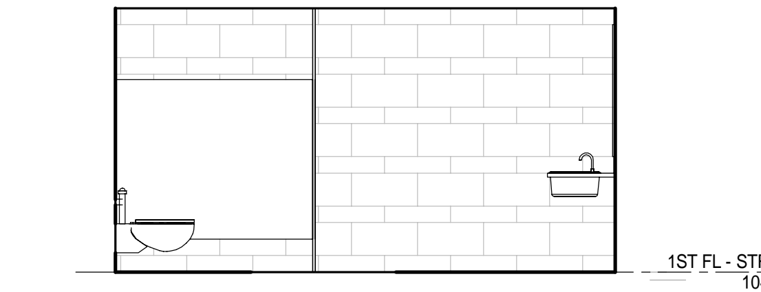
8 1ST FLOOR - WOMEN'S TOILET - NORTH 1/4" = 1'-0"
