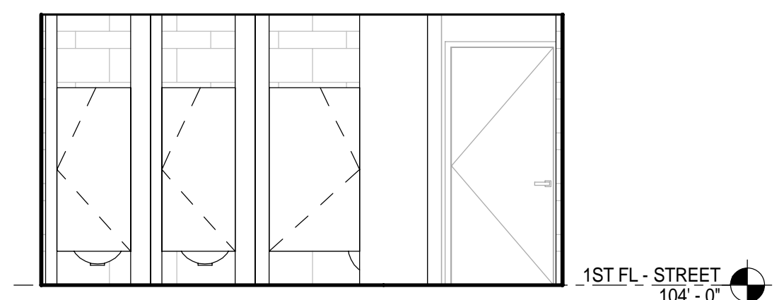
11 1ST FLOOR - MEN'S TOILET - EAST 1/4" = 1'-0"
