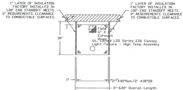
PLAN VIEW - Hood #1 2' 4.00" LONG 3044BD-2
