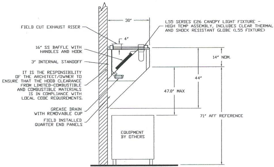
SECTION VIEW - MODEL 3044BD-2 HOOD - #1
