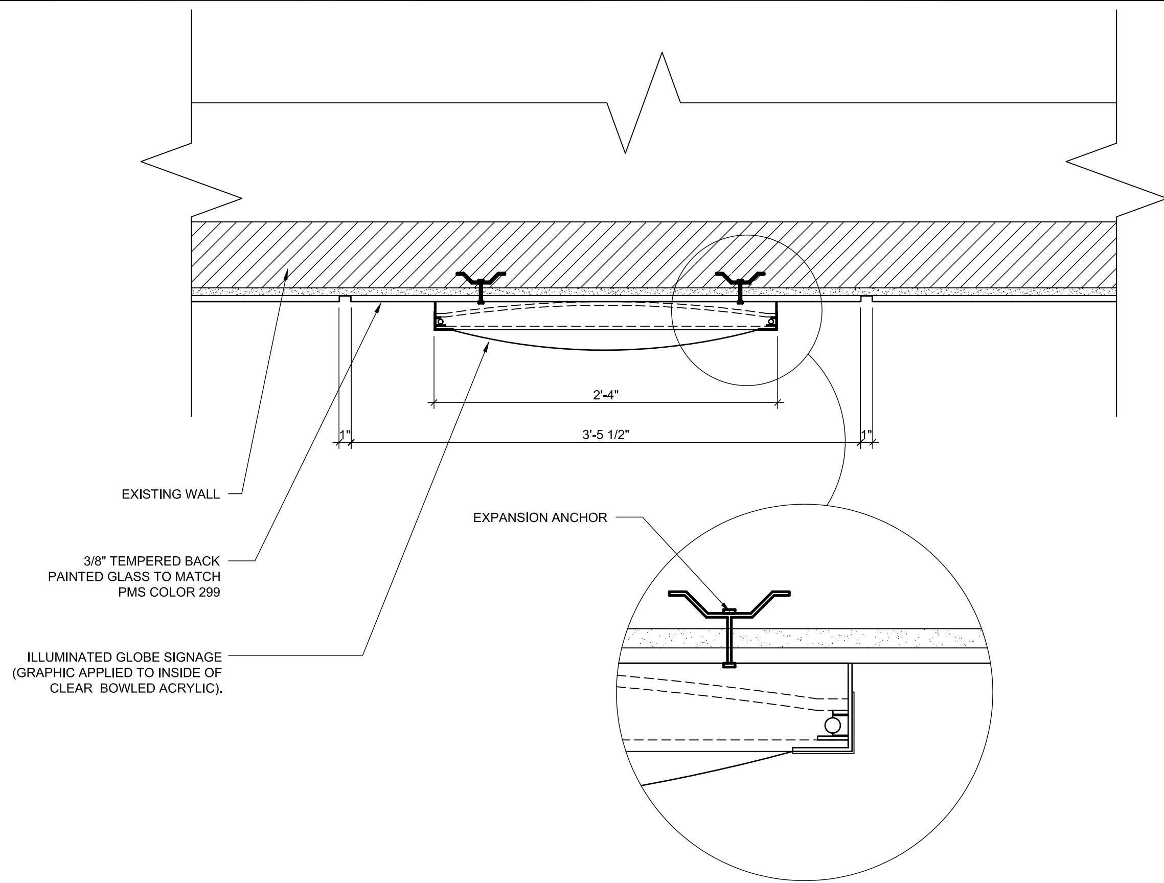
HORIZONTAL SECTION THRU GLOBE SIGN 1-1/2" = 1'-0" 4
