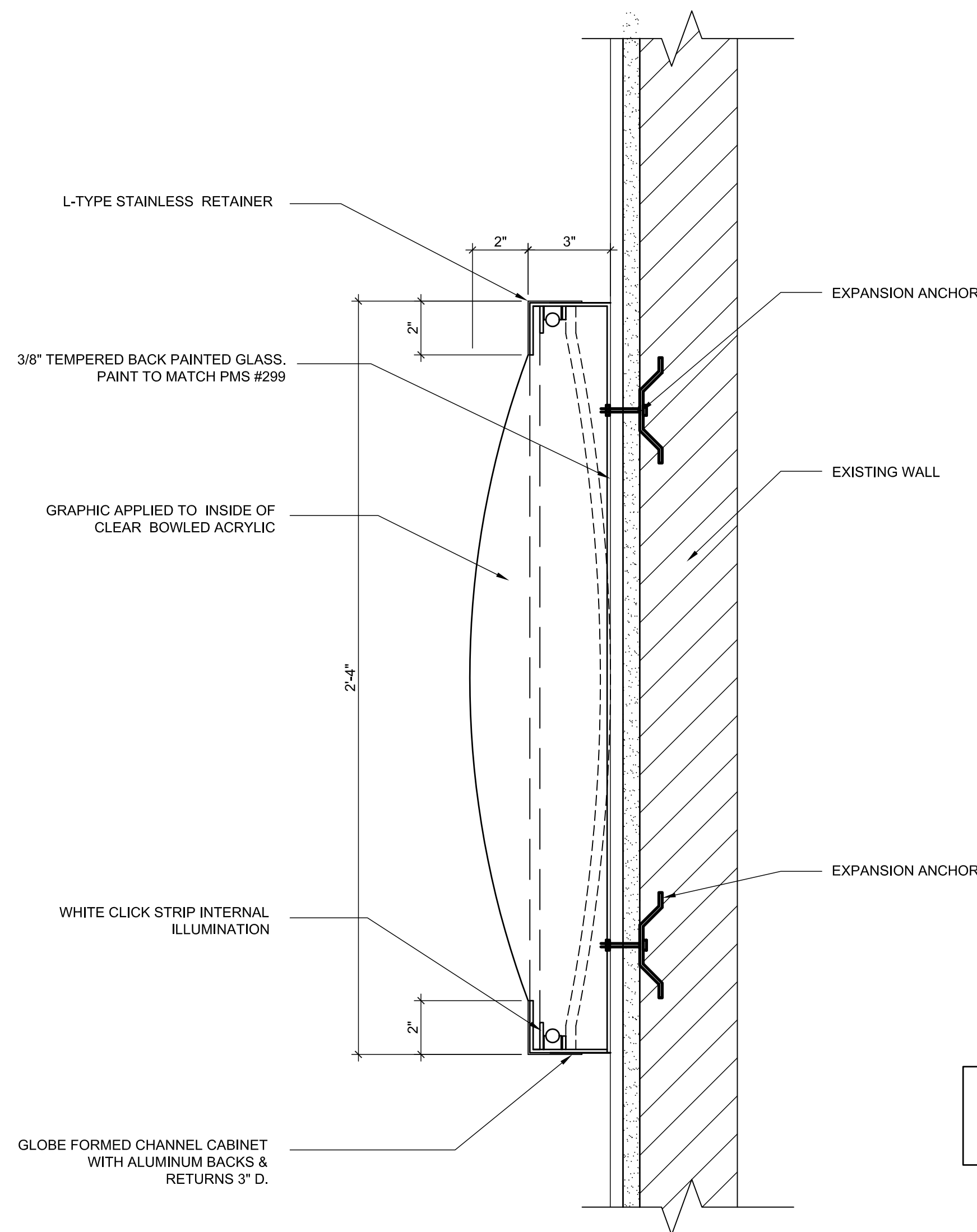
VERTICAL SECTION THRU GLOBE SIGN 3" = 1'-0" 3
