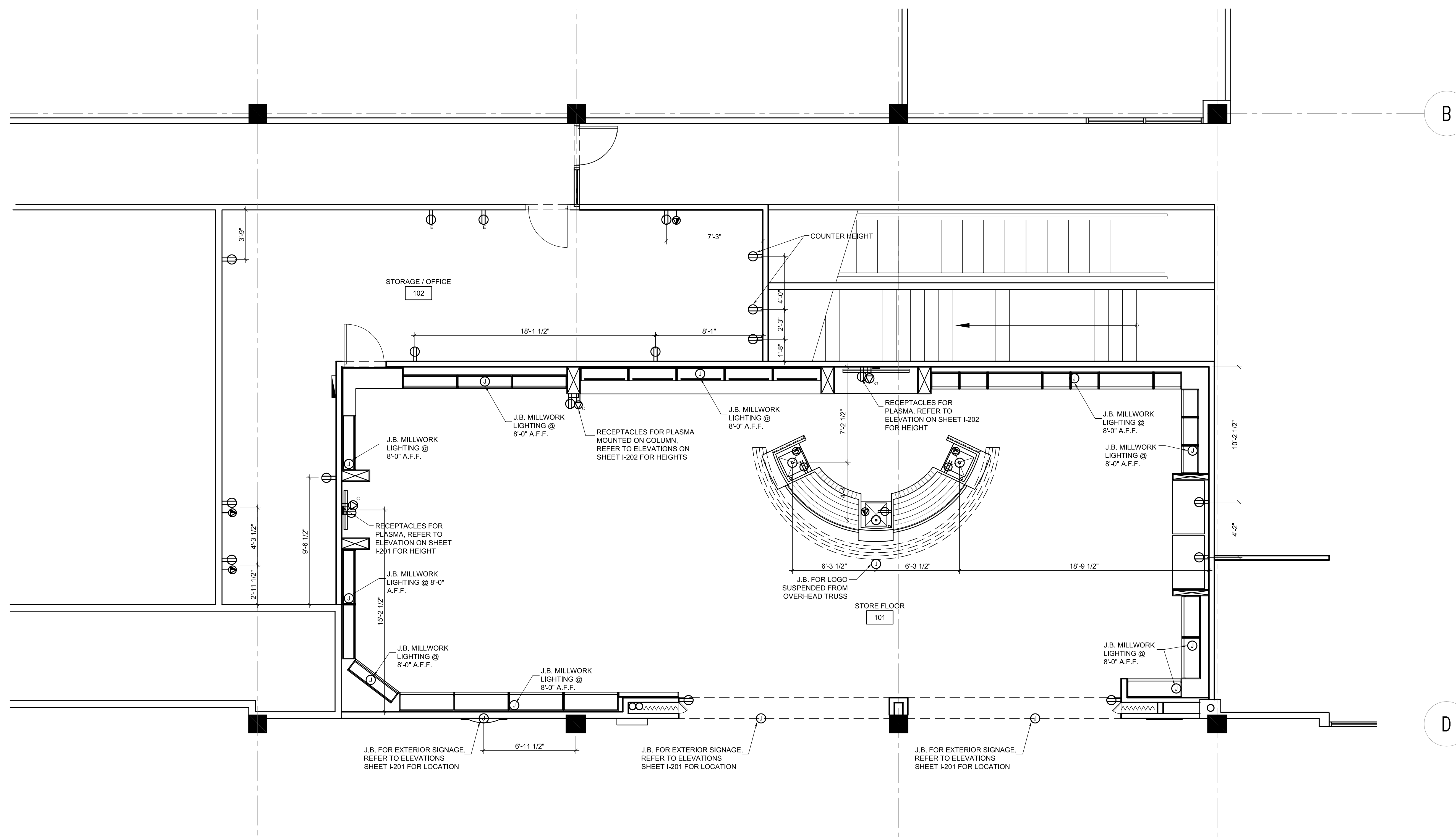
POWER & SIGNAL PLAN 1/4" = 1'-0" 1
