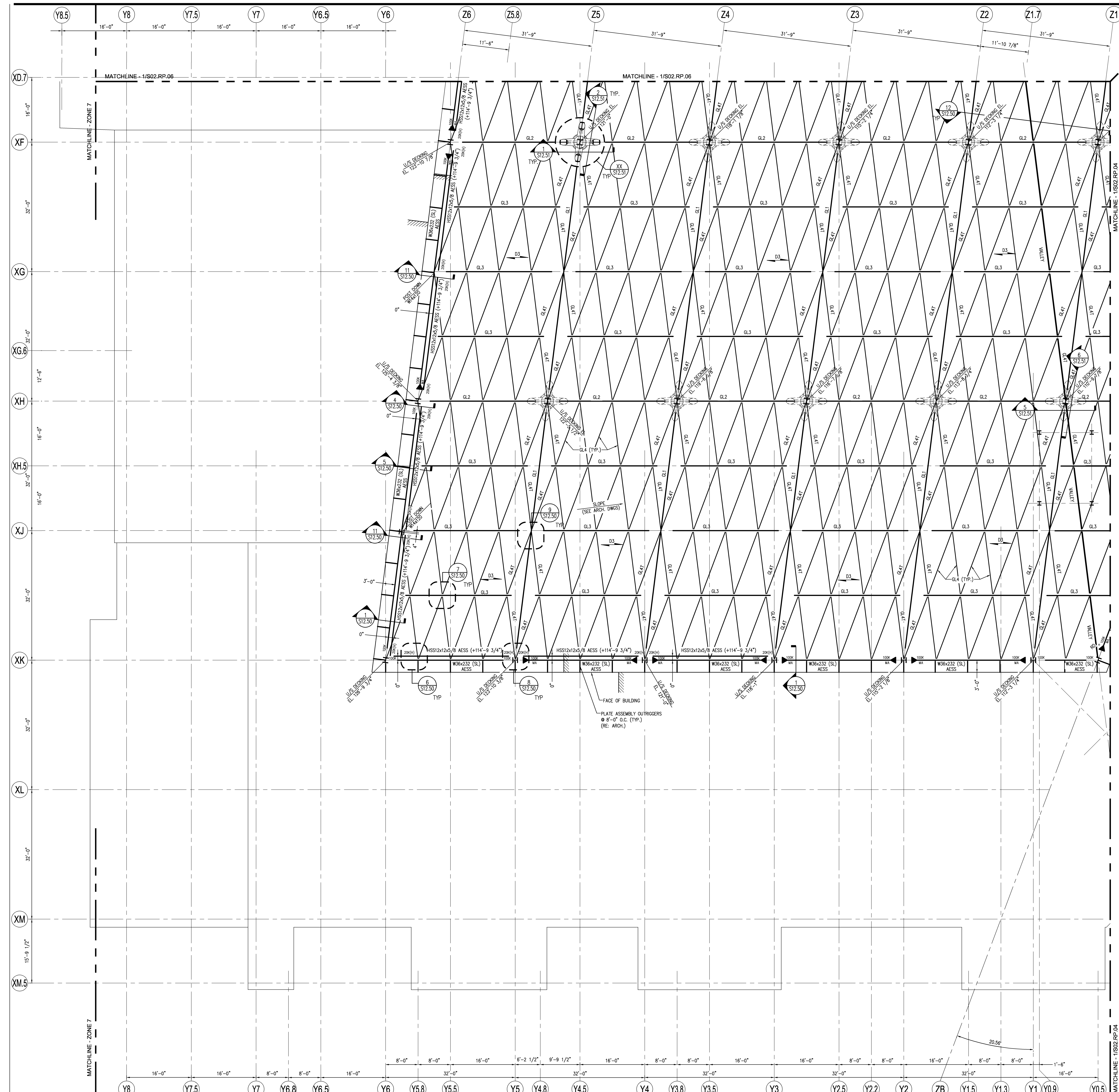
FRAMING PLAN - ROOF - ZONE 5 SCALE: 1/8" = 1'-0"
