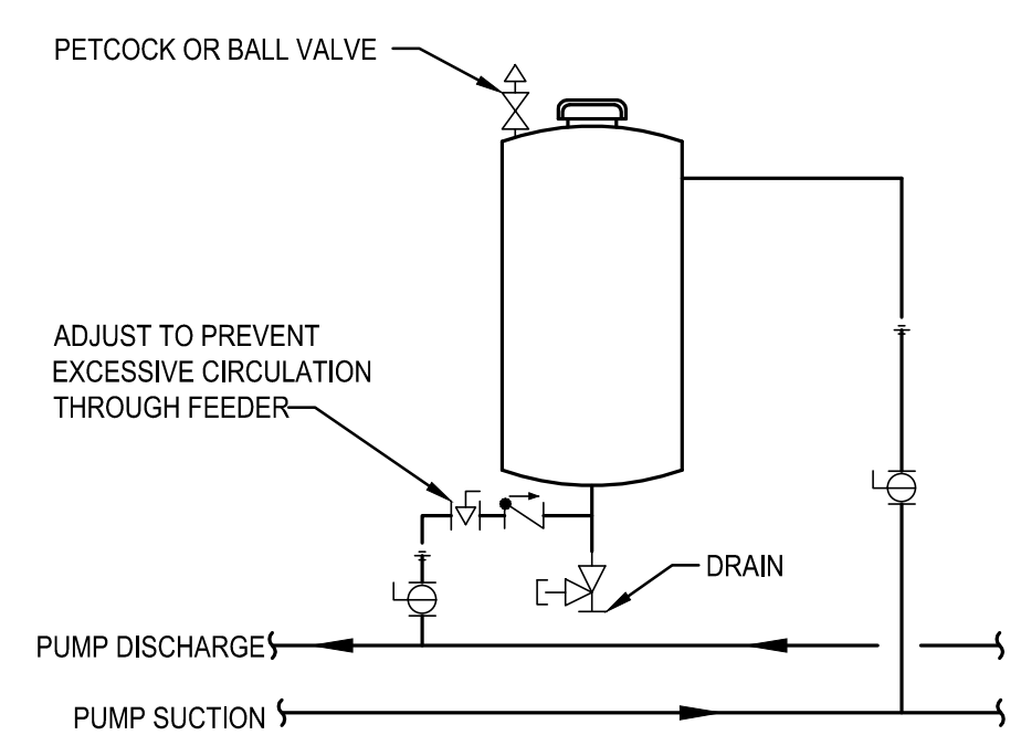
DETAIL - BYPASS CHEMICAL FEEDER 13 SCALE: NOT TO SCALE
