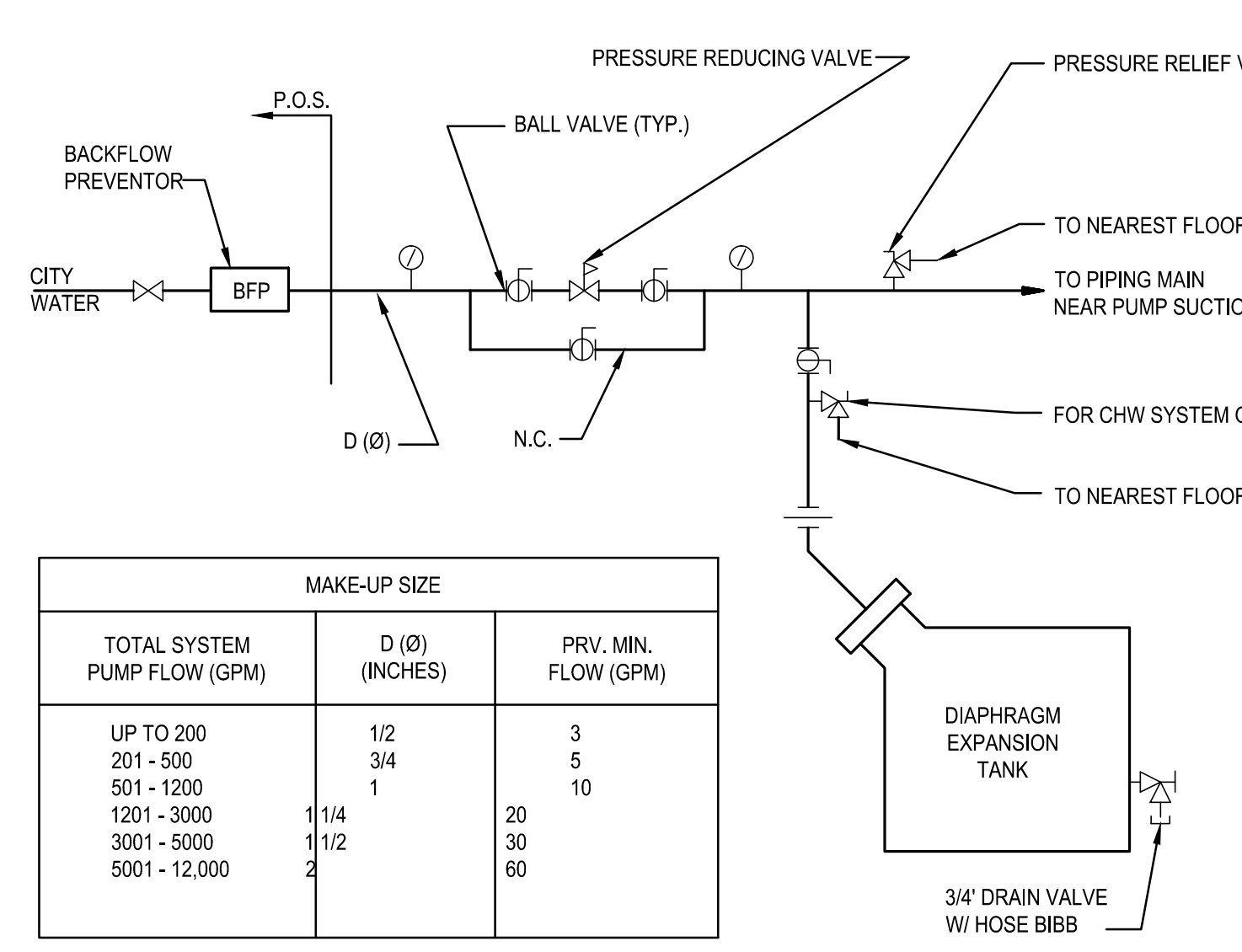
DETAIL - MAKE-UP WATER & DIAPHRAGM EXPANSION TANK 8 SCALE: NOT TO SCALE
