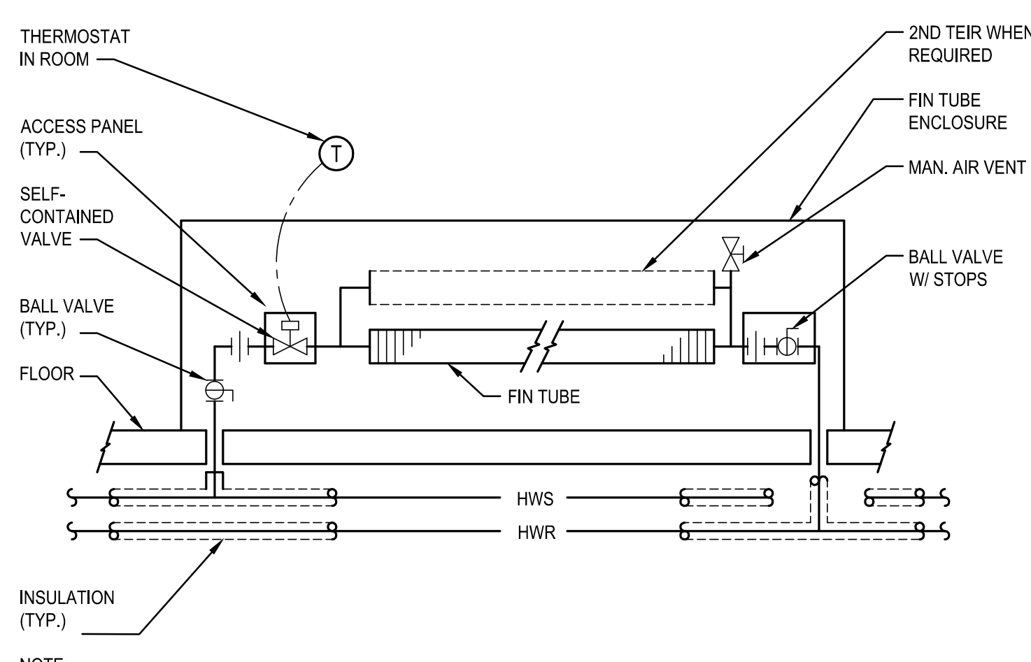
DETAIL - HOT WATER FTR PIPING 6 SCALE: NOT TO SCALE
