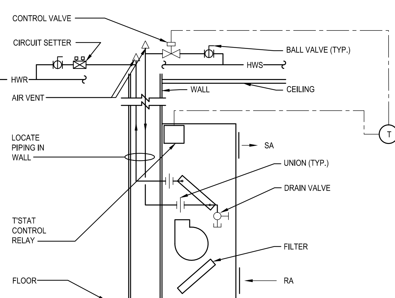
DETAIL - WALL CABINET UNIT HEATER 11 SCALE: NOT TO SCALE
