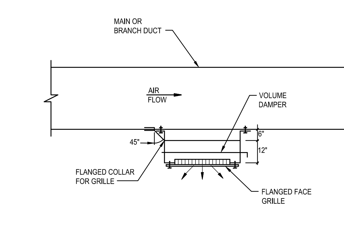
DETAIL - DUCT SUPPLY GRILLE TAKE OFF 3 SCALE: NOT TO SCALE
