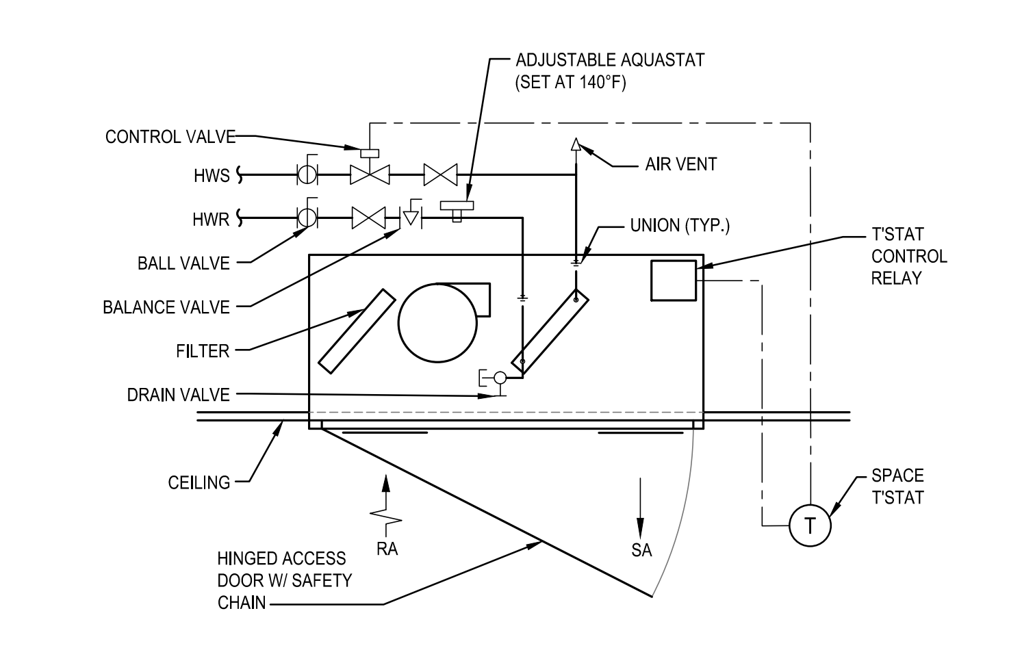
DETAIL - CEILING RECESSED CABINET UNIT HEATER 7 SCALE: NOT TO SCALE
