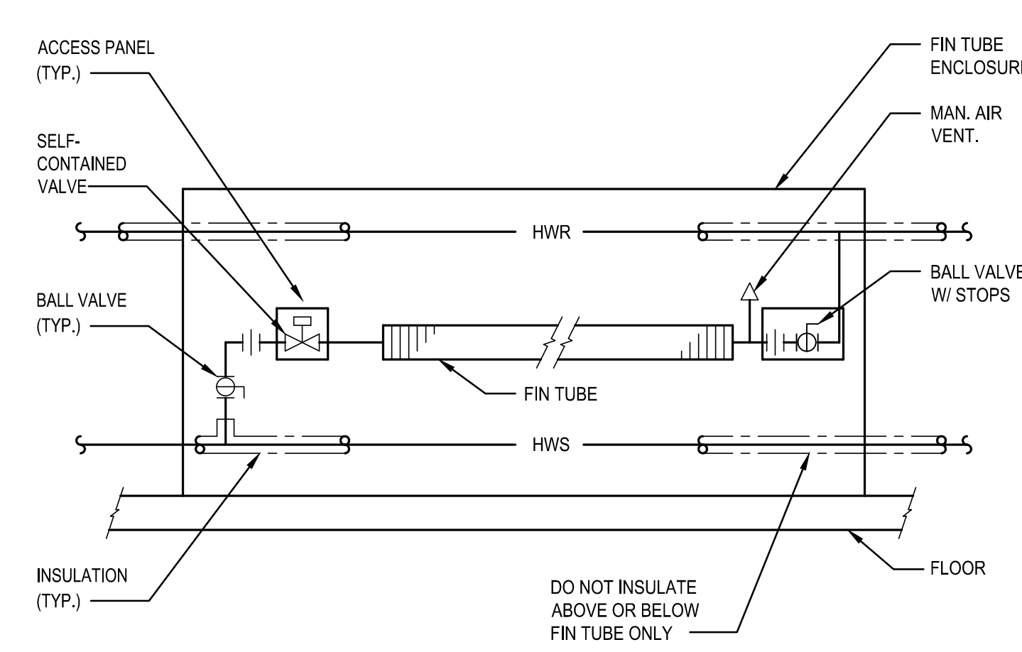
DETAIL - HOT WATER FTR PIPING 2 SCALE: NOT TO SCALE
