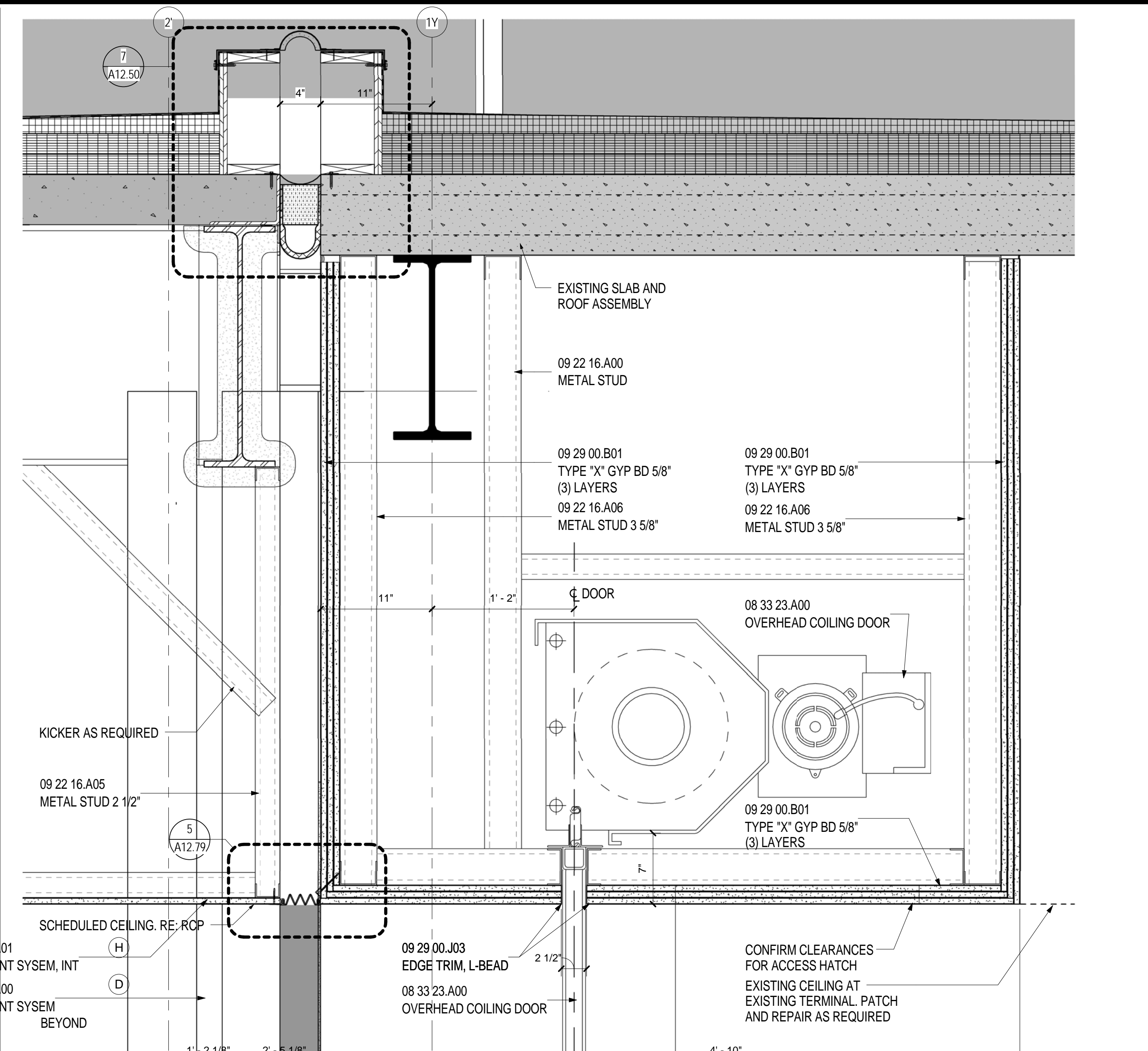
FIRE SHUTTER DETAIL - LEVEL 3 SCALE: 1 1/2" = 1'-0" A04.03.02 1
