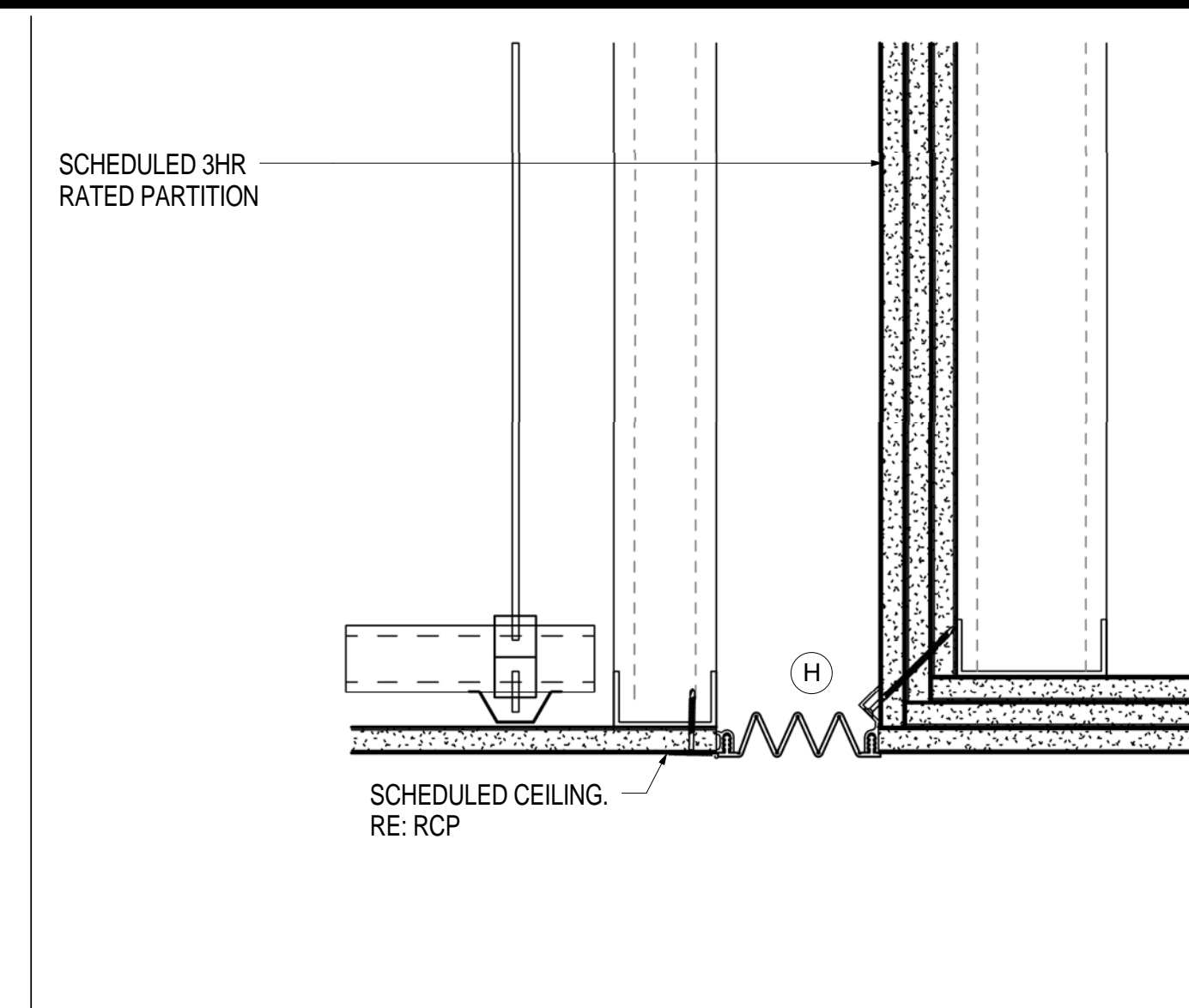
EXPANSION JT LEVEL 2 CEILING SCALE: 3" = 1'-0" A12.79 4
