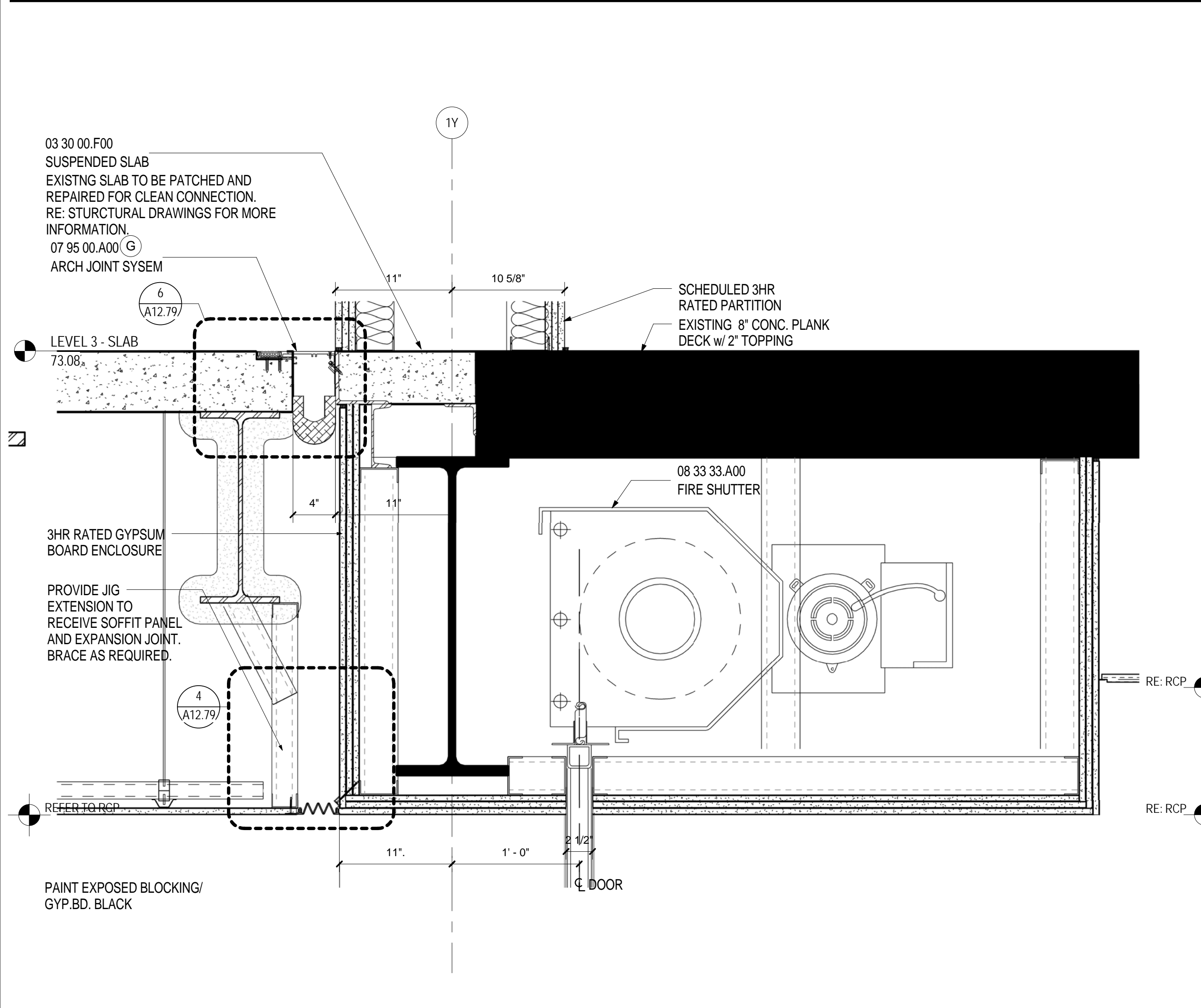
FIRE SHUTTER DETAIL - LEVEL 3 SCALE: 1 1/2" = 1'-0" A04.03.02 1
