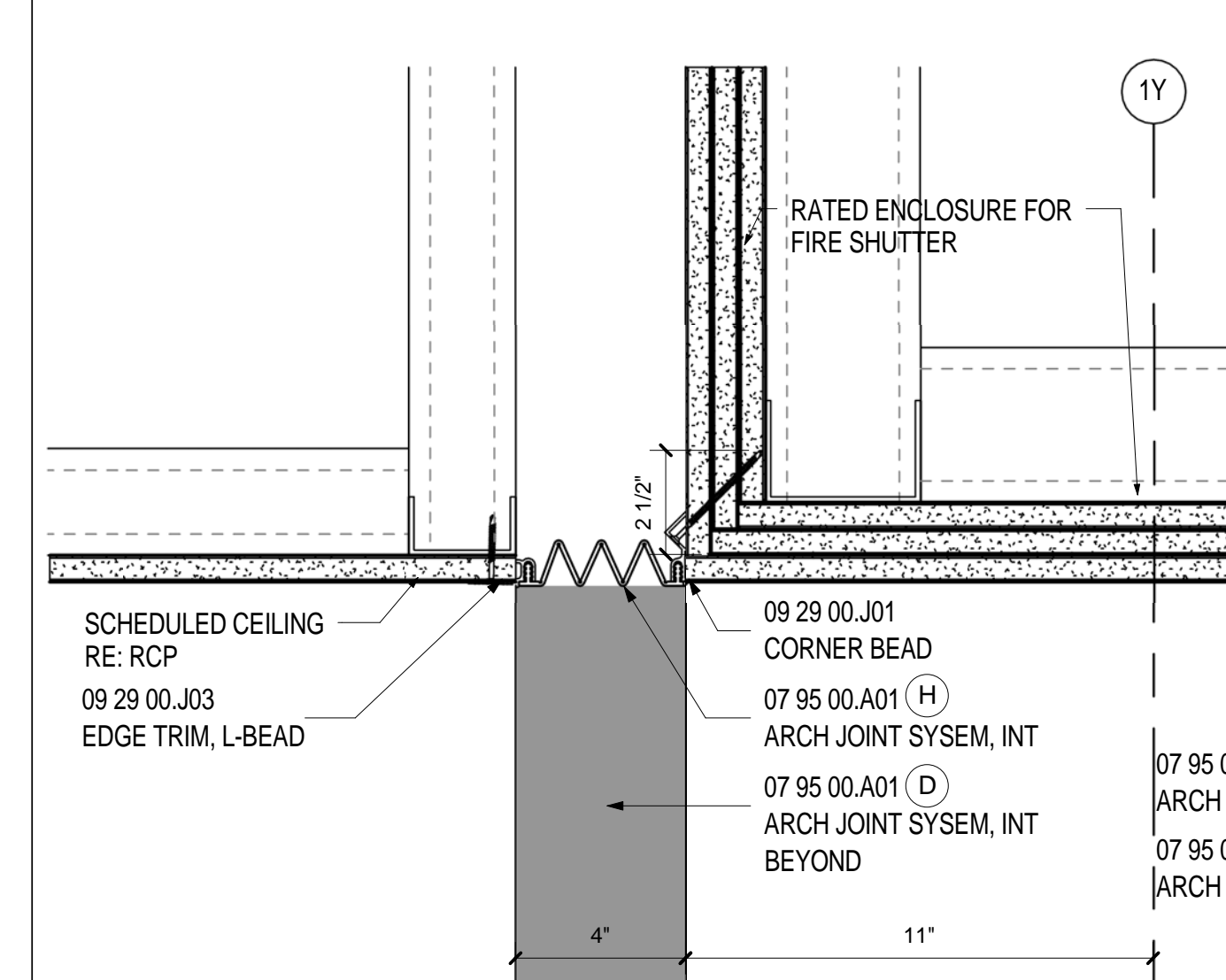
EXPANSION JT LEVEL 3 CEILING SCALE: 3" = 1'-0" A12.79 5
