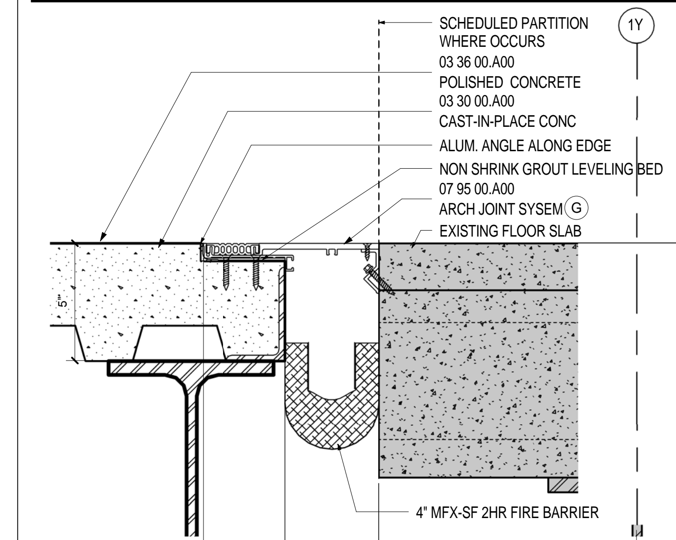
EXPANSION JT @ LEVEL 3 FLOOR SCALE: 3" = 1'-0" A02.03.02 6
