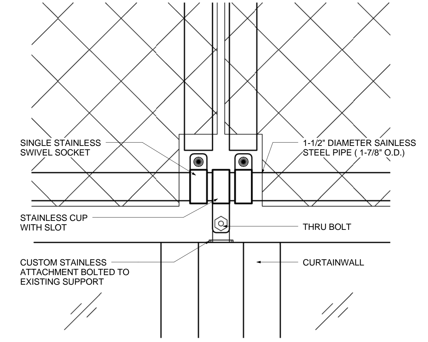
7 DETAIL @ CURTAINWALL ATTACHMENT SCALE: 3" = 1'-0" A11.25 6
