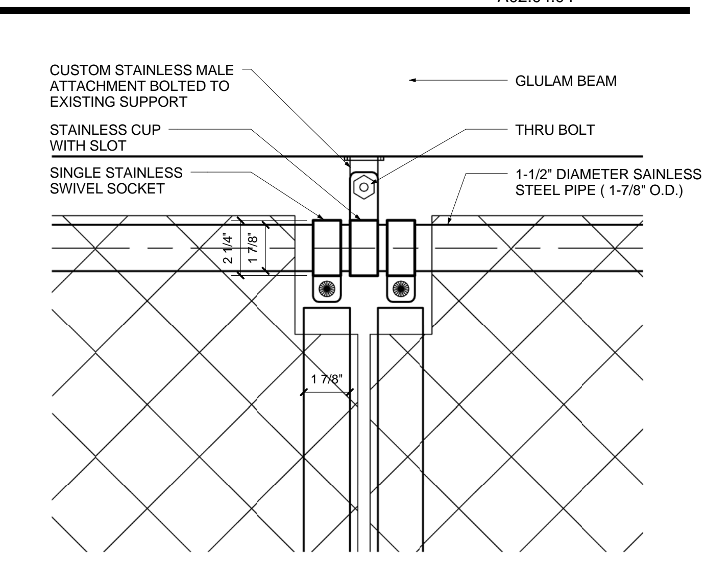
5 DETAIL @ GLU-LAM ATTACHMENT SCALE: 3" = 1'-0" A11.25 4
