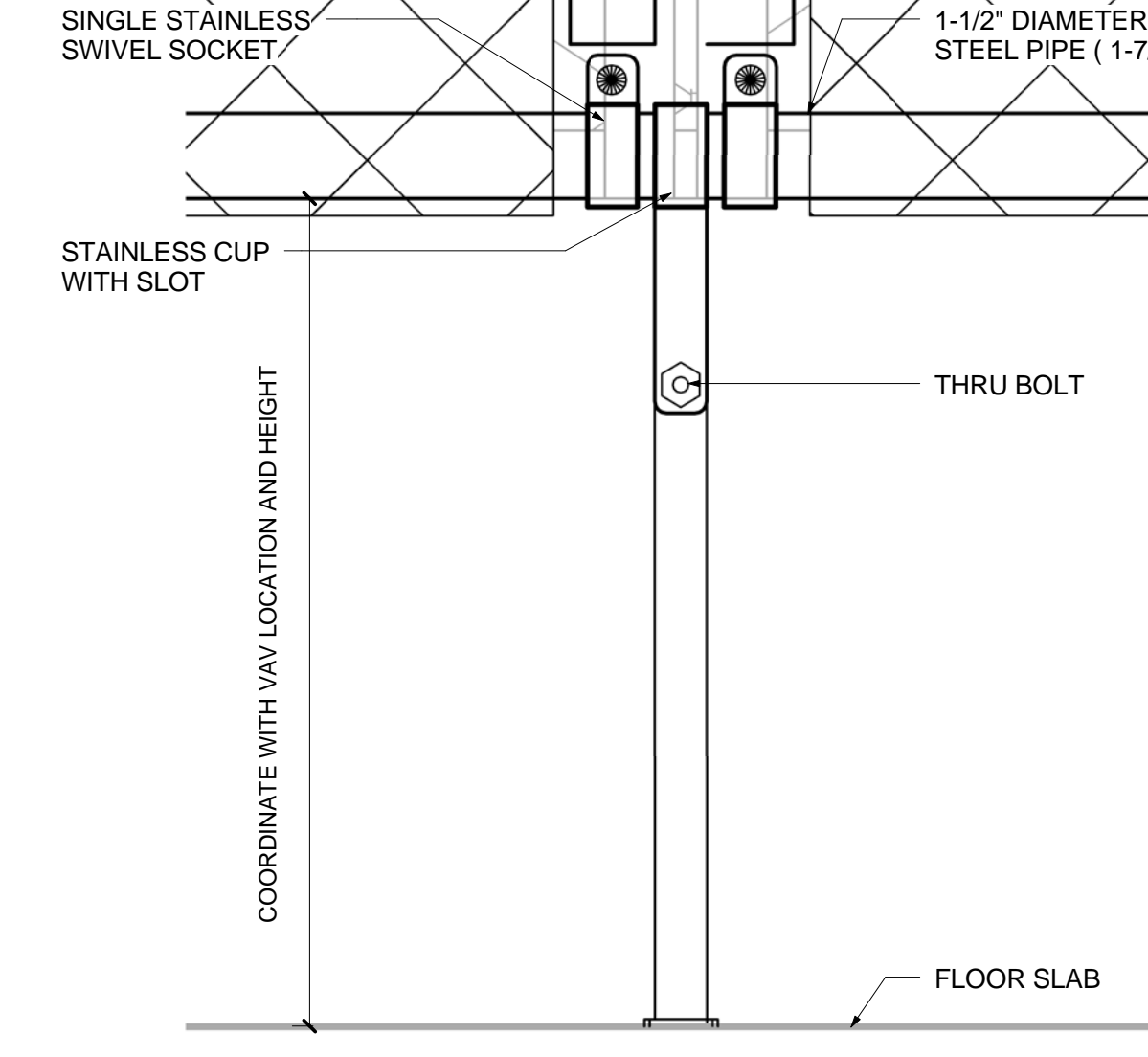
DETAIL @ SLAB ATTACHMENT SCALE: 3" = 1'-0" A11.25
