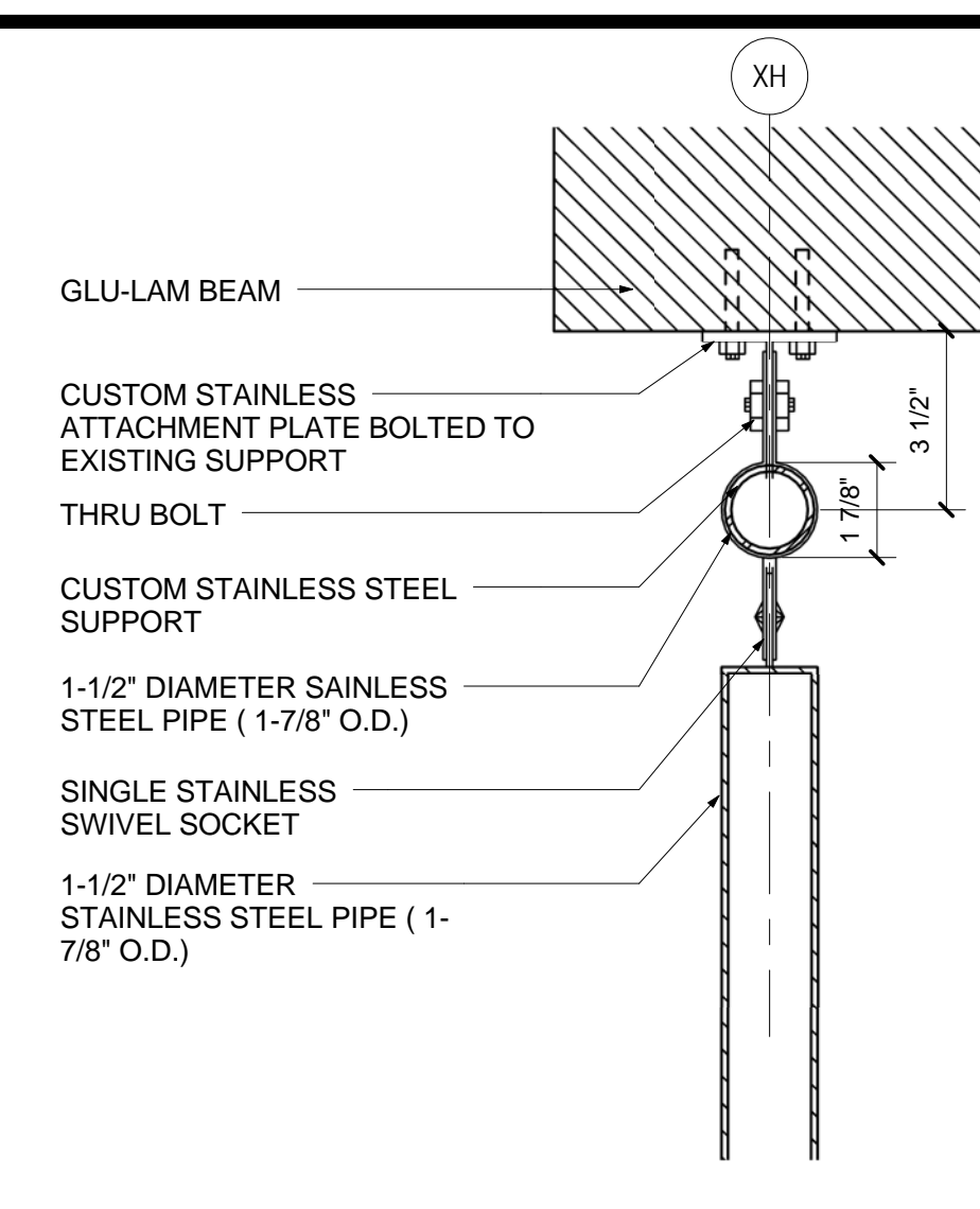
SECTION @ GLU-LAM SCALE: 3" = 1'-0" A11.10
