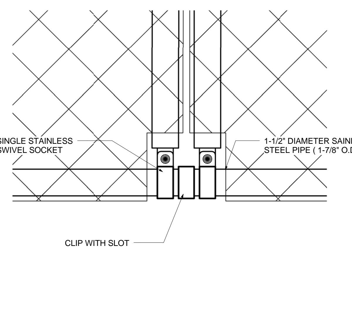
DETAIL @ FENCE ATTACHMENT SCALE: 3" = 1'-0" A11.25 9
