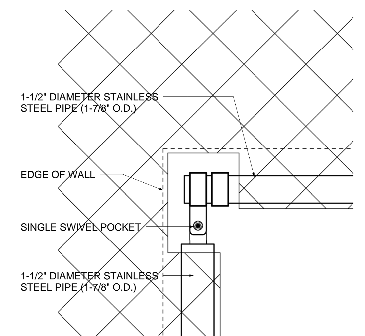
DETAIL @ CORNER ATTACHMENT SCALE: 3" = 1'-0" A11.25 8
