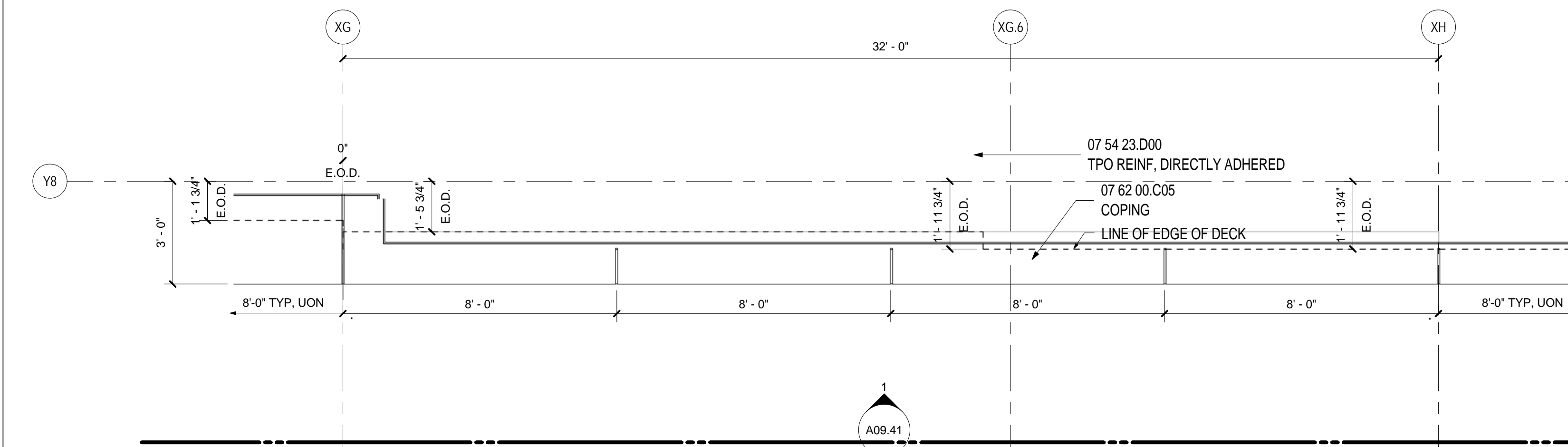
WALL TYPE C.1 - ROOF
