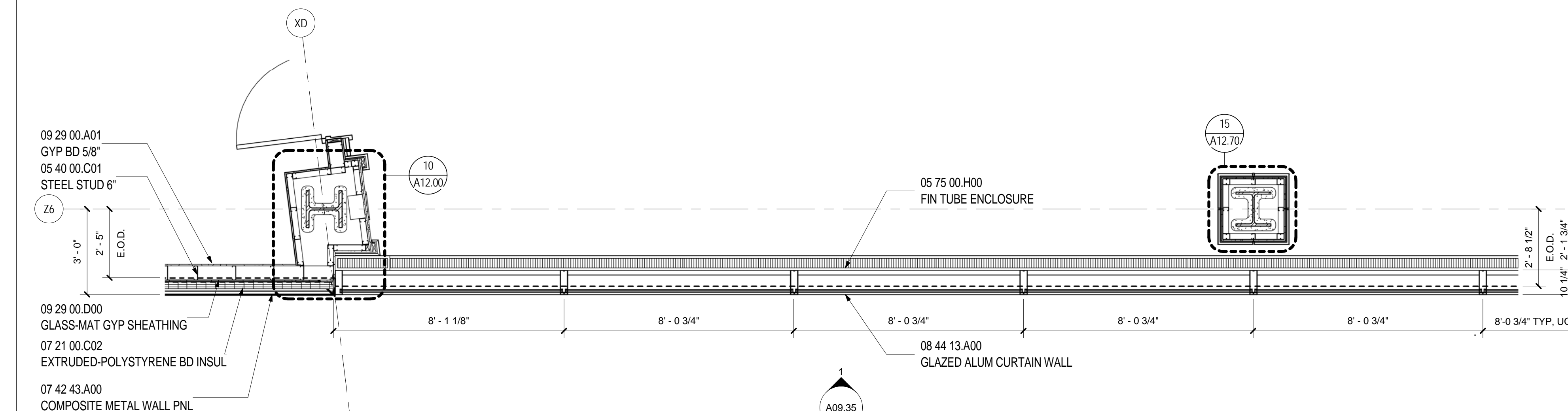
WALL TYPE B.6 - PLAN LEVEL 4
