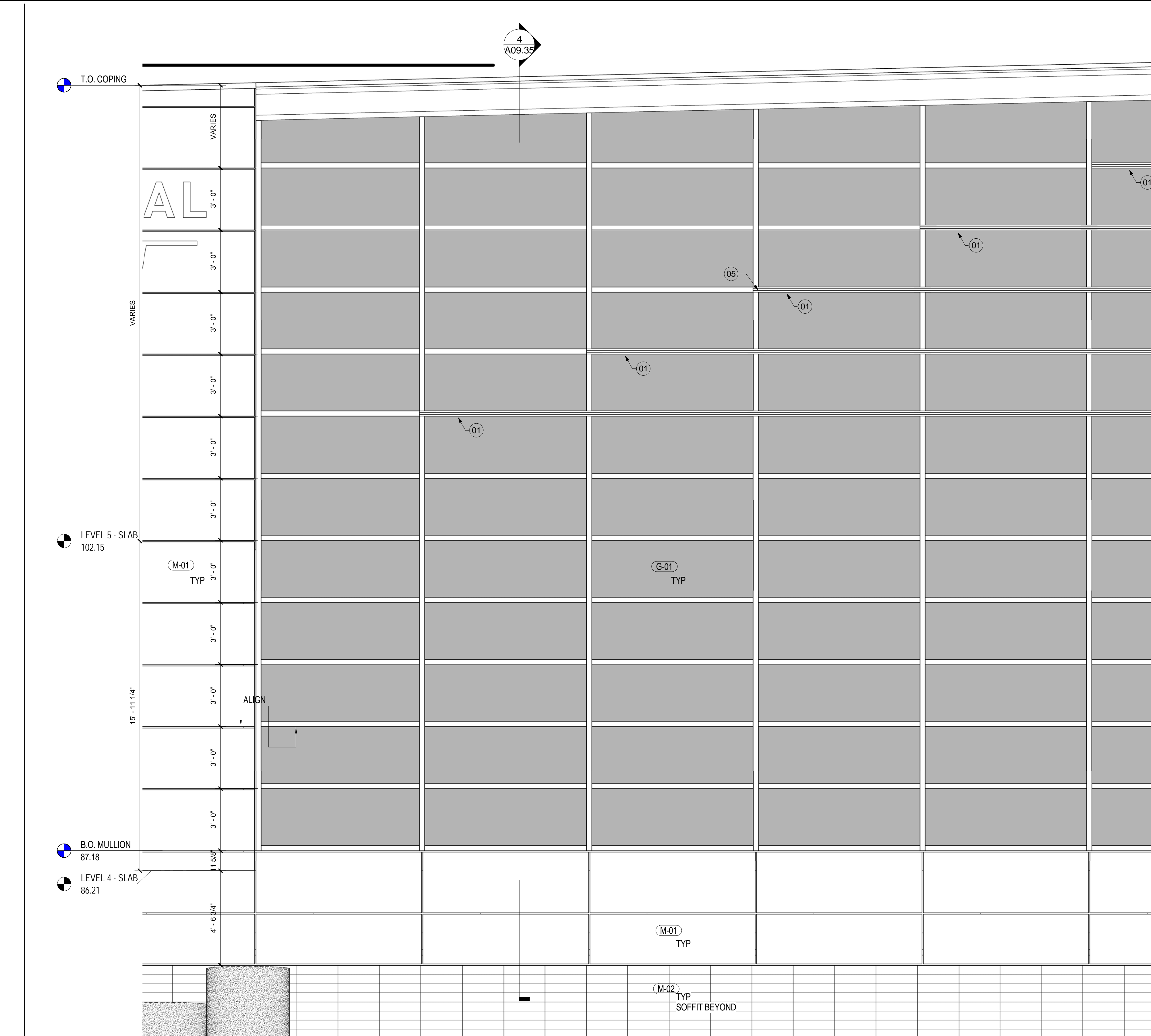
WALL TYPE B.6 - ELEVATION
