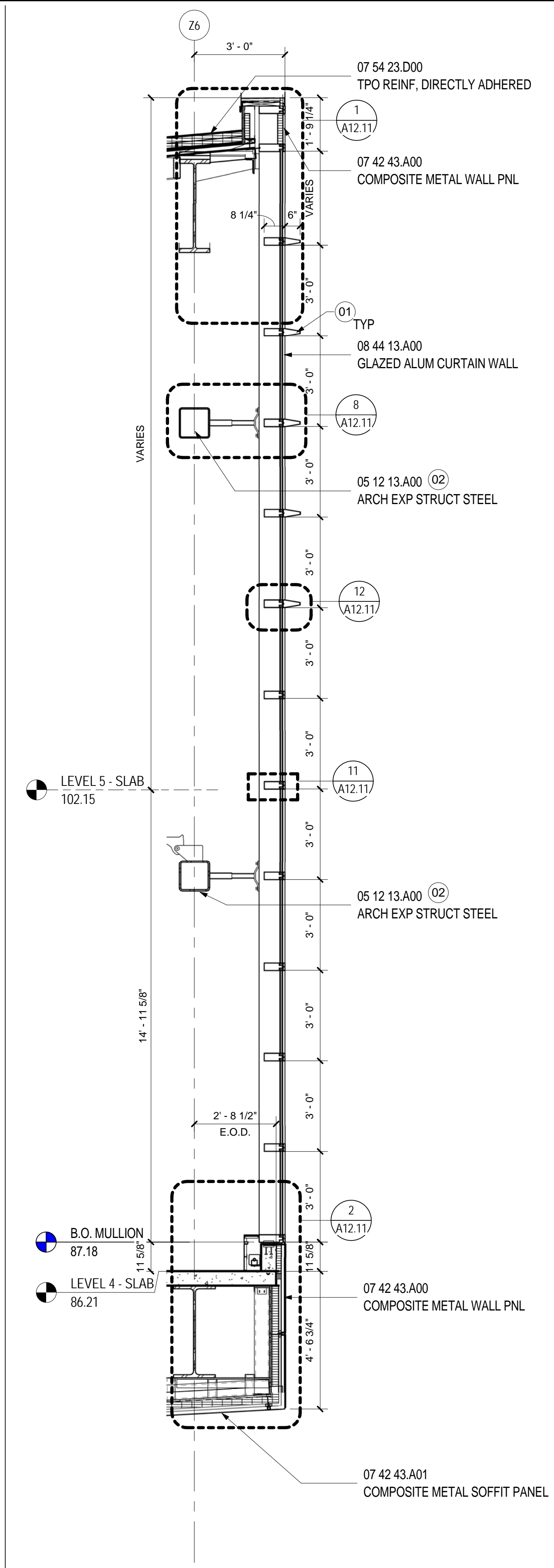
WALL TYPE B.6 - SECTION
