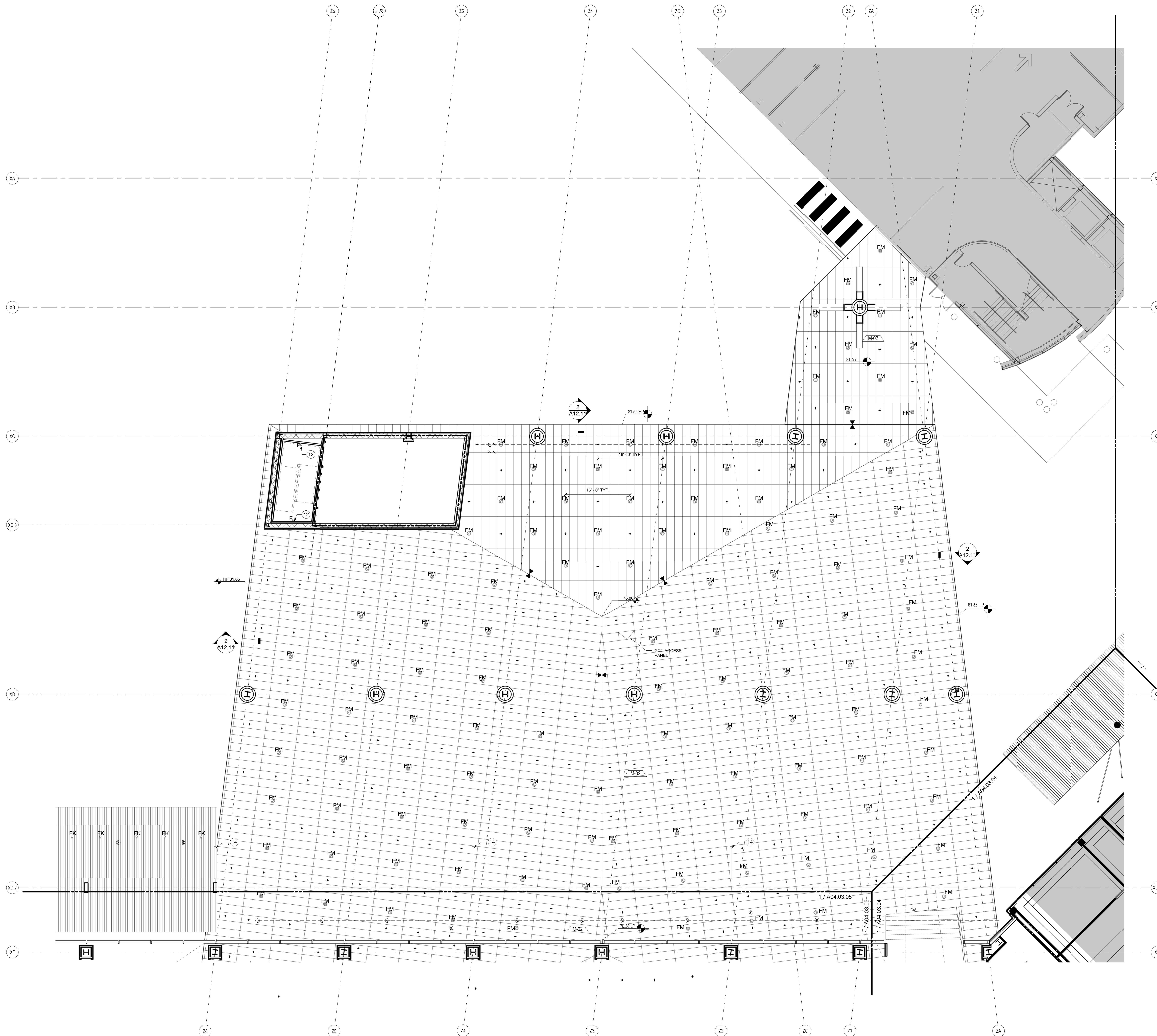
REFLECTED CEILING PLAN - LEVEL 3 - ZONE 6 SCALE: 1/8" = 1'-0"
