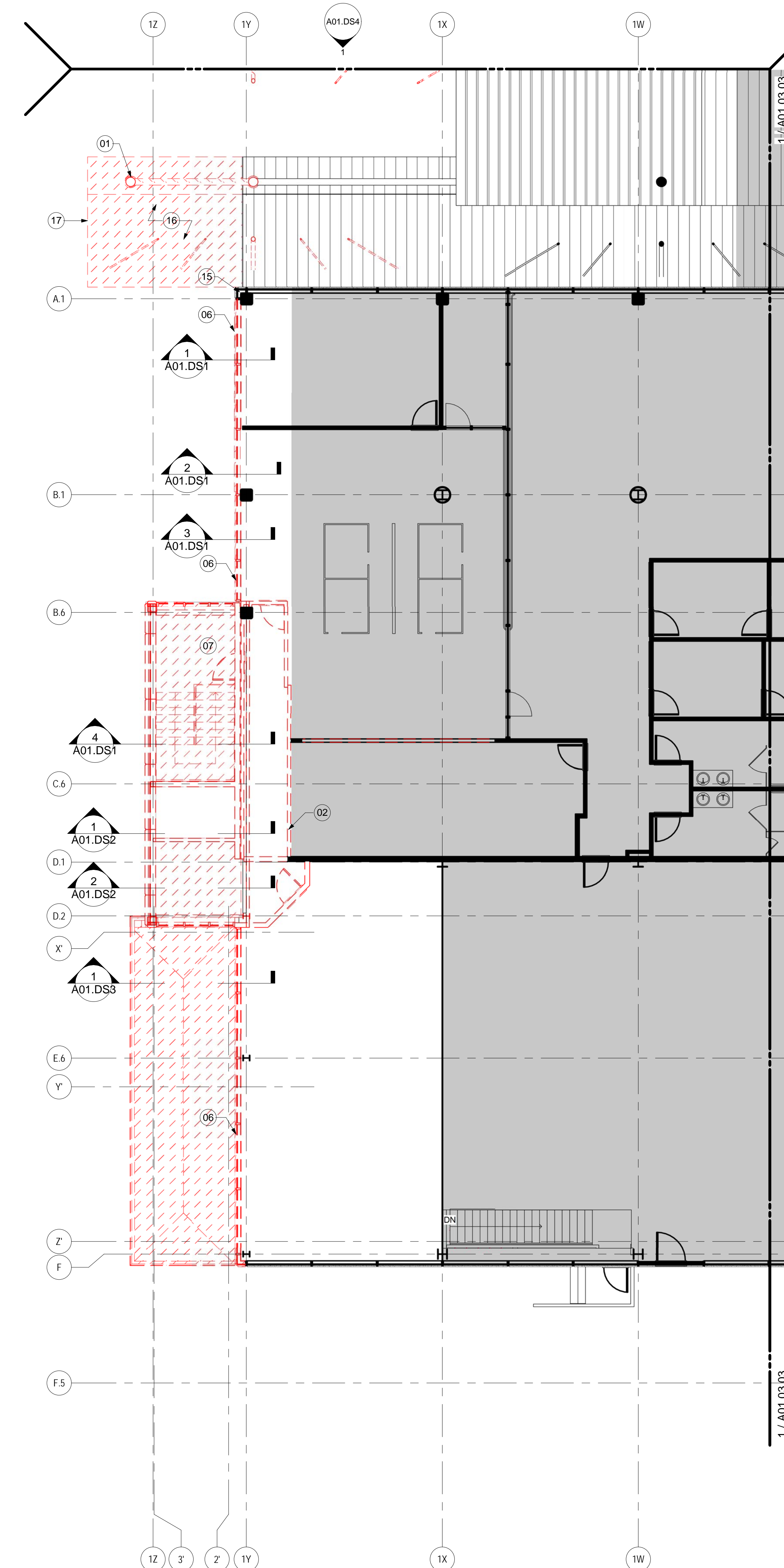
DEMOLITION PLAN - LEVEL 3 - ZONE 4 SCALE: 1/8" = 1'-0" A01.DS1 1
