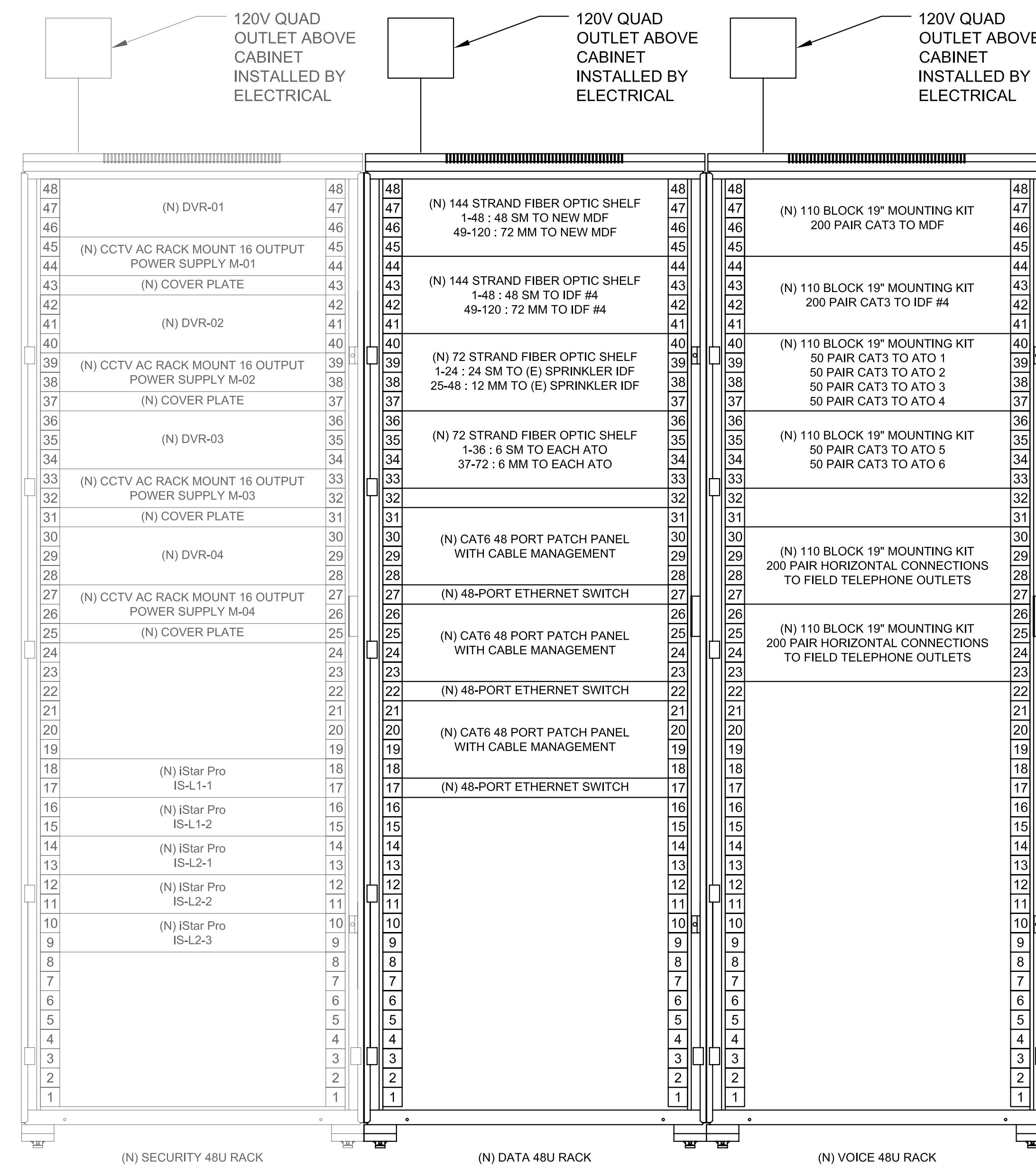
3 TELECOMMUNICATIONS VOICE, DATA AND SECURITY AND SURVEILLANCE RACK RACK TC12.03 NTS
