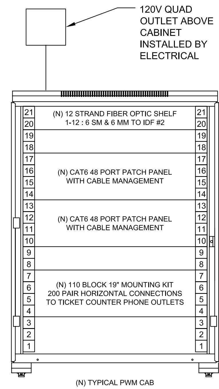
2 PWM TELECOMMUNICATIONS VOICE/DATA MINI-CABINET TC12.03 NTS
