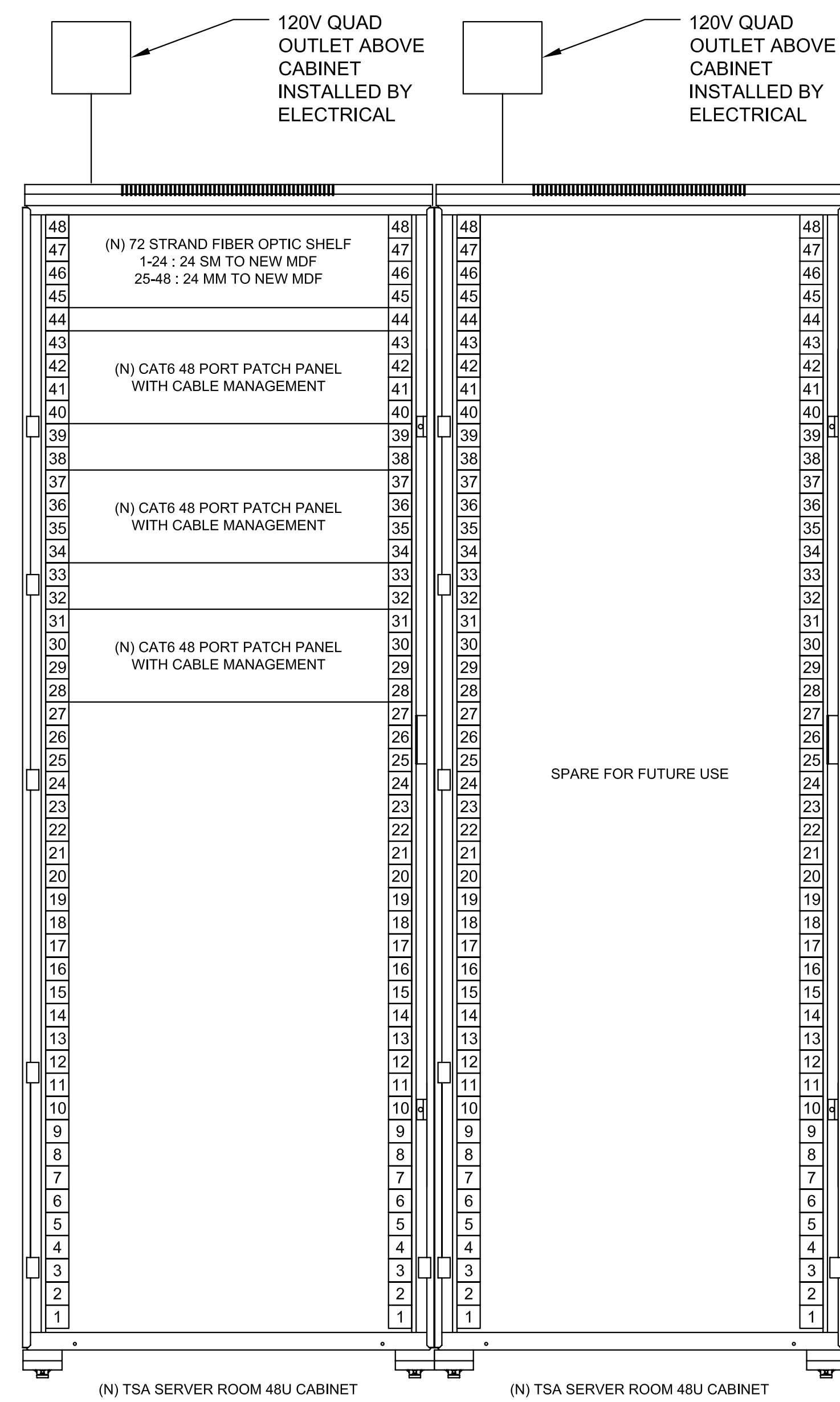
1 TSATELECOMMUNICATIONS CABINETS TC12.03 NTS
