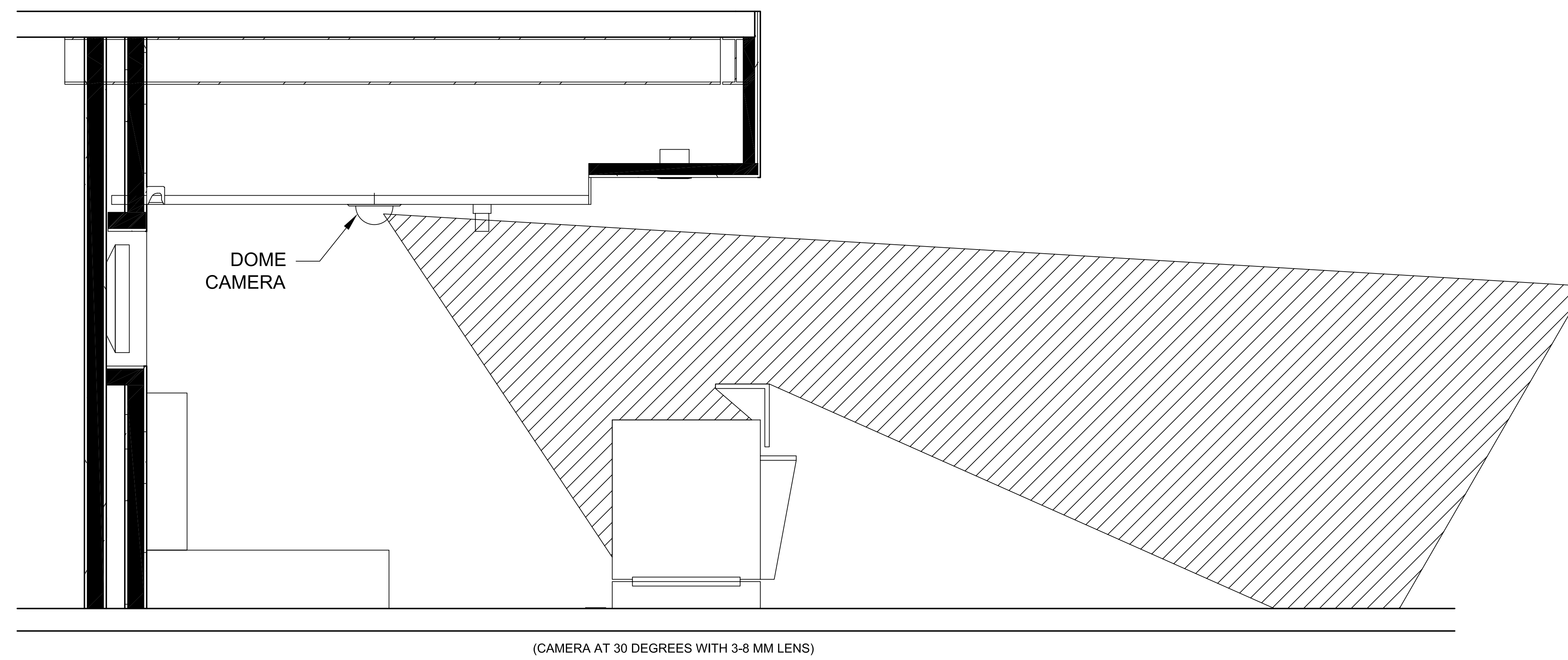
1 CCTV PLACEMENT AT TICKETING COUNTERS SS12.25 SCALE: 3/4" = 1'
