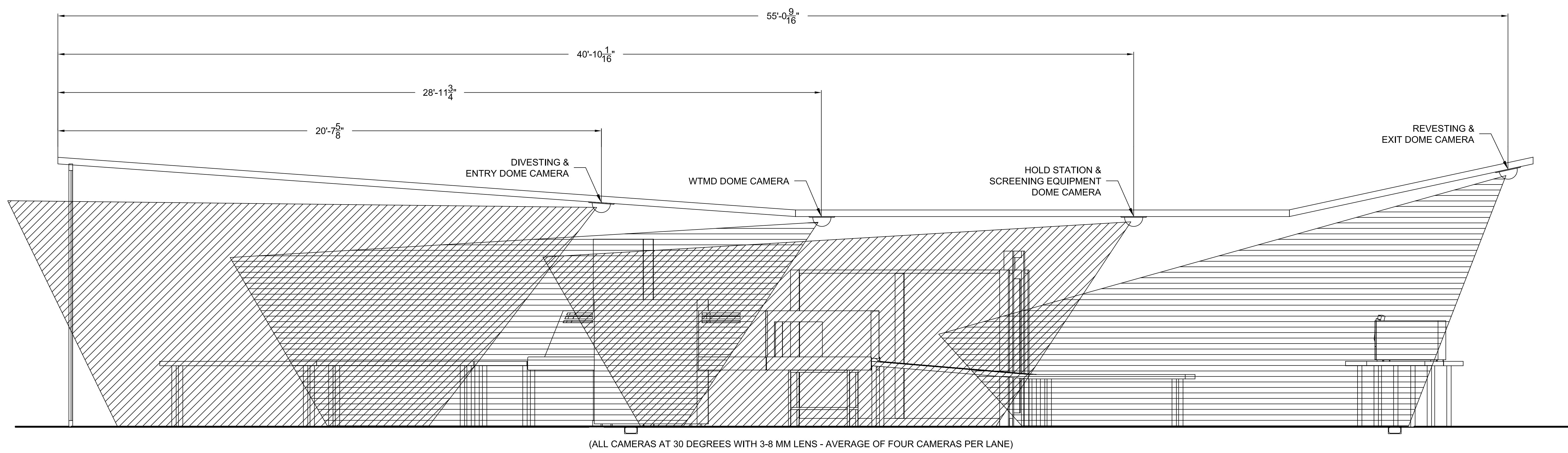
2 CCTV PLACEMENT AT SECURITY CHECKPOINT SS12.25 SCALE: 1/2" = 1'
