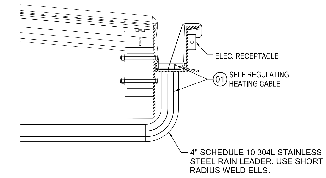
HEAT TRACE DETAIL @ GUTTER SCALE: NOT TO SCALE
