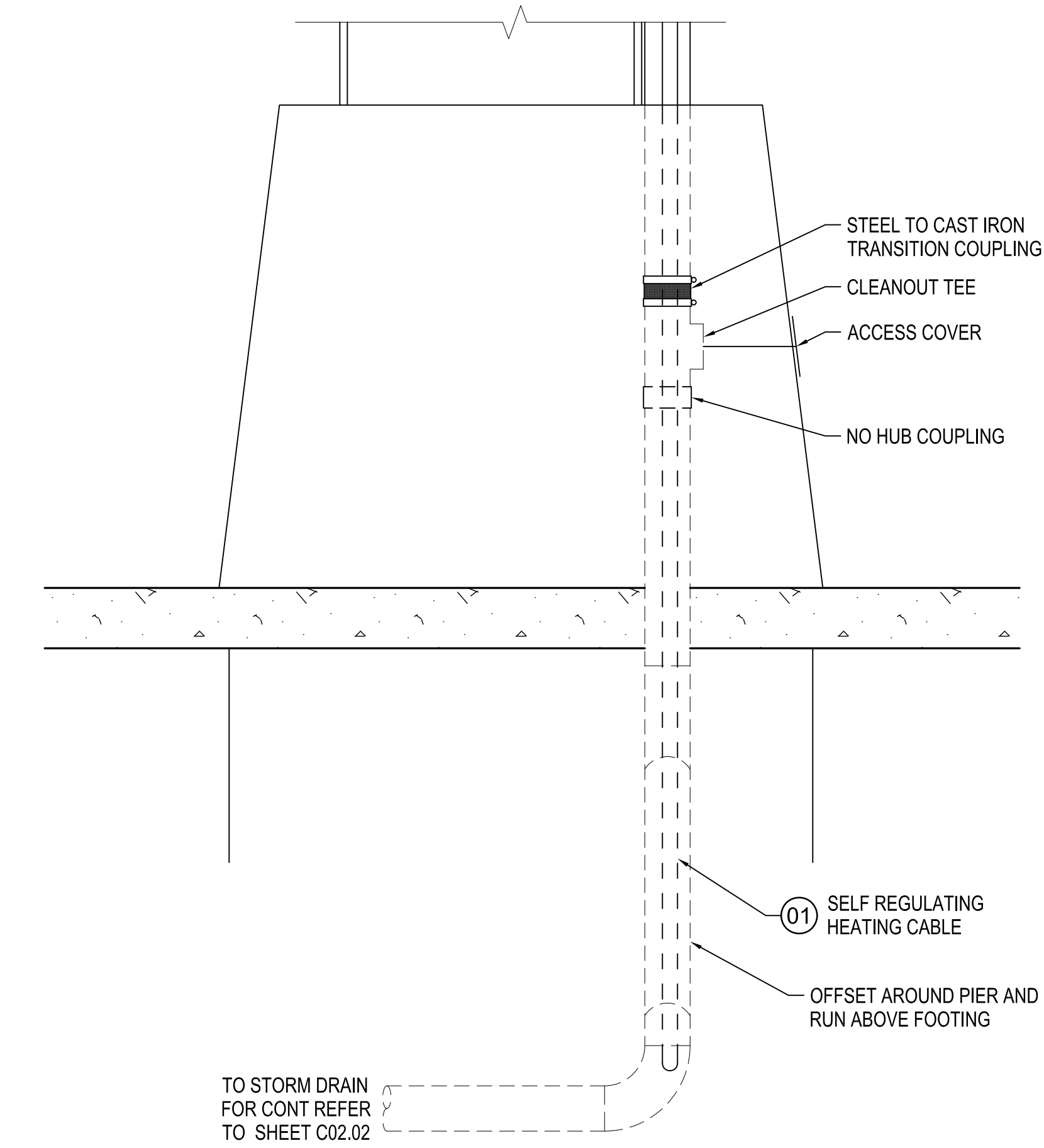
HEAT TRACE DETAIL @ BASE SCALE: NOT TO SCALE
