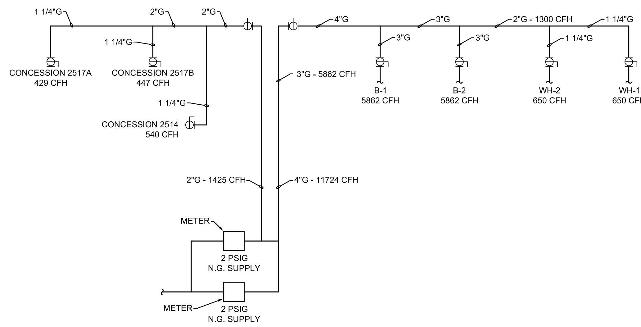
GAS RISER DIAGRAM SCALE: NOT TO SCALE
