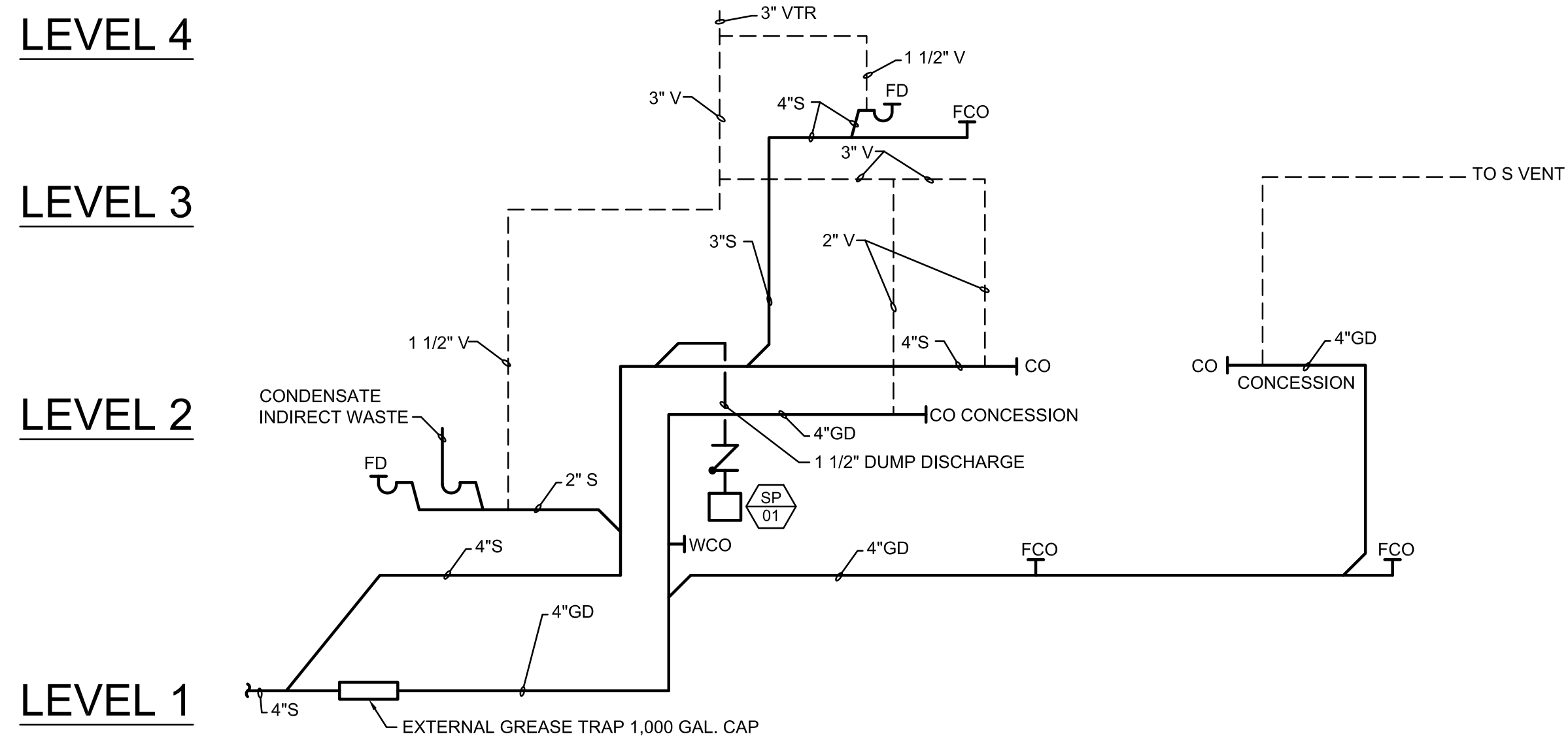
WEST SANITARY & GREASE DRAIN SCALE: NOT TO SCALE
