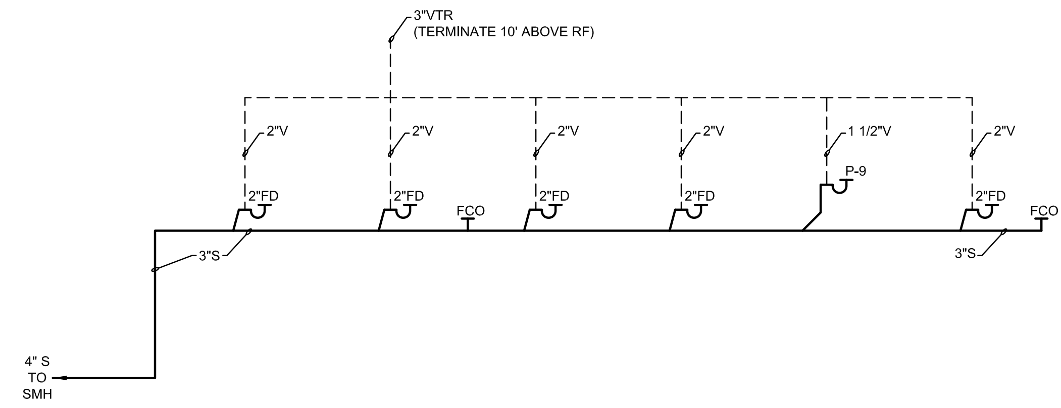
MECHANICAL ROOM SANITARY RISER DIAGRAM SCALE: NOT TO SCALE
