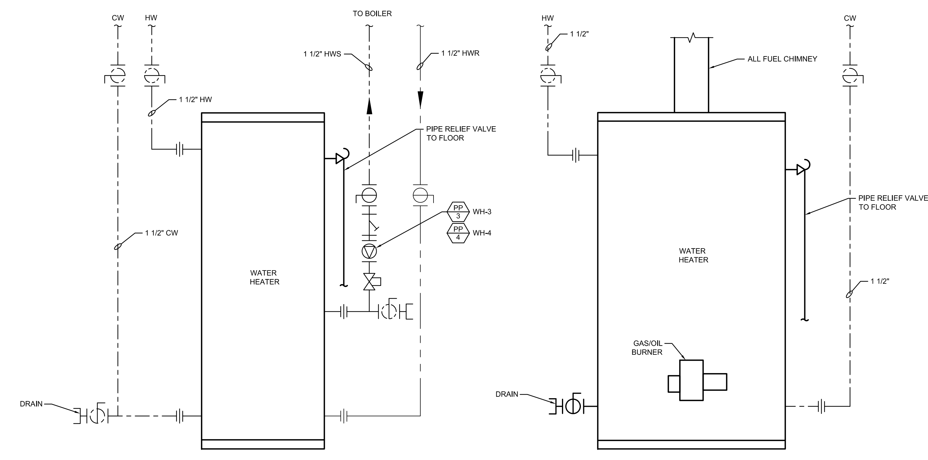
WH-3 & 4 SCHEMATIC PIPING 3 WH-1 & 2 SCHEMATIC PIPING 2 SCALE: NOT TO SCALE SCALE: NOT TO SCALE
