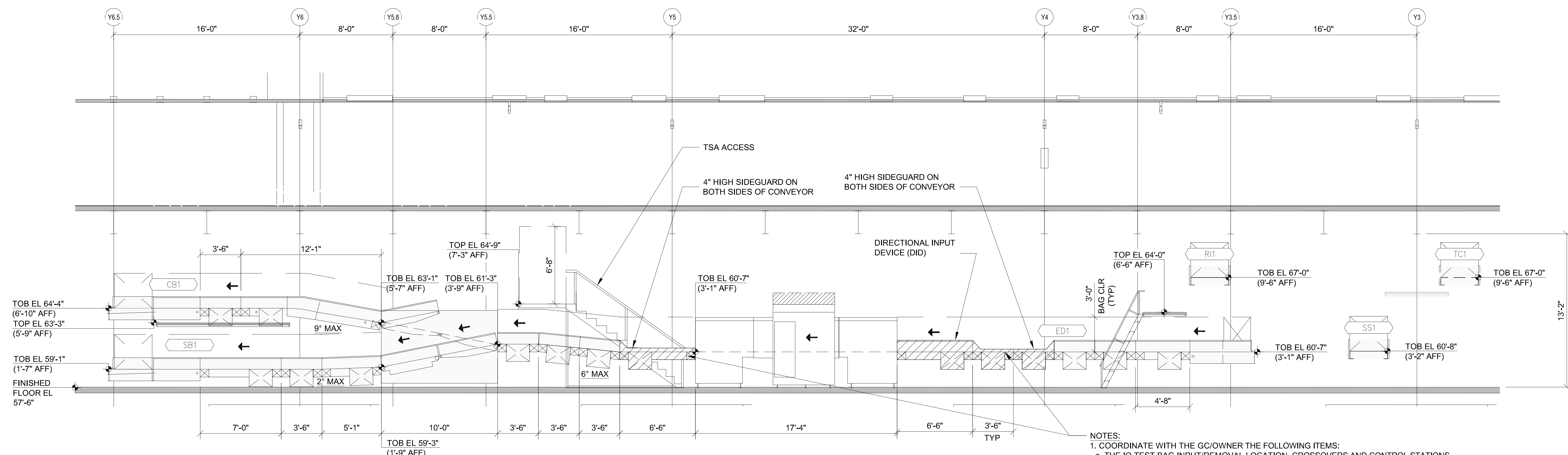
L SECTION - ED1 CONVEYORS B09.03 1/4" = 1'-0"
