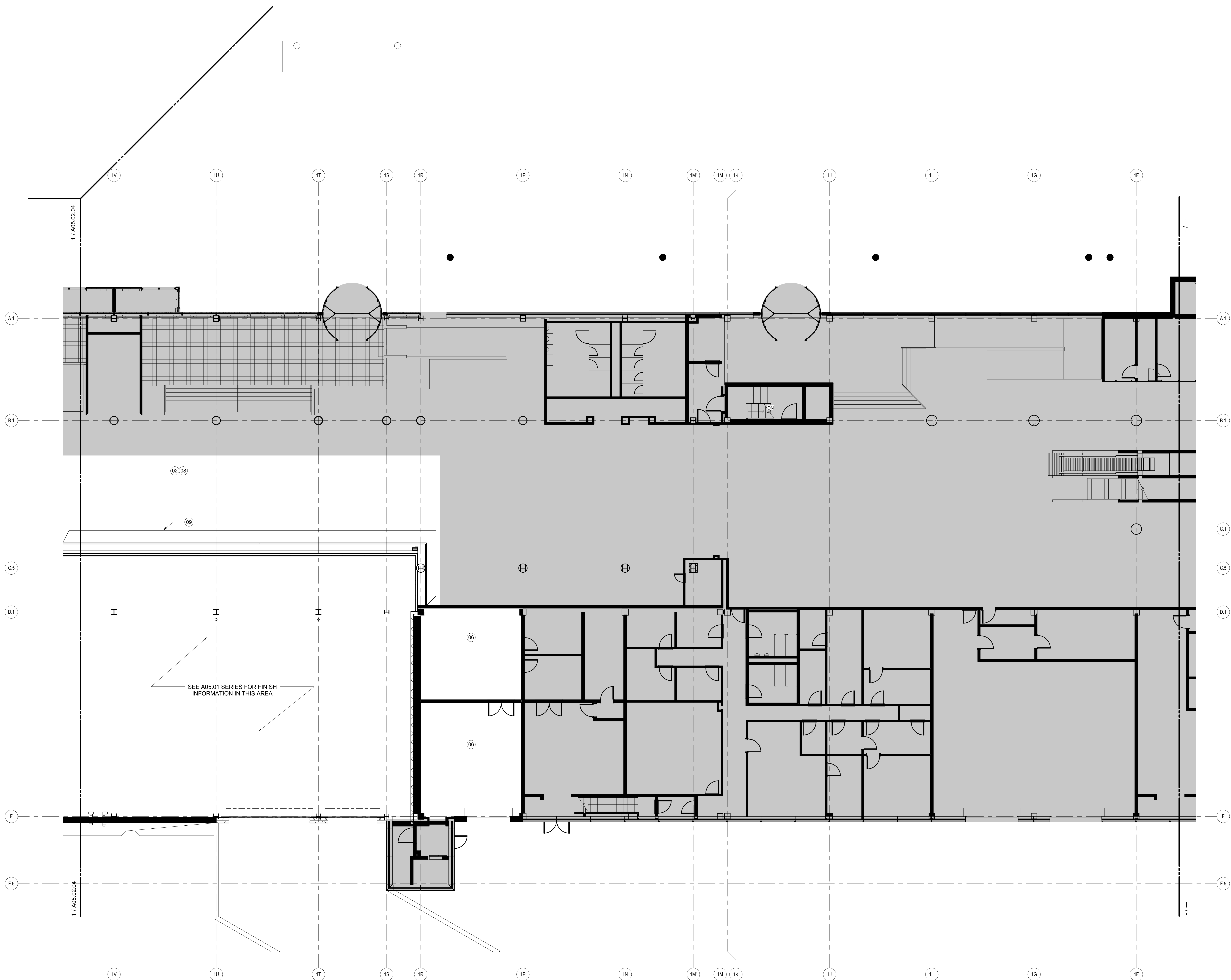
FINISH PLAN - LEVEL 2 - ZONE 3 SCALE: 1/8" = 1'-0"
