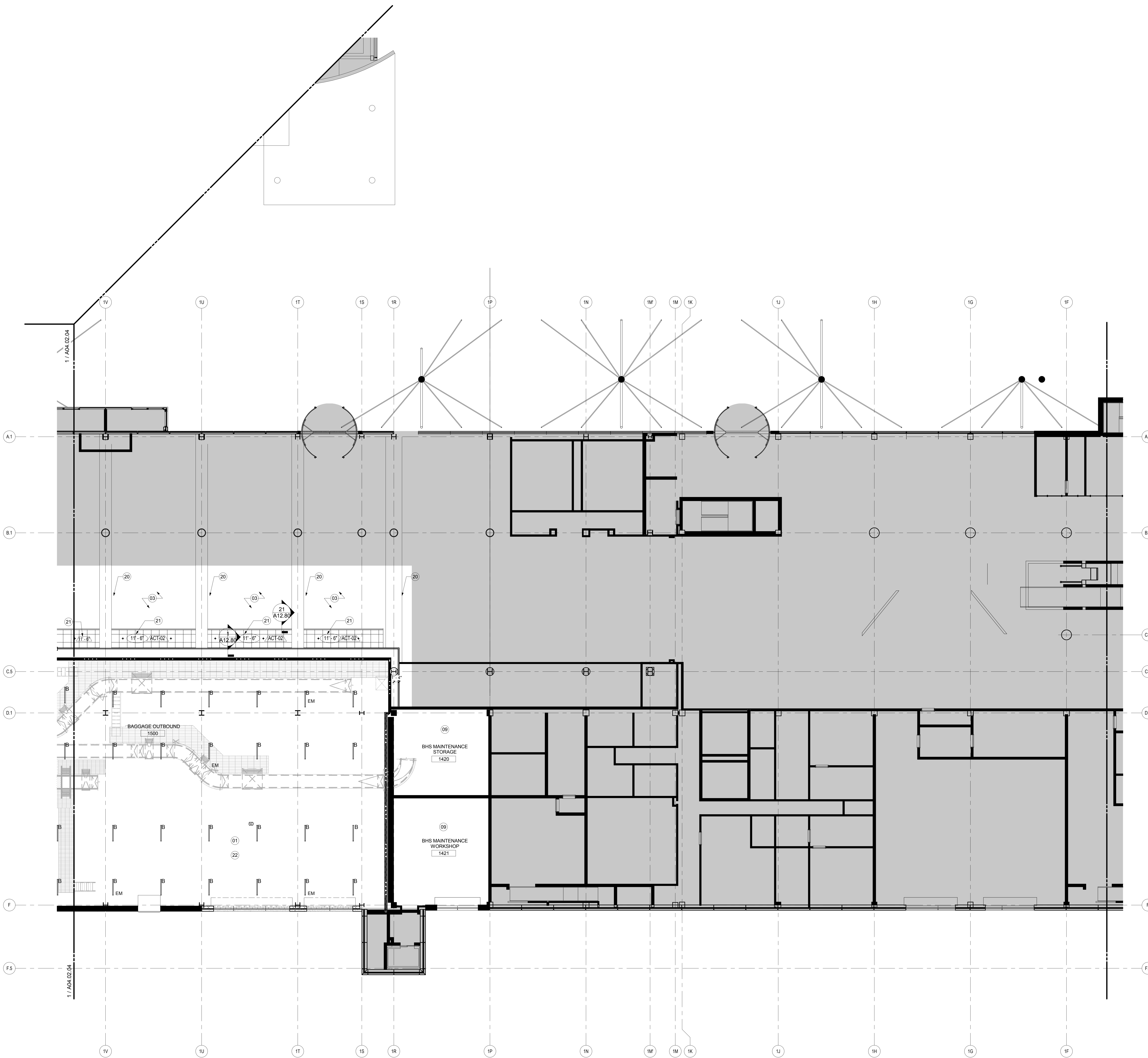
REFLECTED CEILING PLAN - LEVEL 2 - ZONE 3
