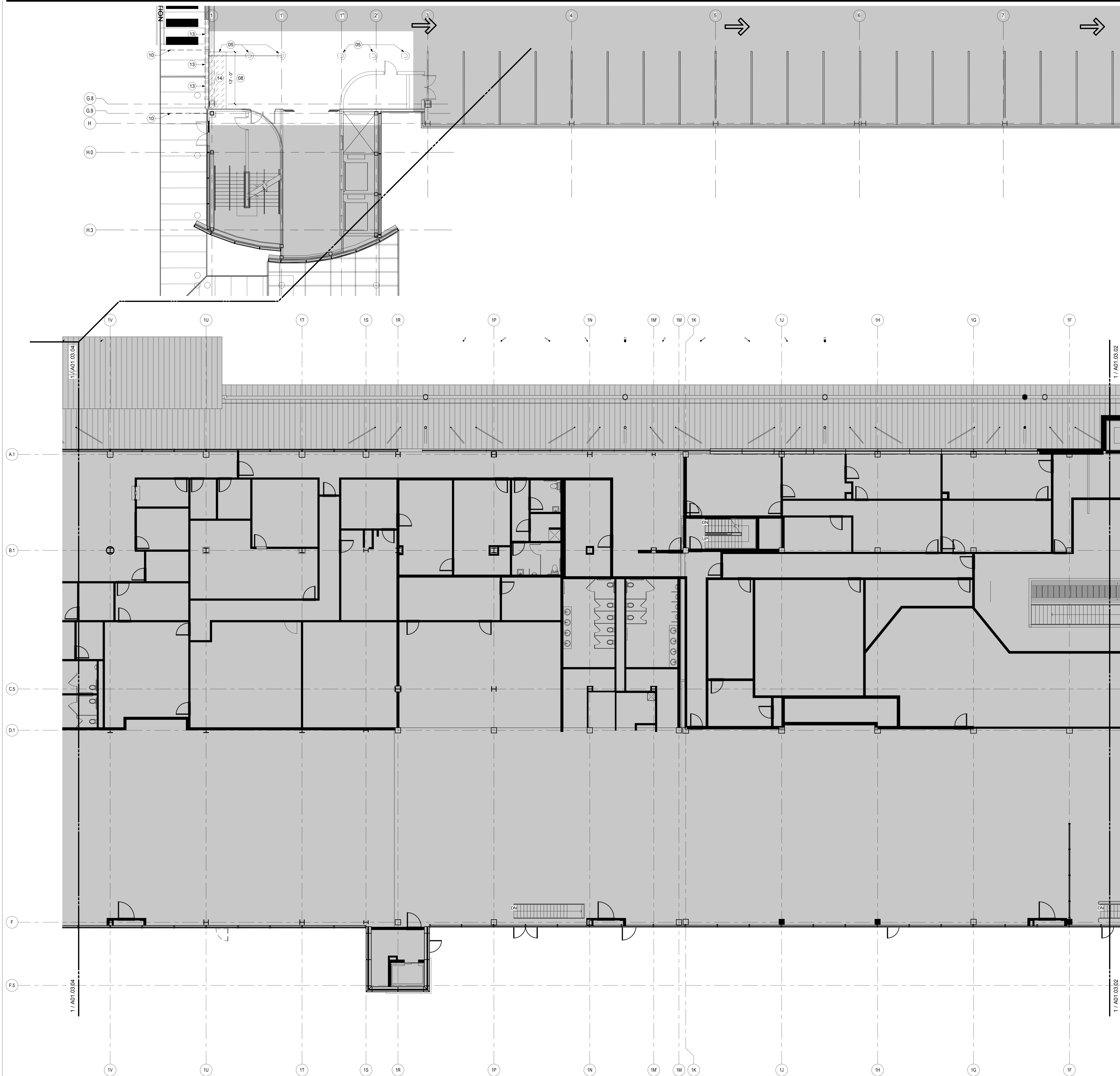
DEMOLITION PLAN - LEVEL 3 - ZONE 3 SCALE: 1/8" = 1'-0"
