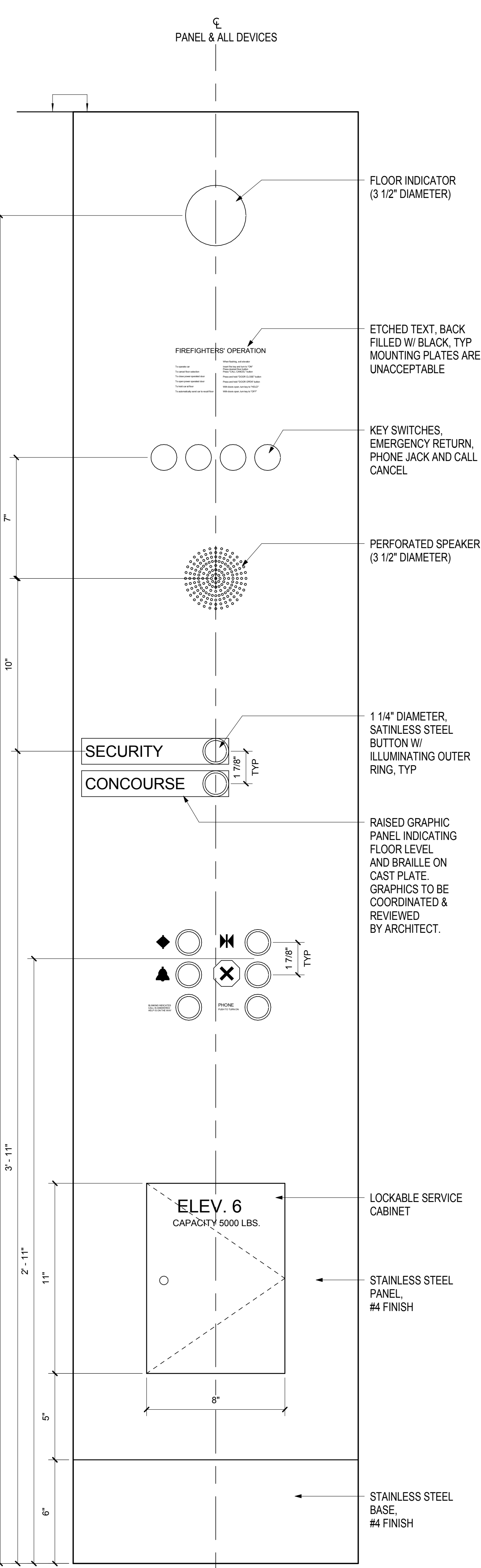
PANEL DETAIL - ELEVATORS 6 & 7 SCALE: 3" = 1'-0" A10.31
