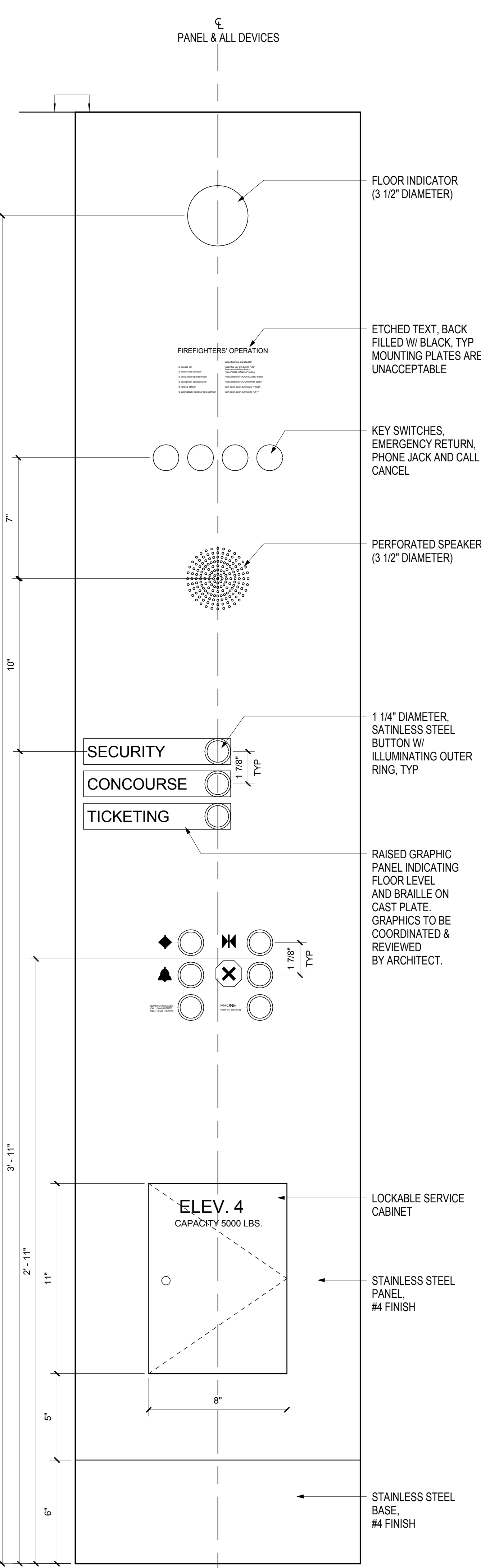
PANEL DETAIL - ELEVATORS 4 & 5 SCALE: 3" = 1'-0" A10.30
