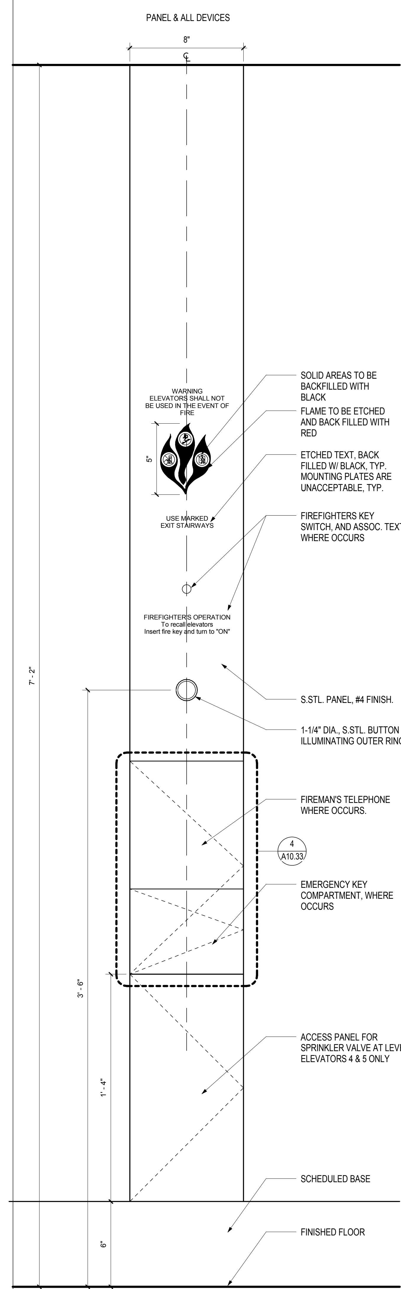
CALL PANEL TYP @ ELEV 4, 5, 6 & 7 SCALE: 3" = 1'-0" A10.03
