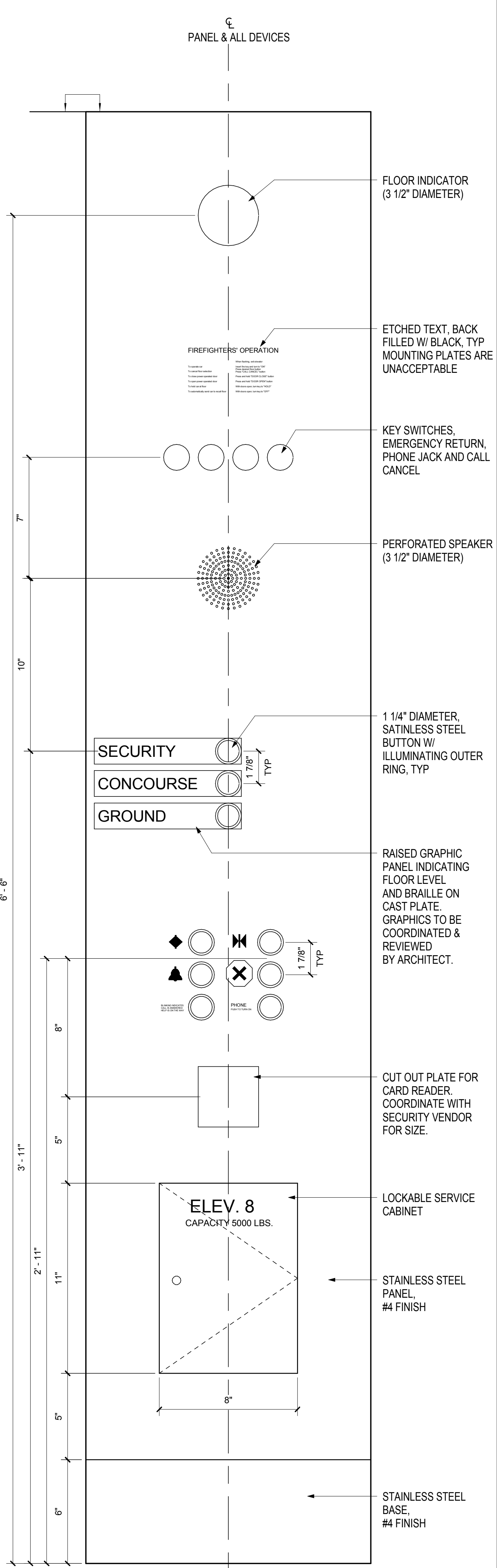
PANEL DETAIL - ELEVATOR 8 SCALE: 3" = 1'-0" A10.32
