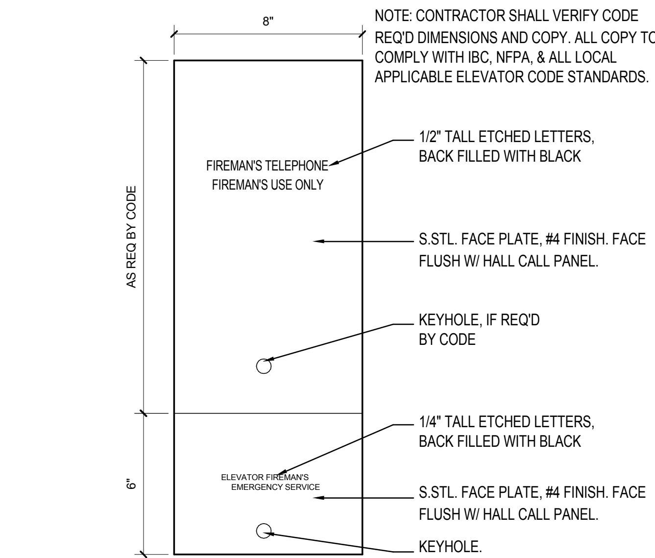
FIREMANS TELEPHONE & KEY BOX SCALE: 3" = 1'-0" A10.33
