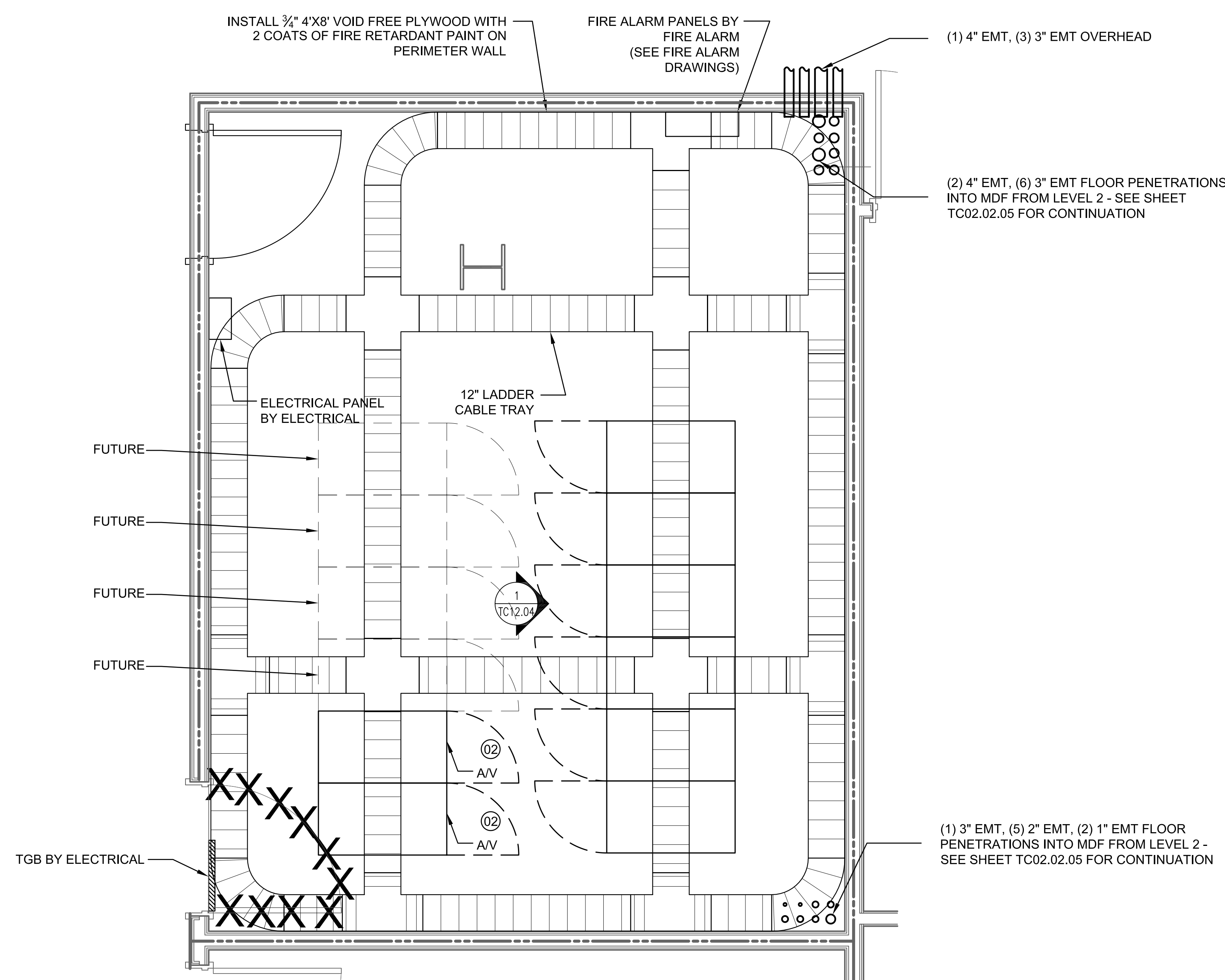
2 TELECOMMUNICATIONS MDF ROOM TC12.04 SCALE: 1/2"=1'
