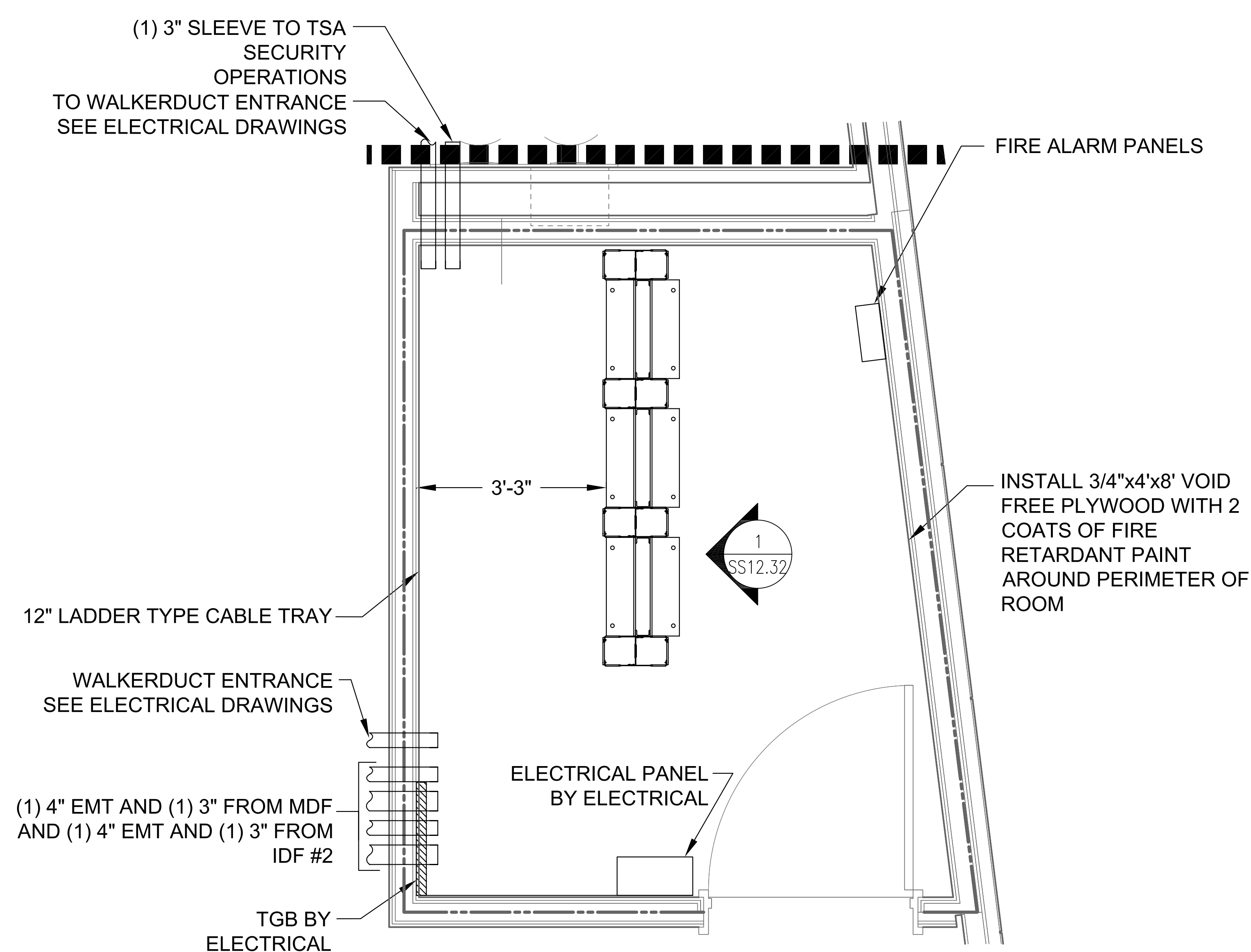
2 TELECOMMUNICATIONS ROOM IDF L4 SS12.32 SCALE: NTS
