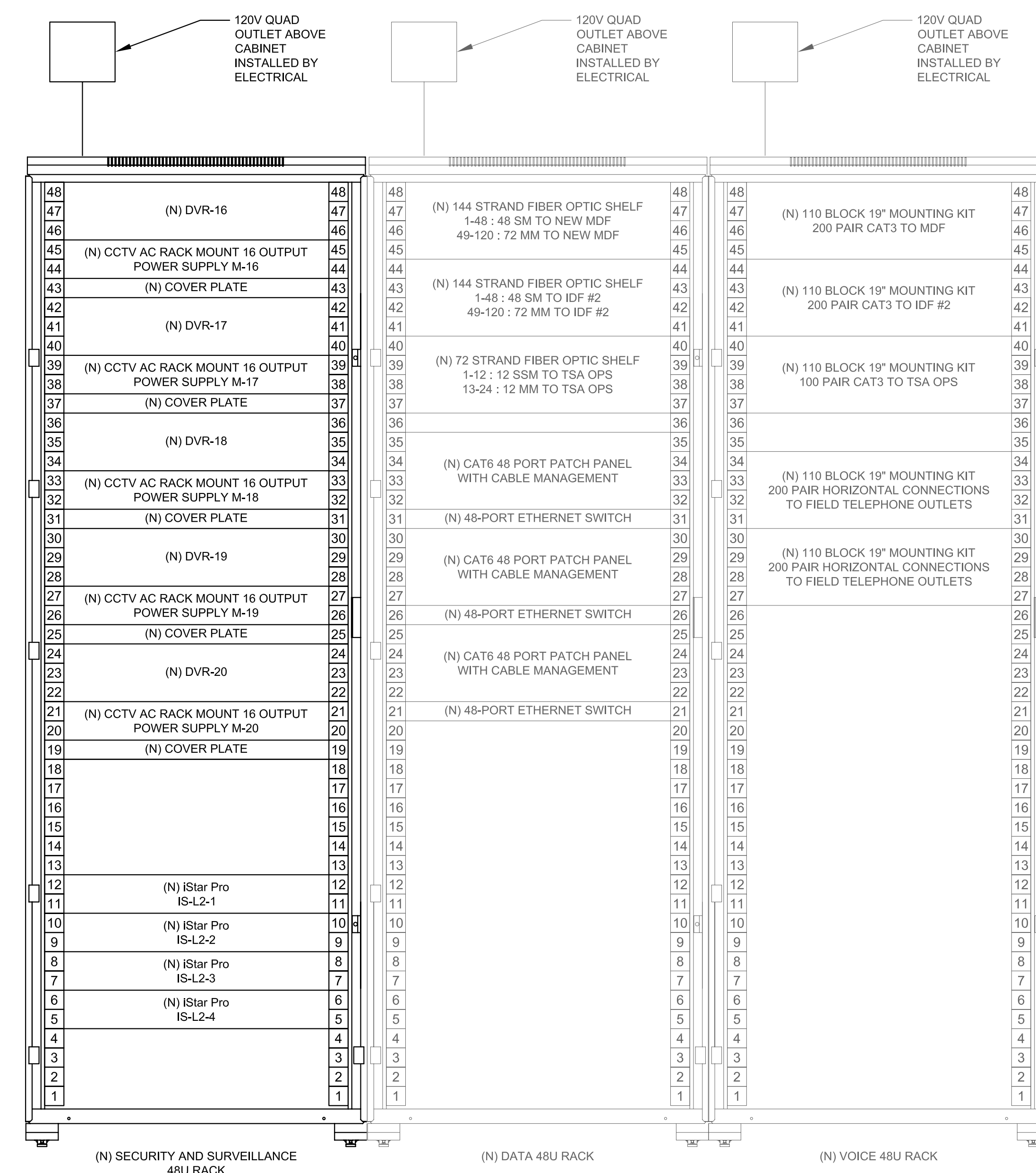
1 VOICE/DATA/SECURITY RACK ELEVATIONS SS12.32 NTS
