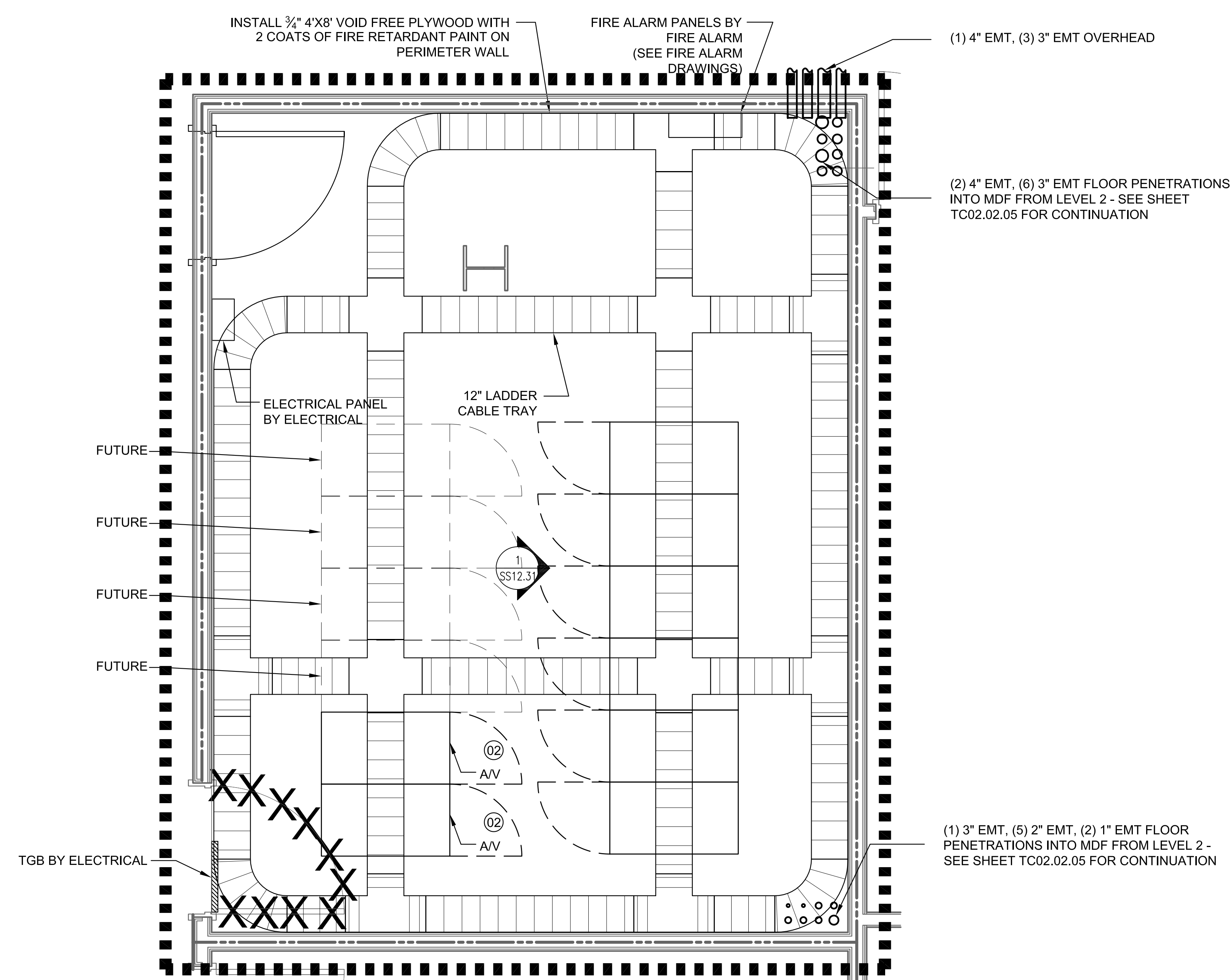
2 TELECOMMUNICATIONS ROOM MDF SS12.31 SCALE: NTS
