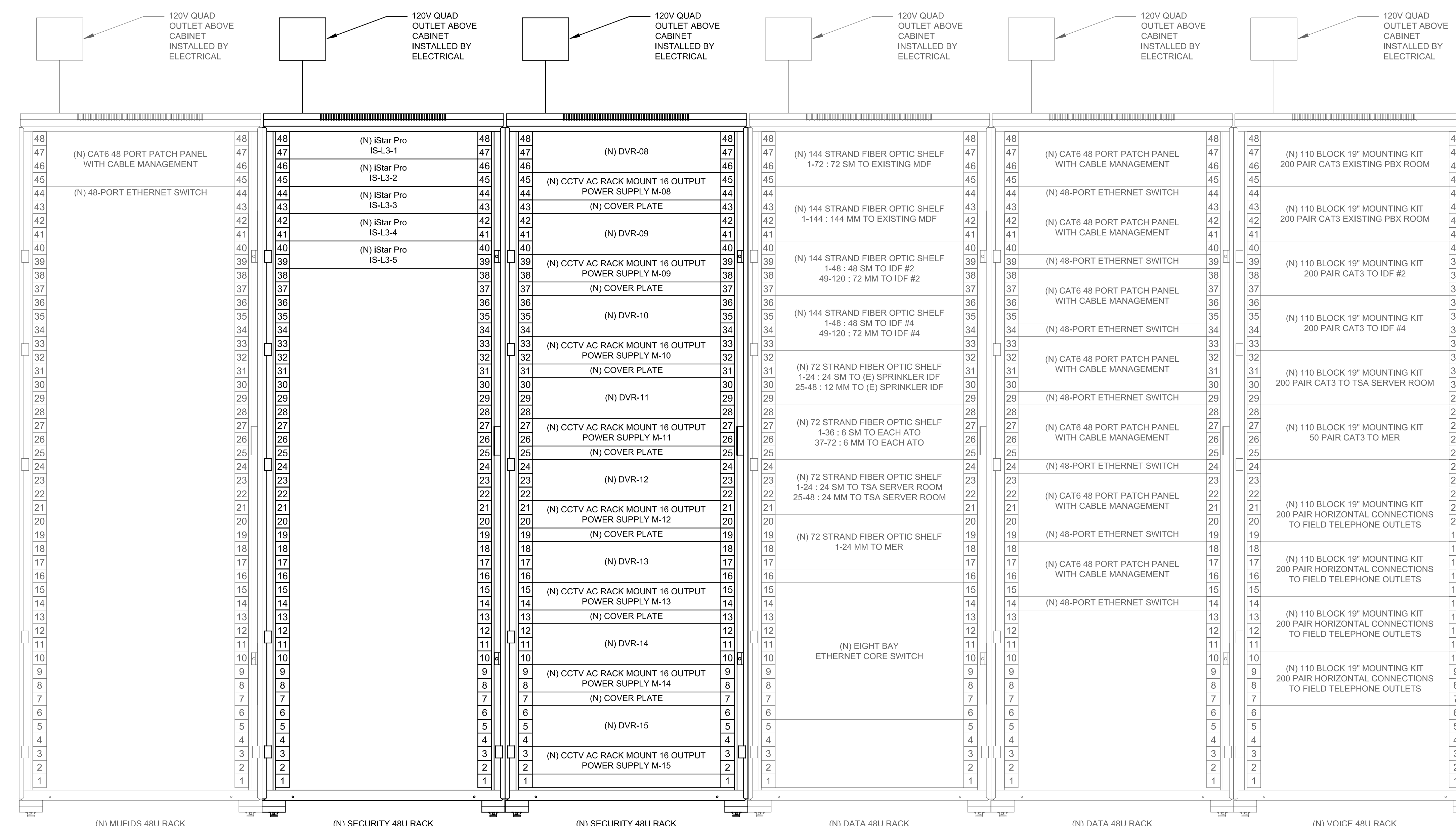
1 VOICE/DATA/SECURITY CABINET ELEVATIONS SS12.31 NTS
