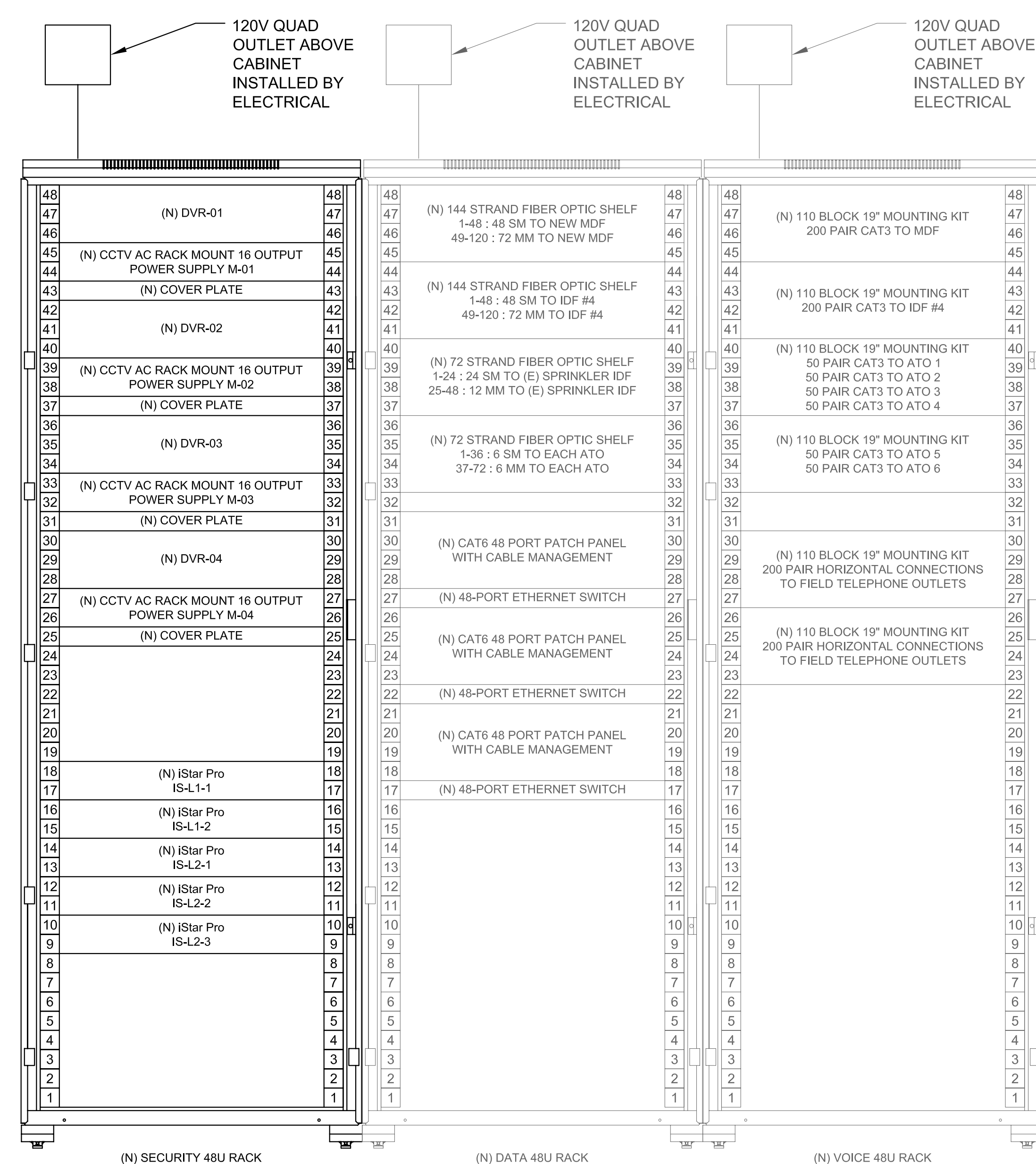
1 VOICE/DATA/SECURITY RACK ELEVATIONS SS12.30 NTS
