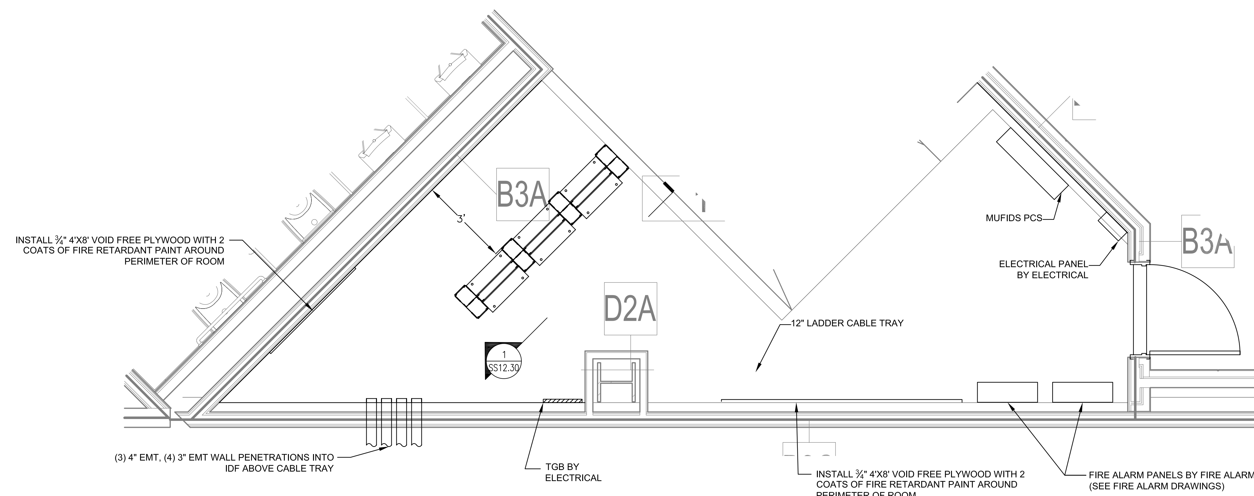
2 TELECOMMUNICATIONS ROOM IDF L2 SS12.30 SCALE: NTS
