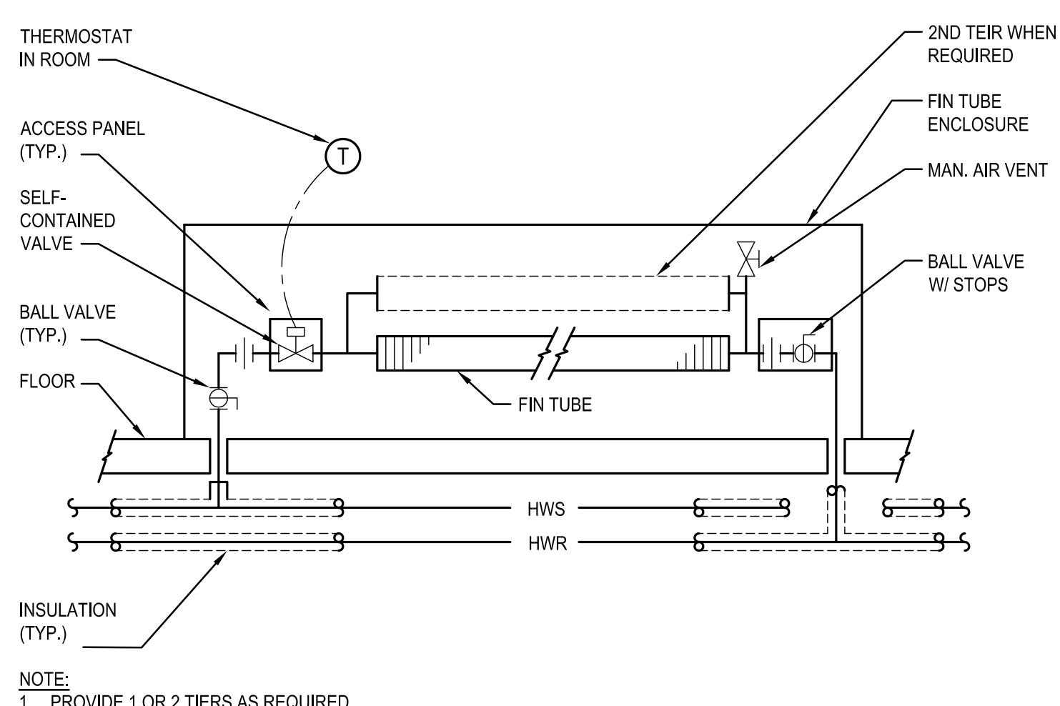
DETAIL - HOT WATER FTR PIPING 6 SCALE: NOT TO SCALE
