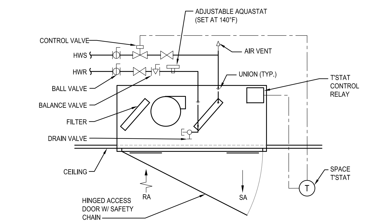
DETAIL - CEILING RECESSED CABINET UNIT HEATER 7 SCALE: NOT TO SCALE
