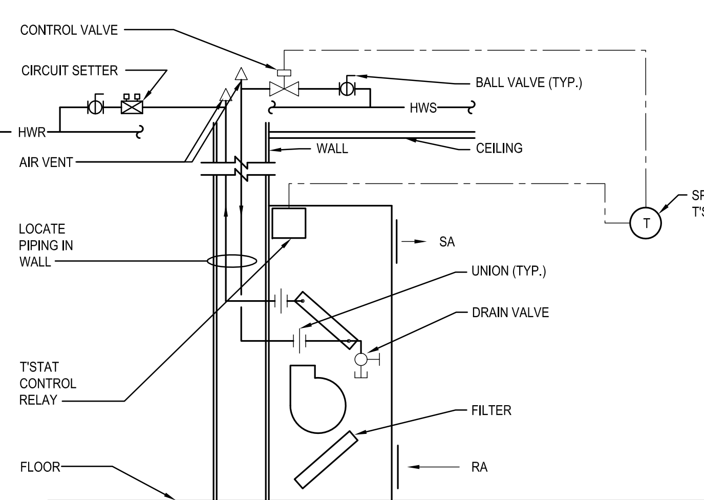
DETAIL - WALL CABINET UNIT HEATER 11 SCALE: NOT TO SCALE
