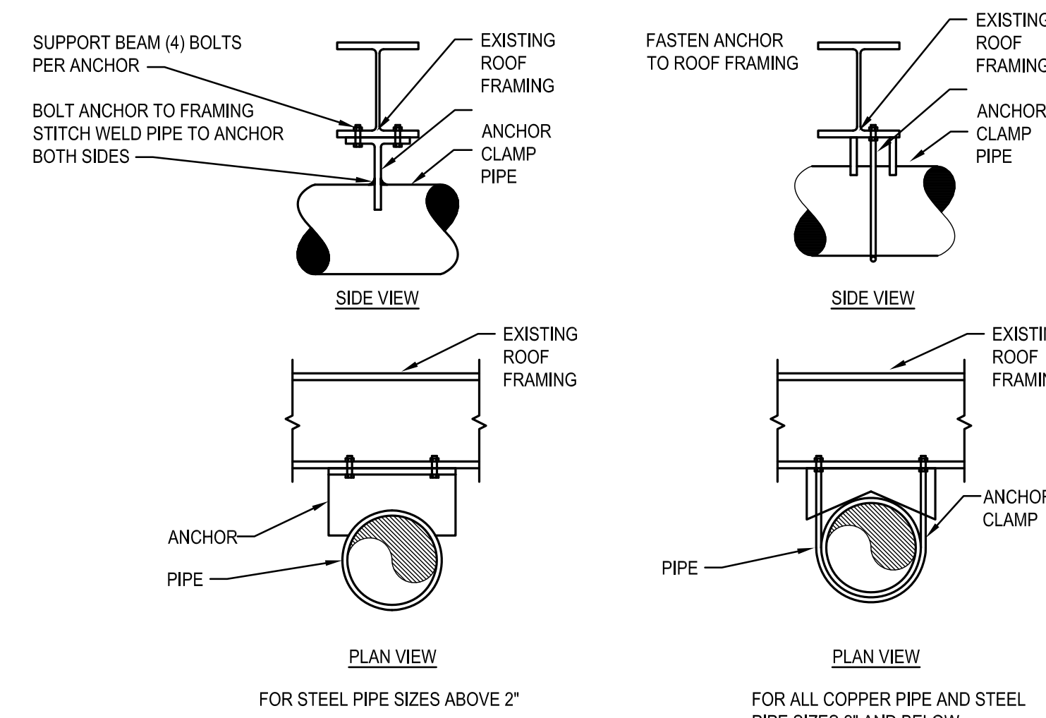
DETAIL - PIPE ANCHOR 5 SCALE: NOT TO SCALE
