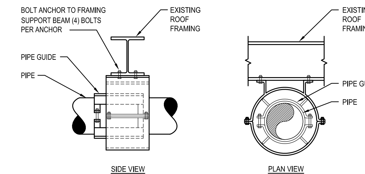
DETAIL - PIPE SPIDER GUIDE DETAIL 1 SCALE: NOT TO SCALE
