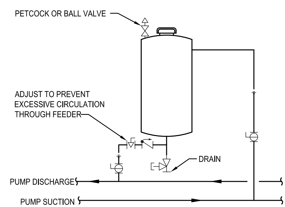
DETAIL - BYPASS CHEMICAL FEEDER 13 SCALE: NOT TO SCALE
