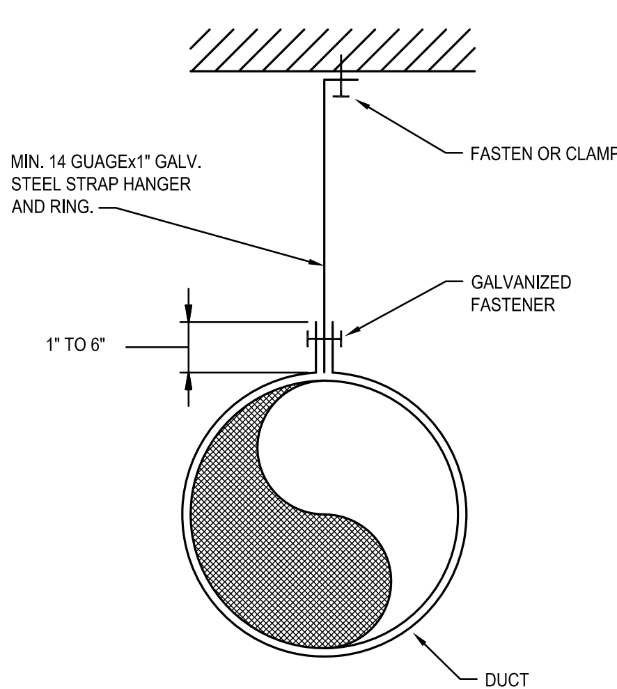
DETAIL - ROUND DUCT HANGER 14 SCALE: NOT TO SCALE
