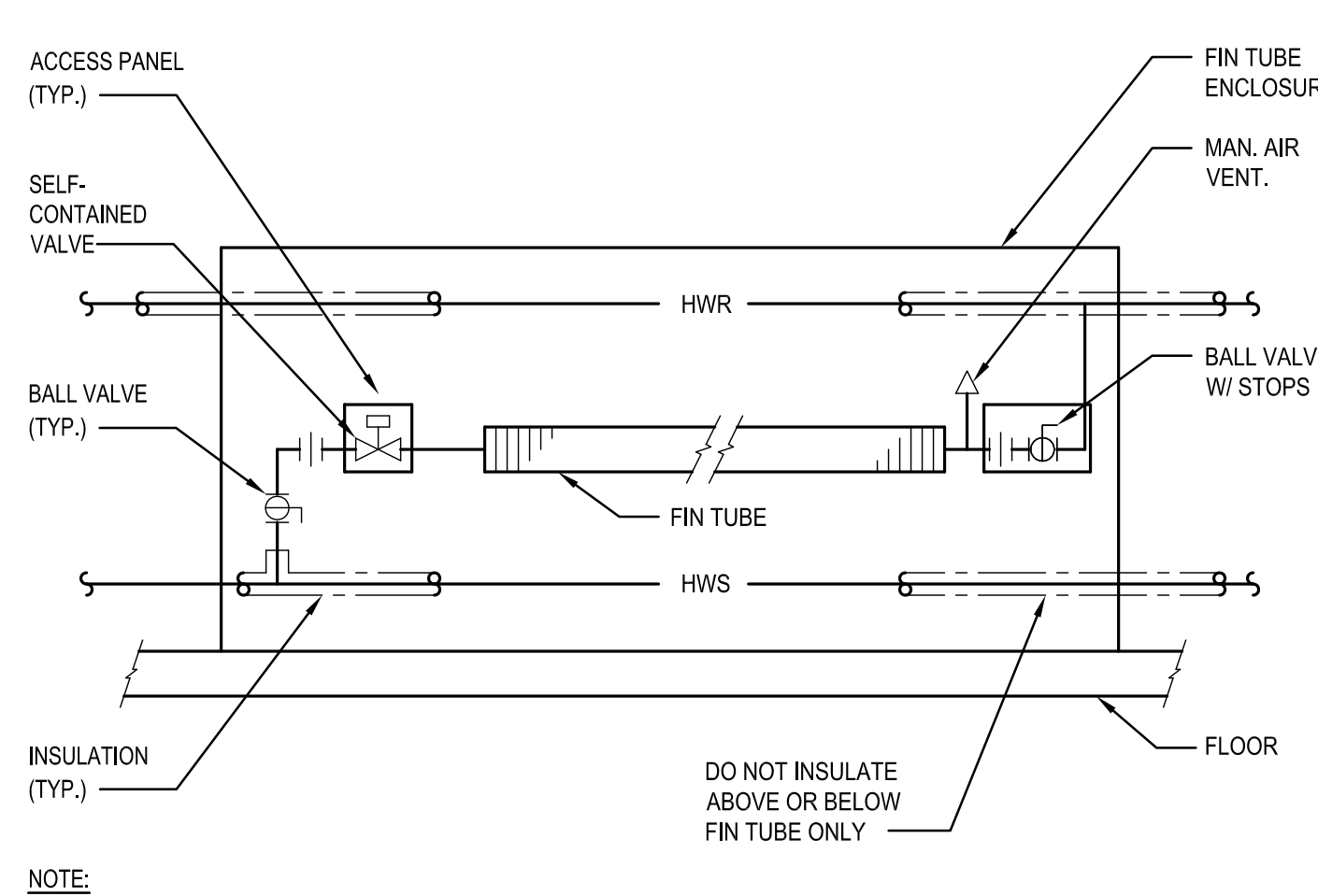
DETAIL - HOT WATER FTR PIPING 2 SCALE: NOT TO SCALE
