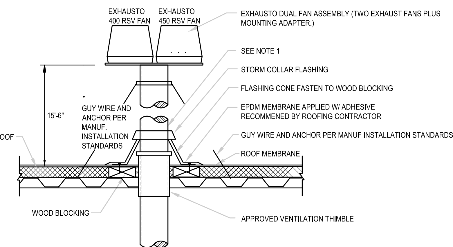
DETAIL - POSITIVE PRESSURE FLUE 12 SCALE: NOT TO SCALE
