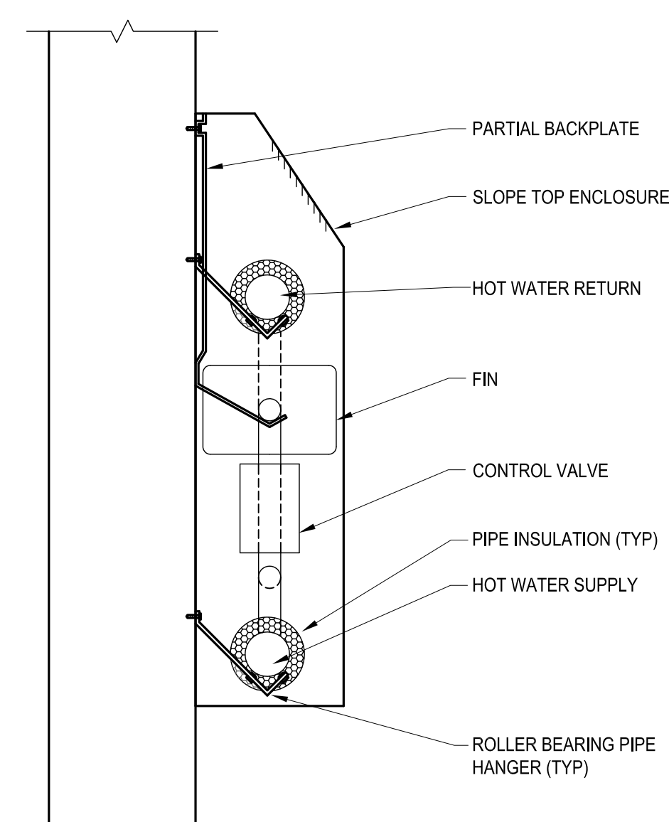
DETAIL - HOT WATER FIN TUBE SECTION 9 SCALE: NOT TO SCALE
