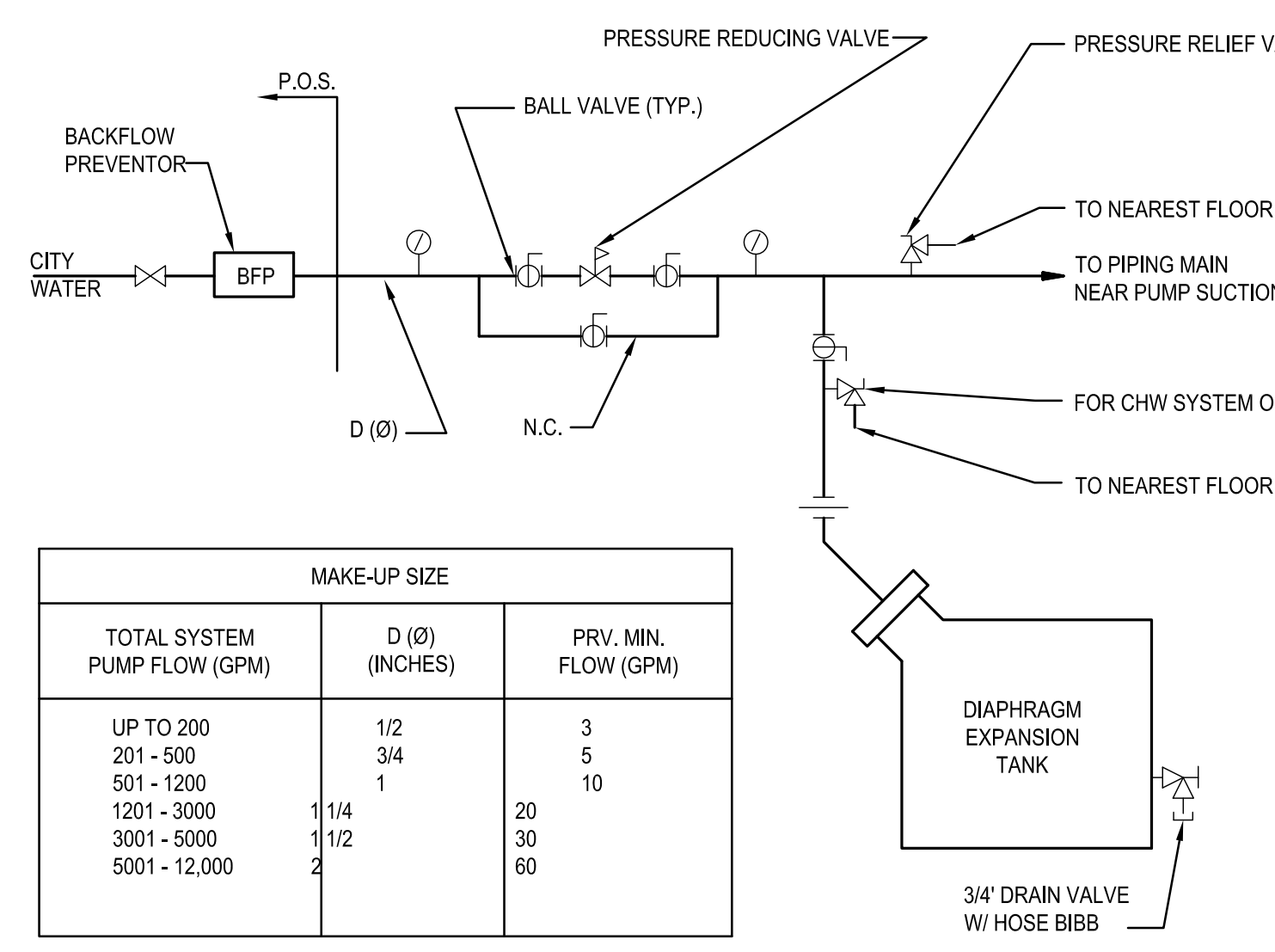
DETAIL - MAKE-UP WATER & DIAPHRAGM EXPANSION TANK 8 SCALE: NOT TO SCALE
