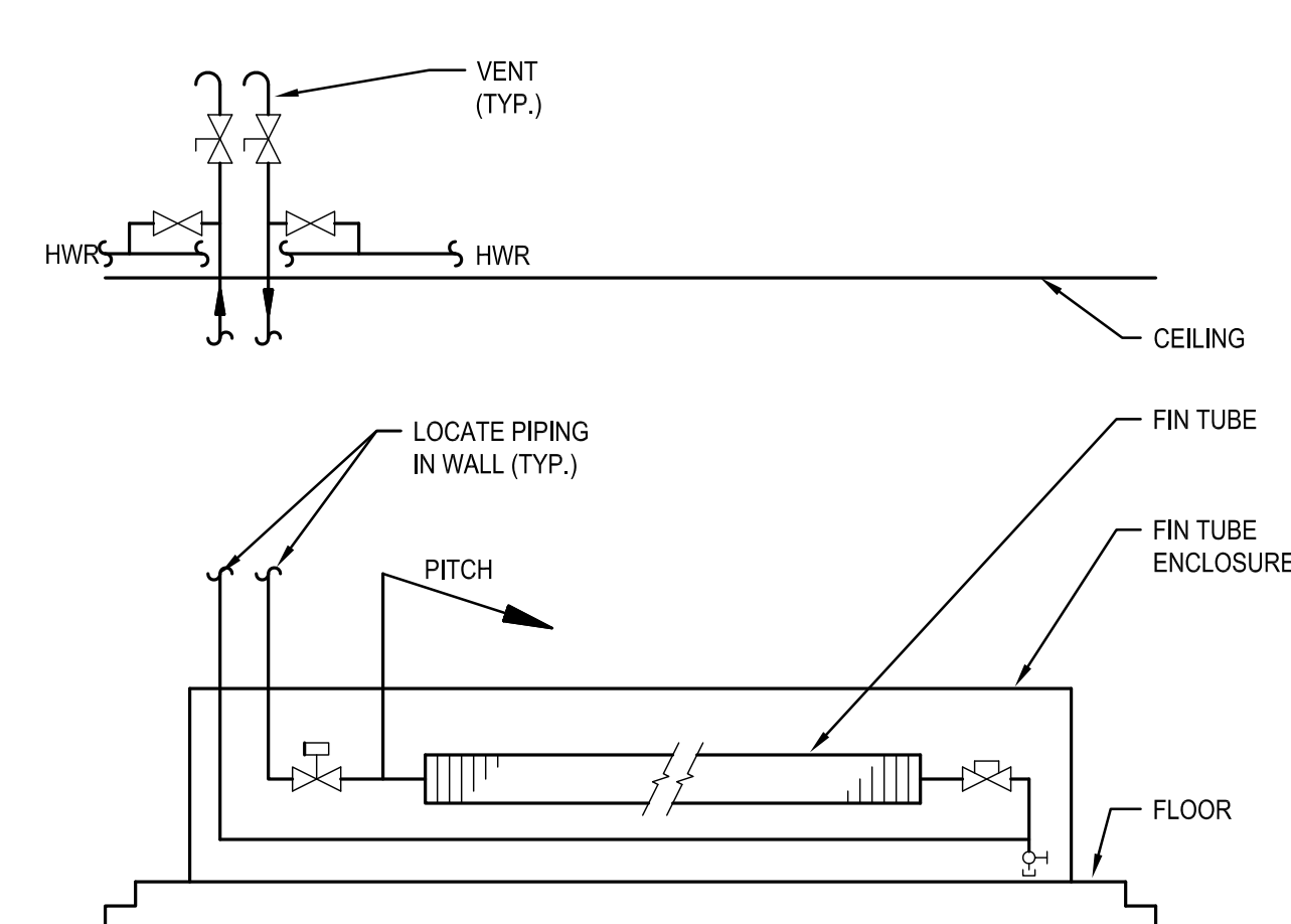
DETAIL - HOT WATER FTR PIPING 10 SCALE: NOT TO SCALE
