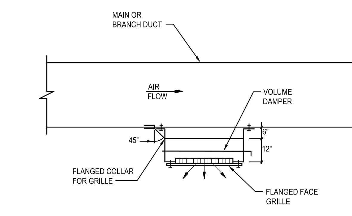
DETAIL - DUCT SUPPLY GRILLE TAKE OFF 3 SCALE: NOT TO SCALE
