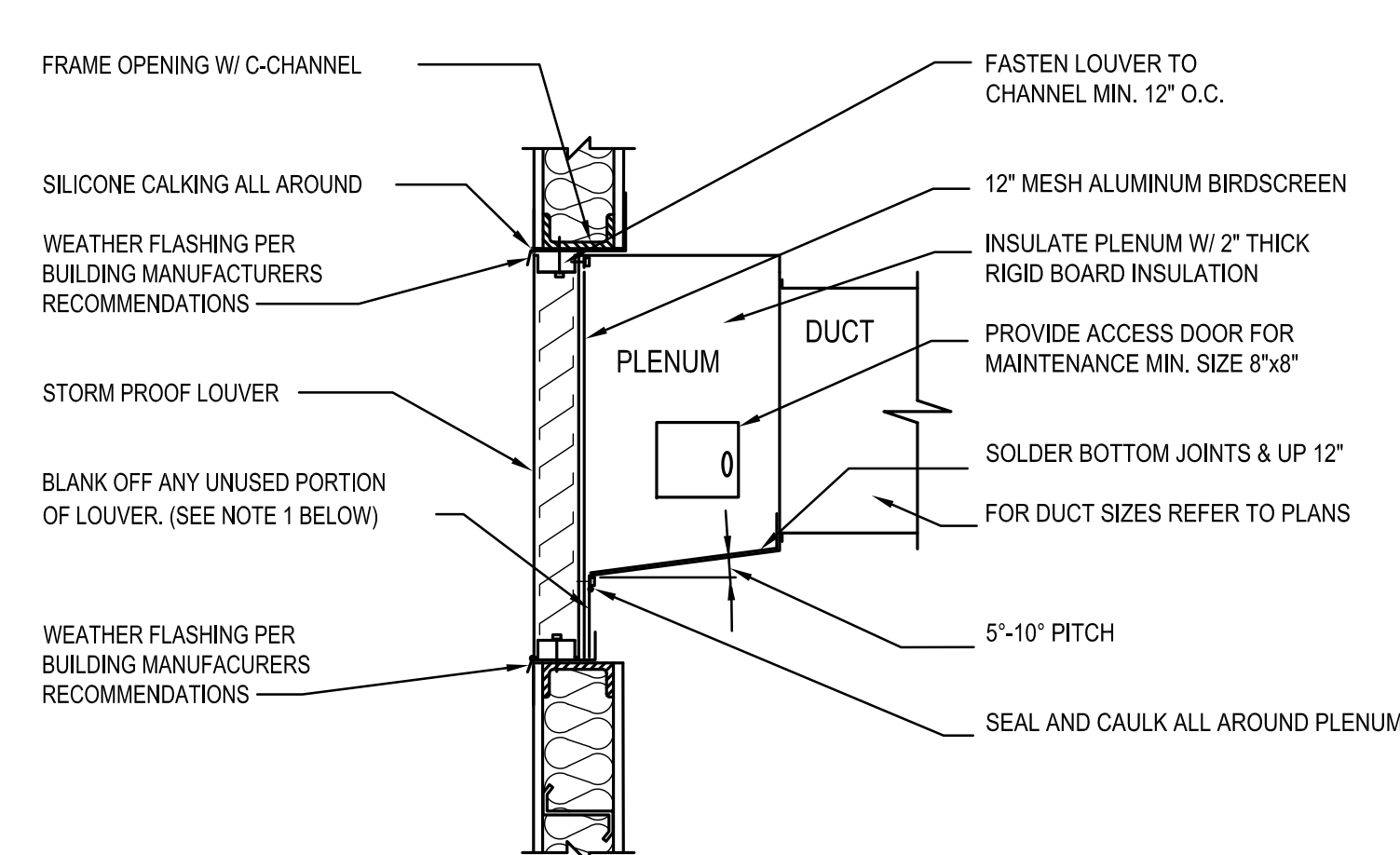
DETAIL - LOUVER CONNECTION 16 SCALE: NOT TO SCALE
