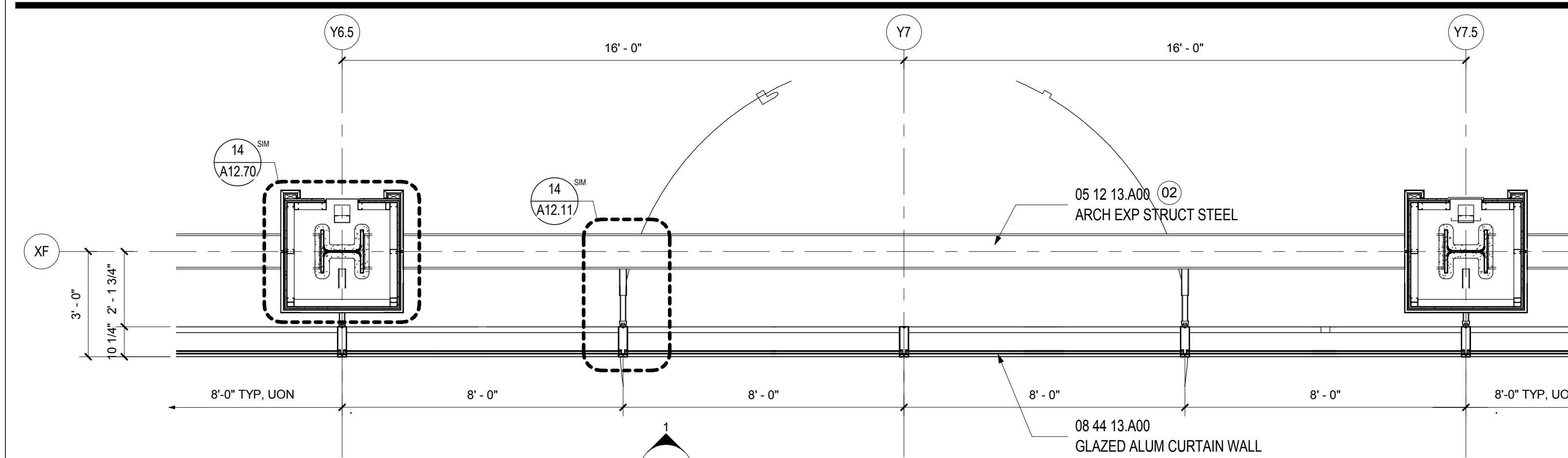
WALL TYPE D.1 - PLAN LEVEL 3
