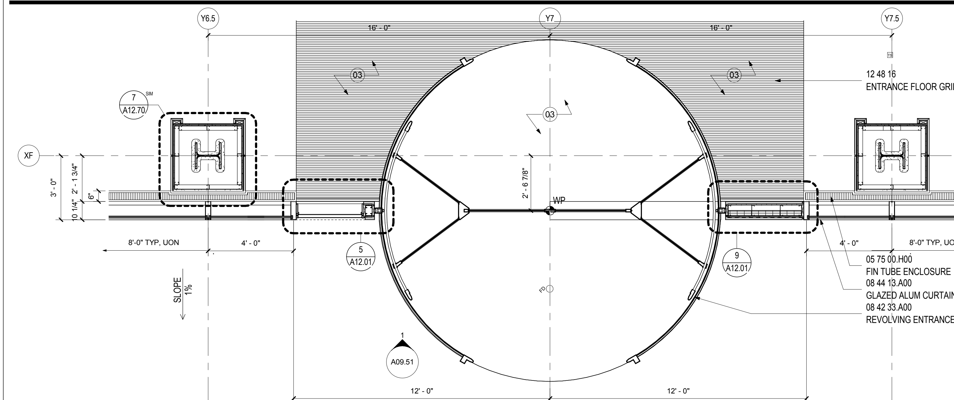
WALL TYPE D.1 - PLAN LEVEL 2
