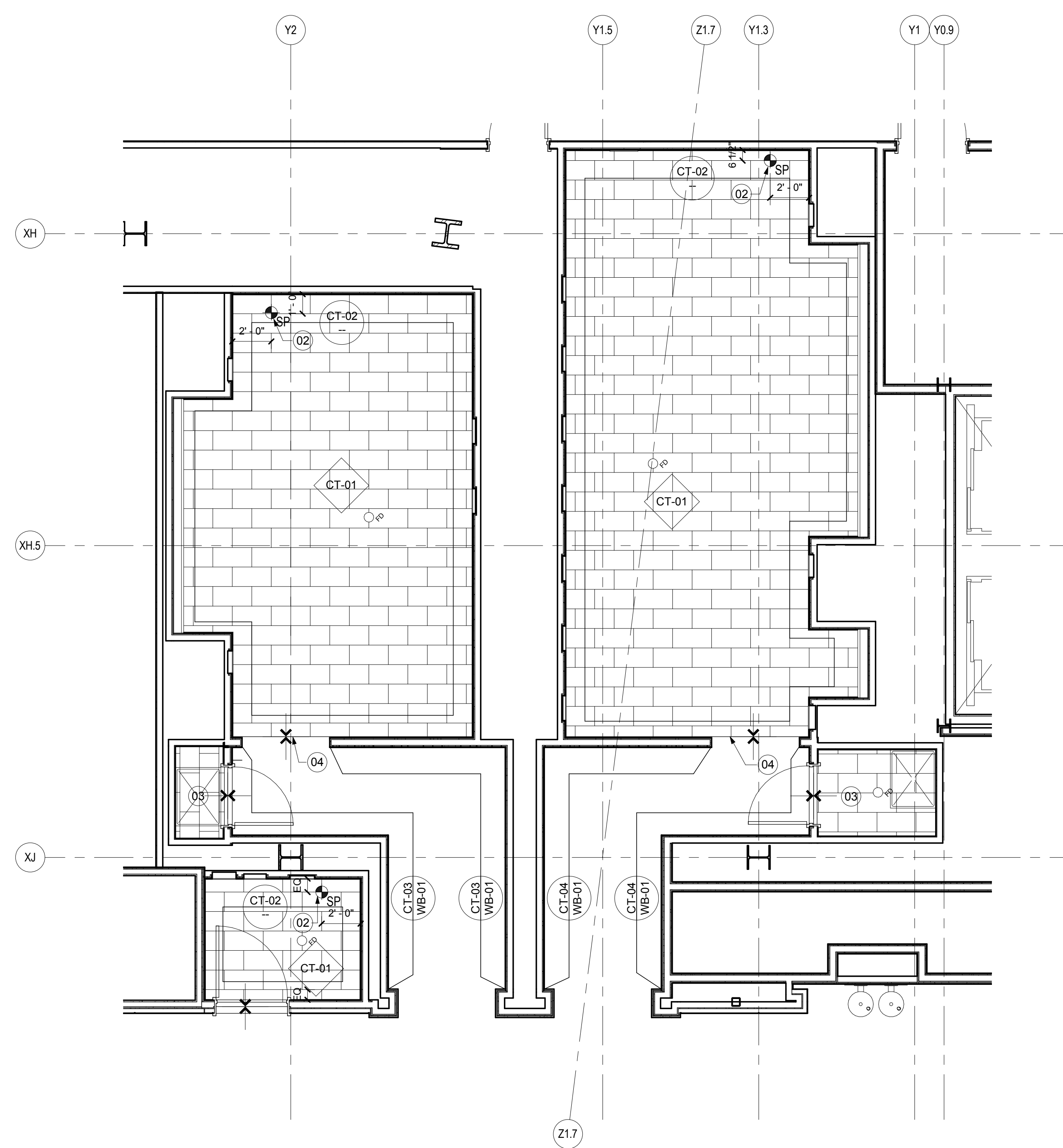
ENLARGED PLAN-LEVEL 3 RESTROOMS - FINISH PLAN
