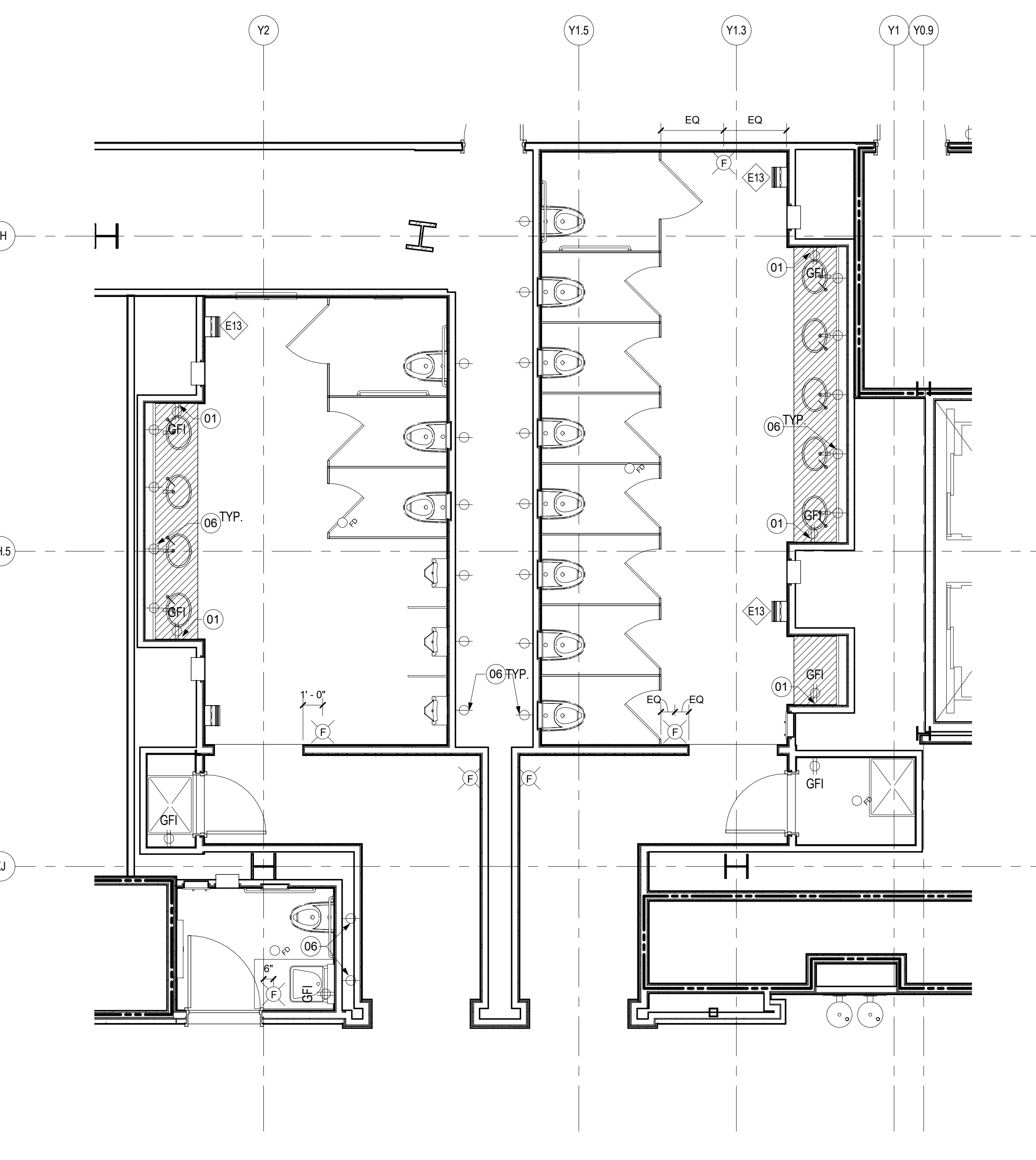
ENLARGED PLAN-LEVEL 3 RESTROOMS - POWER & COMM. PLAN
