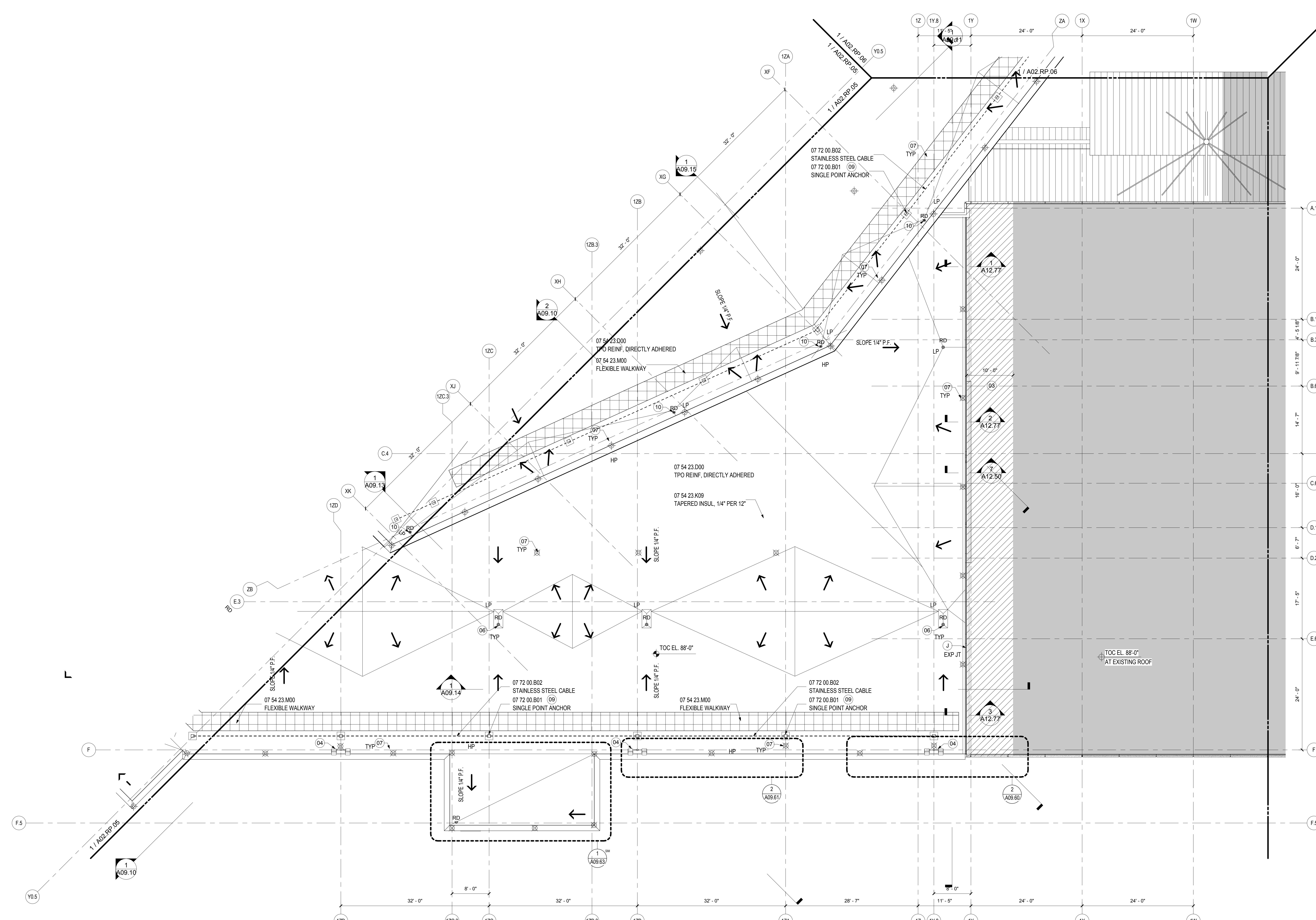
CONSTRUCTION PLAN - ROOF - ZONE 4 SCALE: 1/8" = 1'-0"
