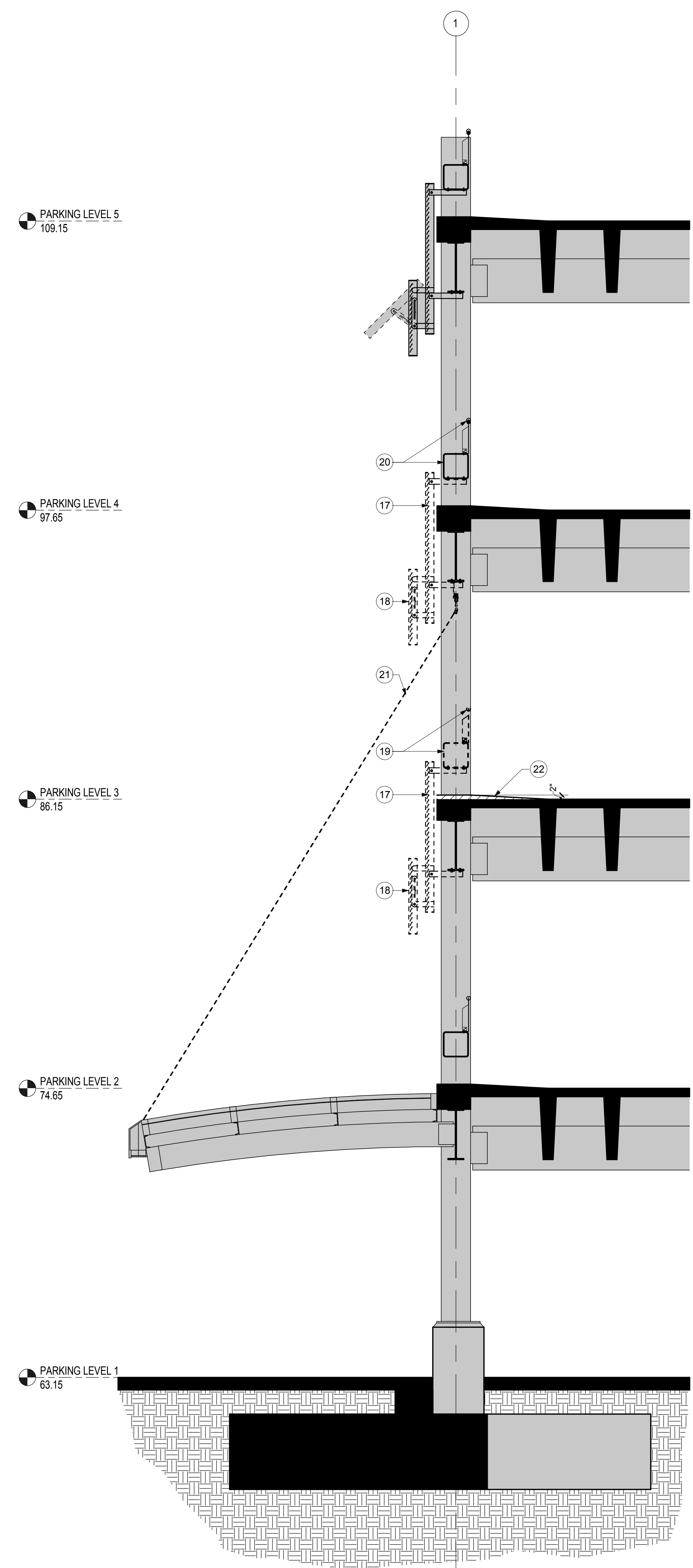
EXISTING GARAGE WALL SECTION
