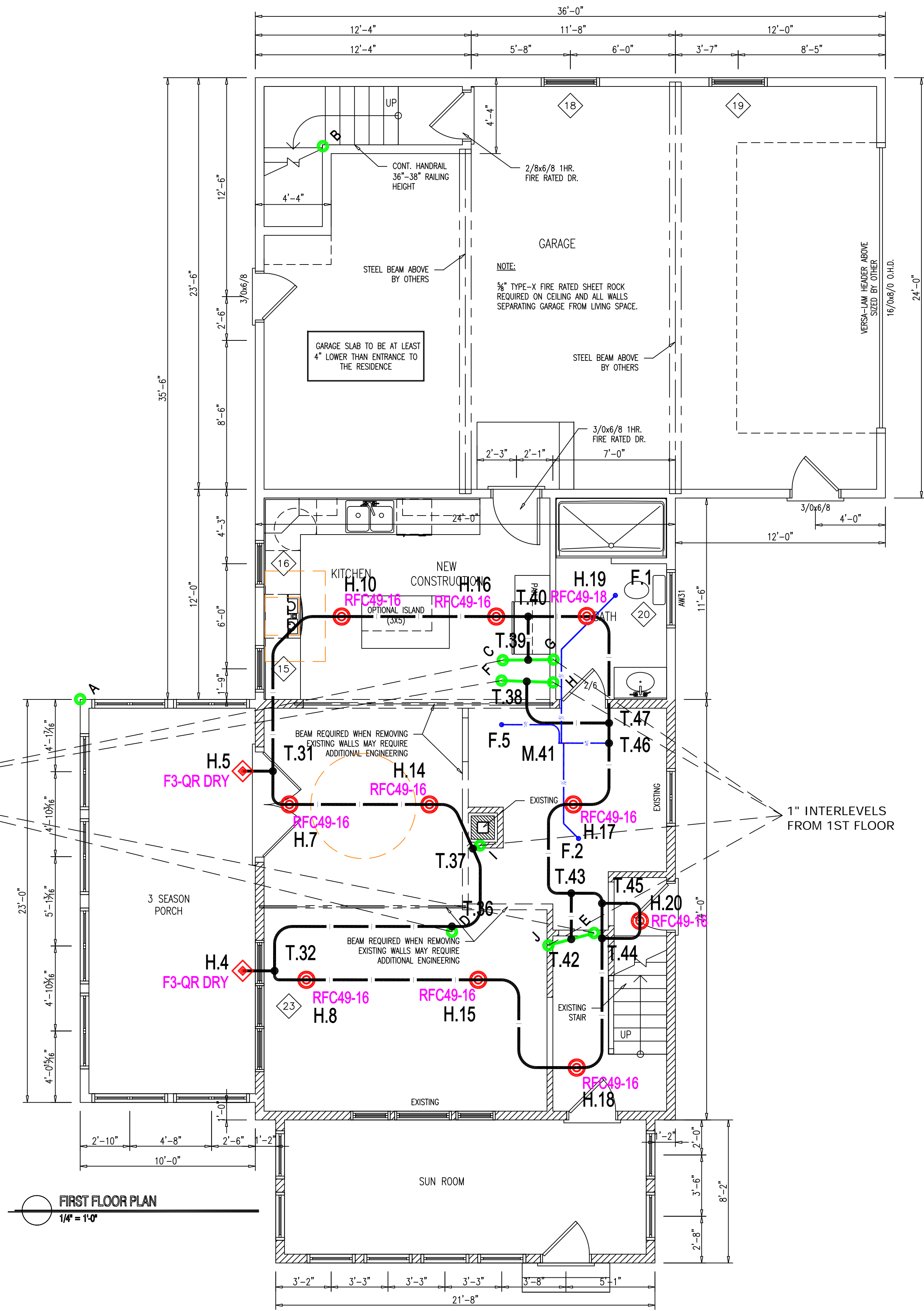
1 F101 FIRST FLOOR 1/4" = 1'-0"
