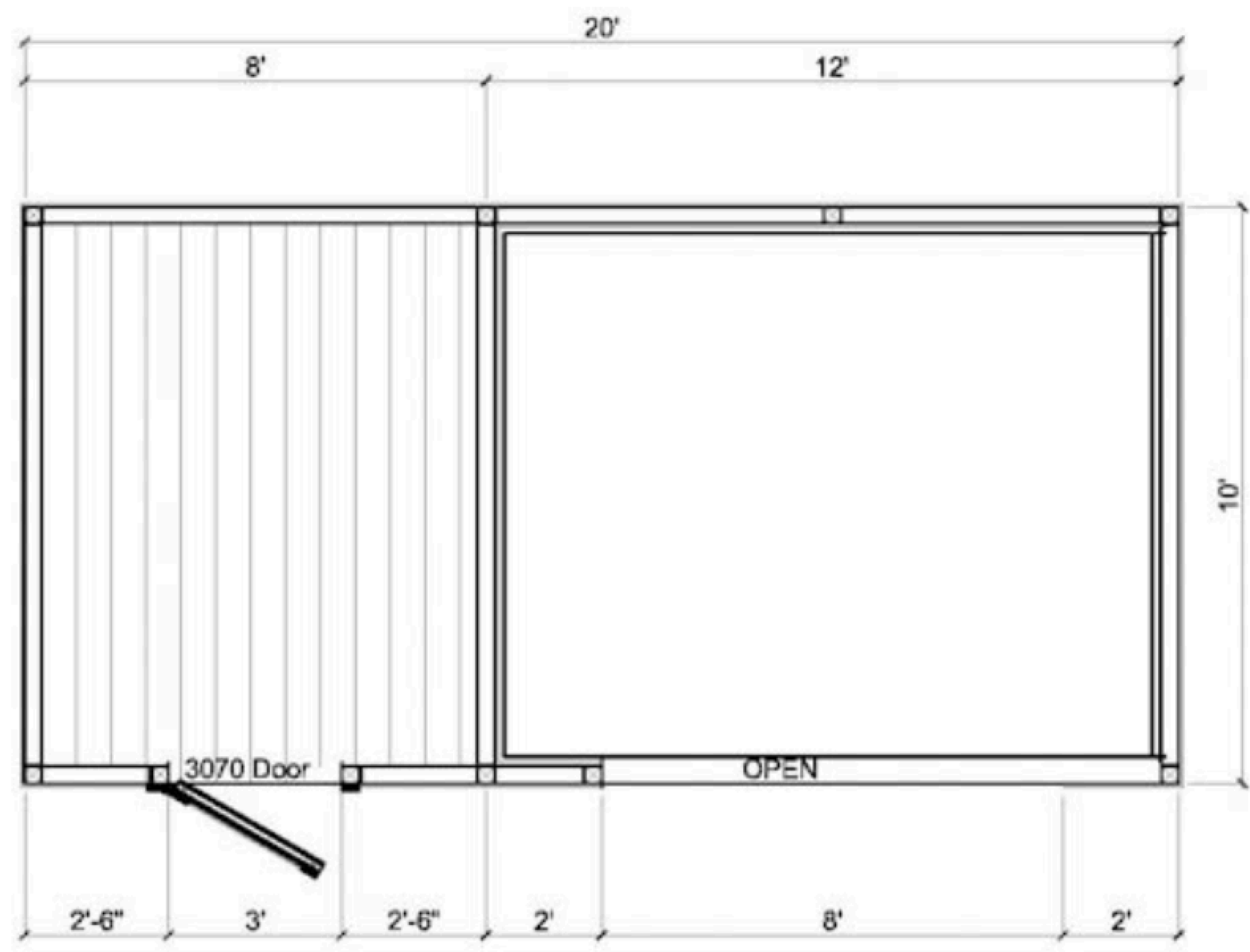
10x20 2 STALL RUN IN SHED WITH TACK ROOM FLOOR PLAN
