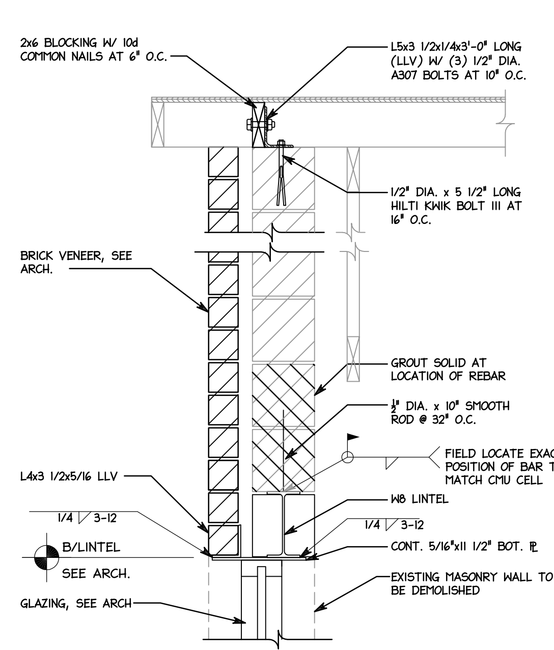
LINTEL DETAIL SCALE T = 1-0"
