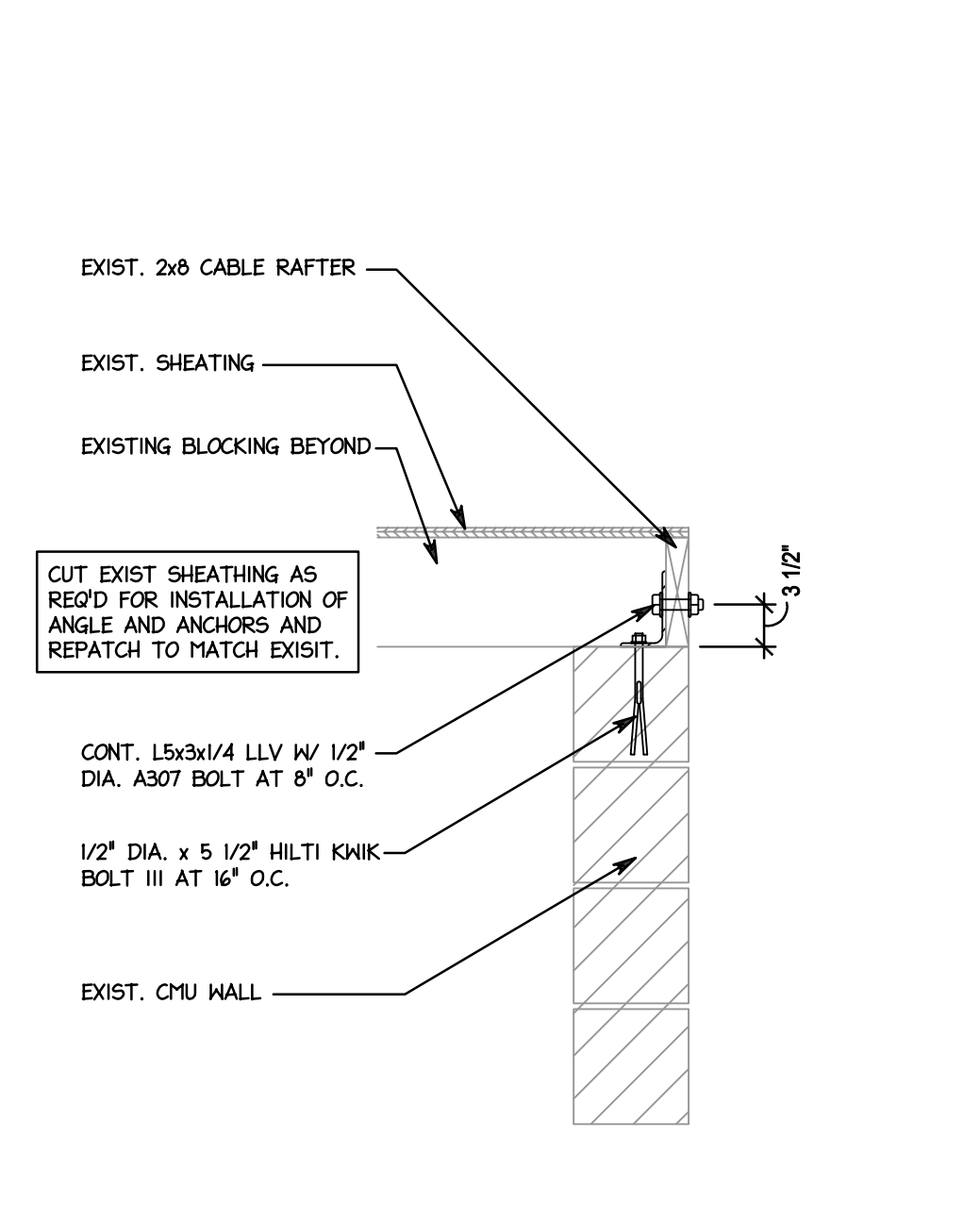
END RAFTER CONNECTION SCALE T = 1-0"
