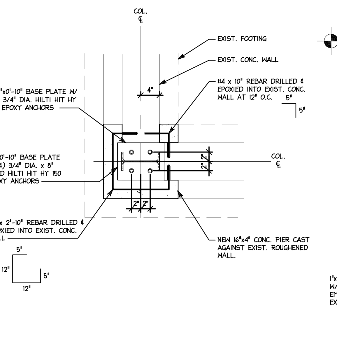
BASE PLATE SCALE T = 1-0"
