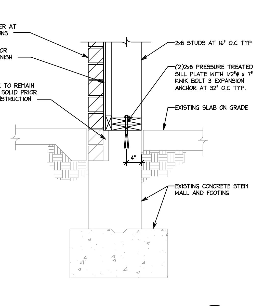
FOUNDATION DETAIL SCALE T = 1-0"
