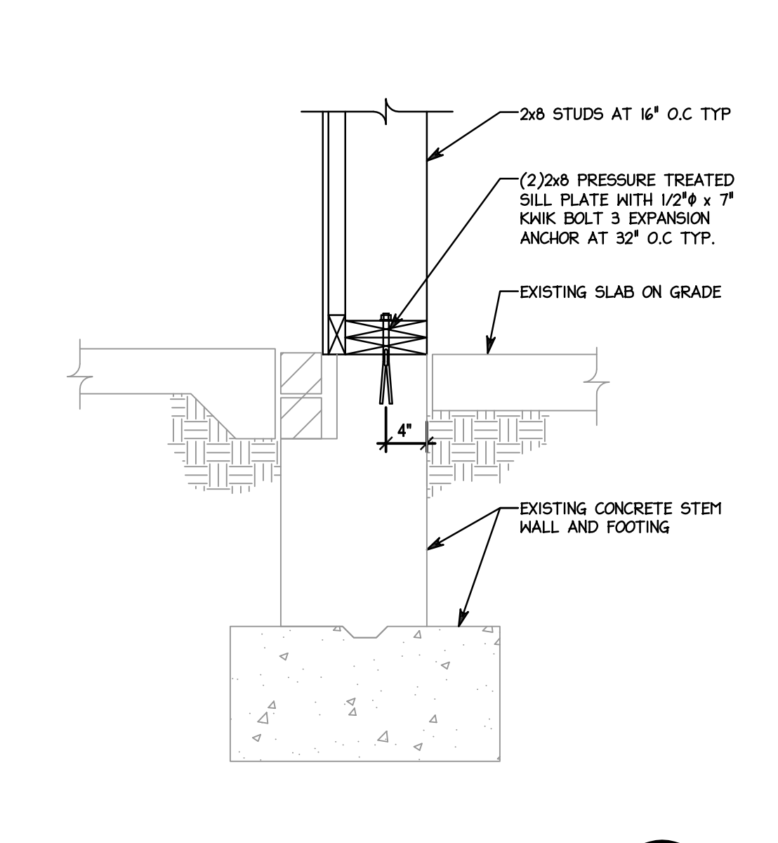
FOUNDATION DETAIL SCALE T = 1-0"
