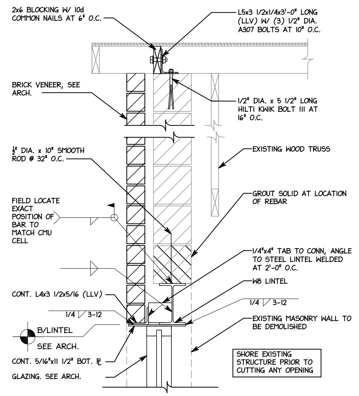
LINTEL DETAIL SCALE T = 1-0"
