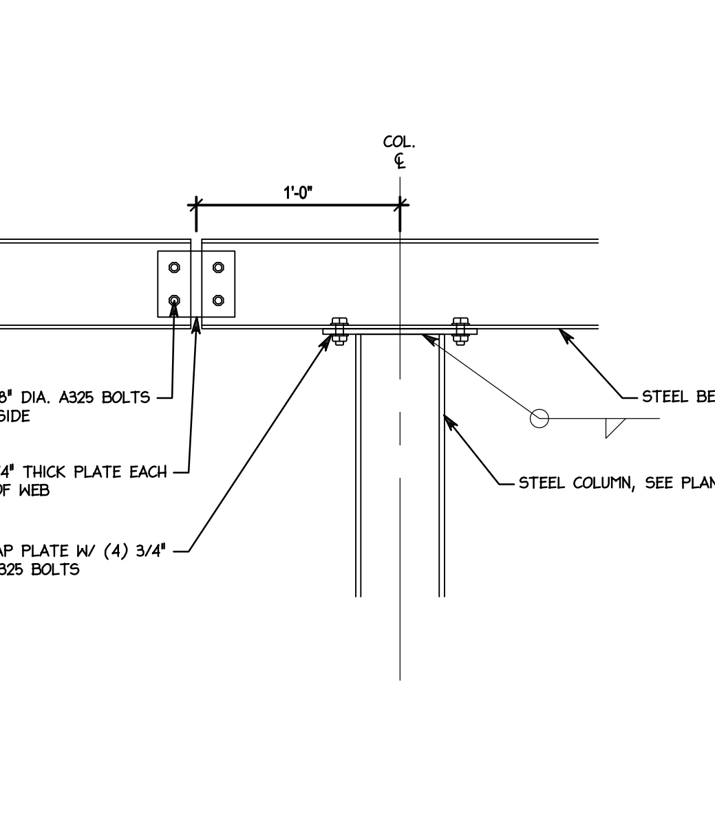
BEAM / COLUMN CONNECTION SCALE T = 1-0"
