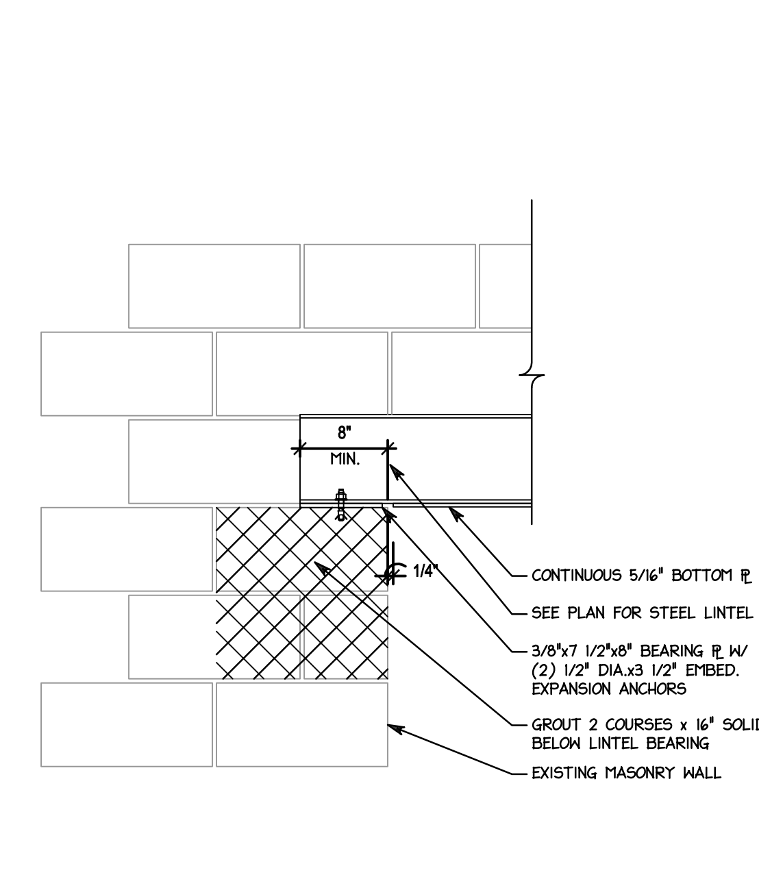
LINTEL BEARING SCALE T = 1-0"
