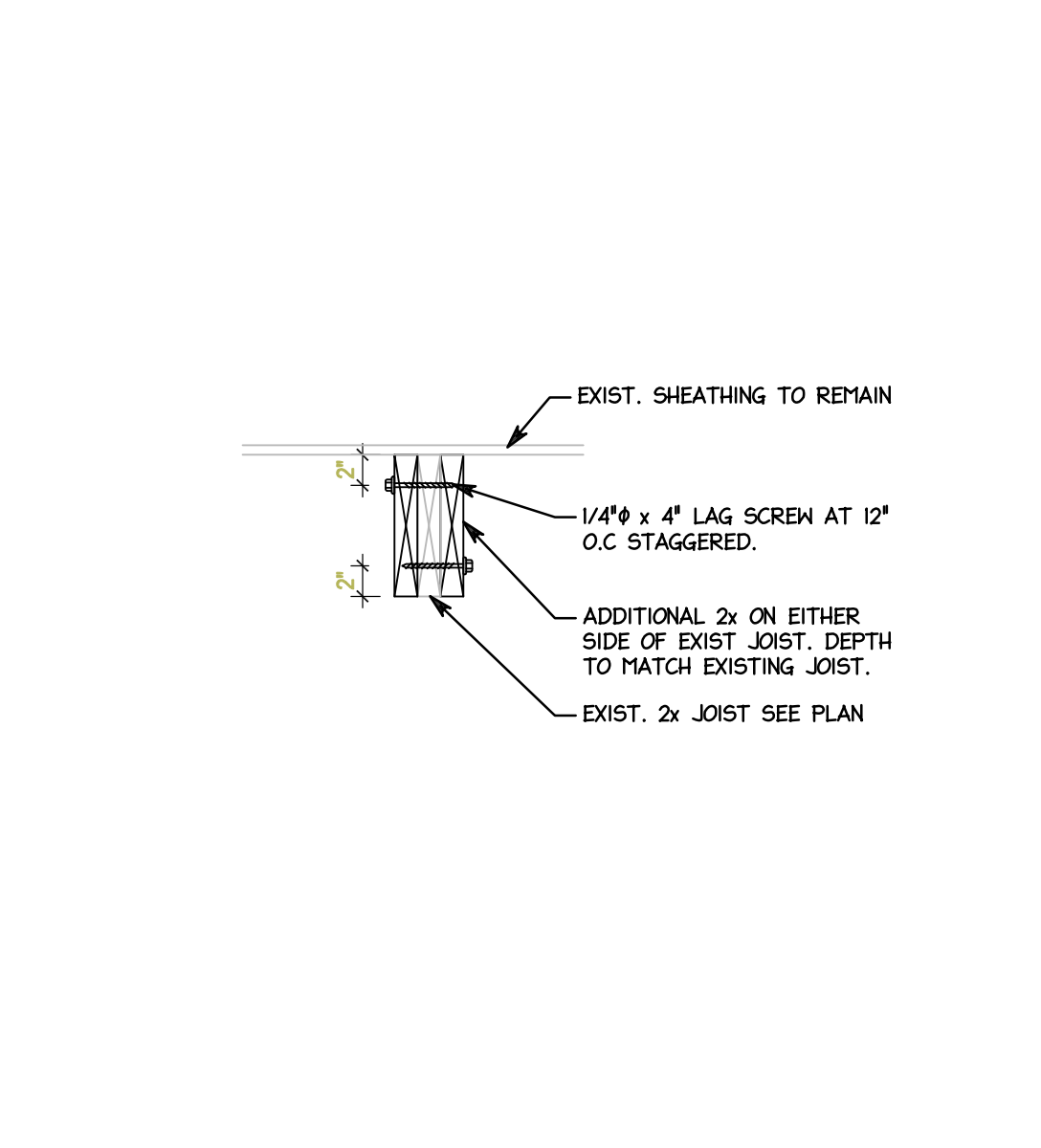
JOIST REINFORCING SCALE T = 1-0"
