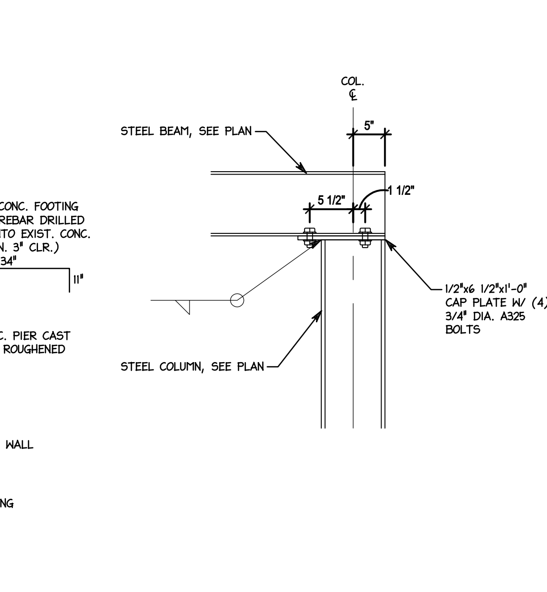
BEAM / COLUMN CONNECTION SCALE T = 1-0"
