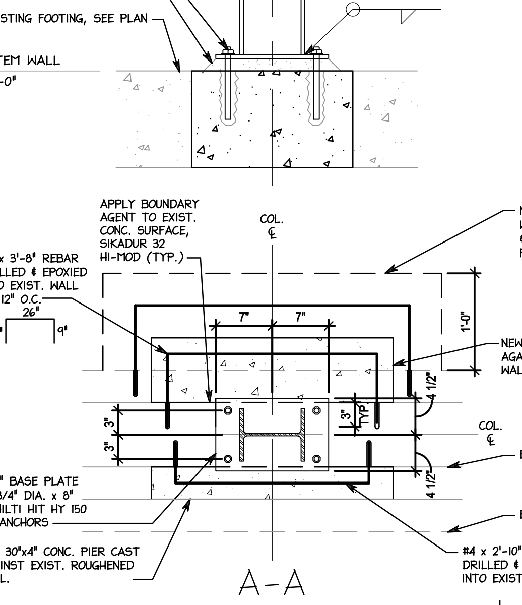
BASE PLATE SCALE T = 1-0"
