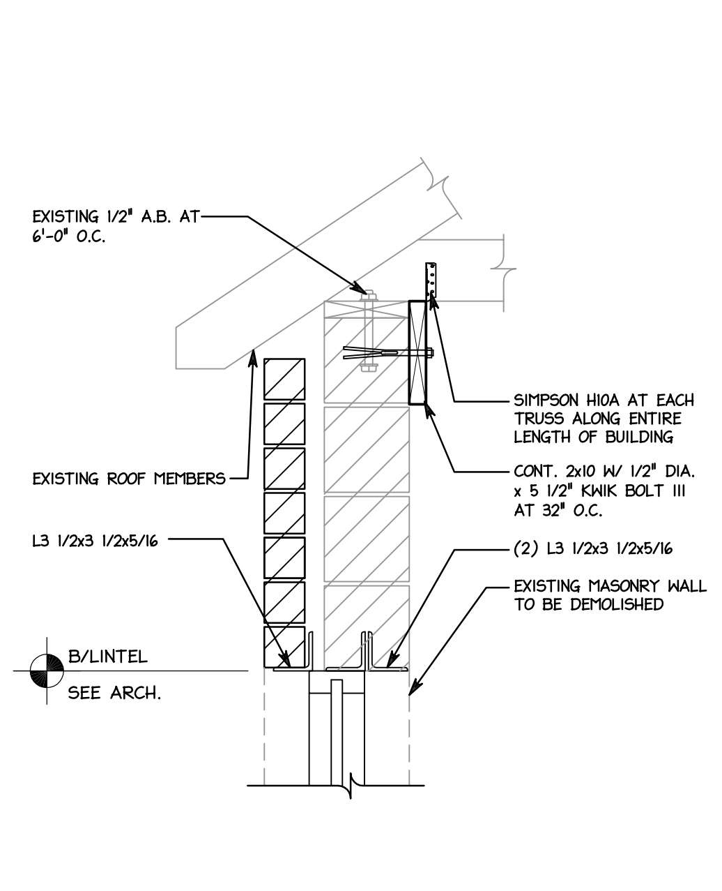
LINTEL DETAIL SCALE T = 1-0"
