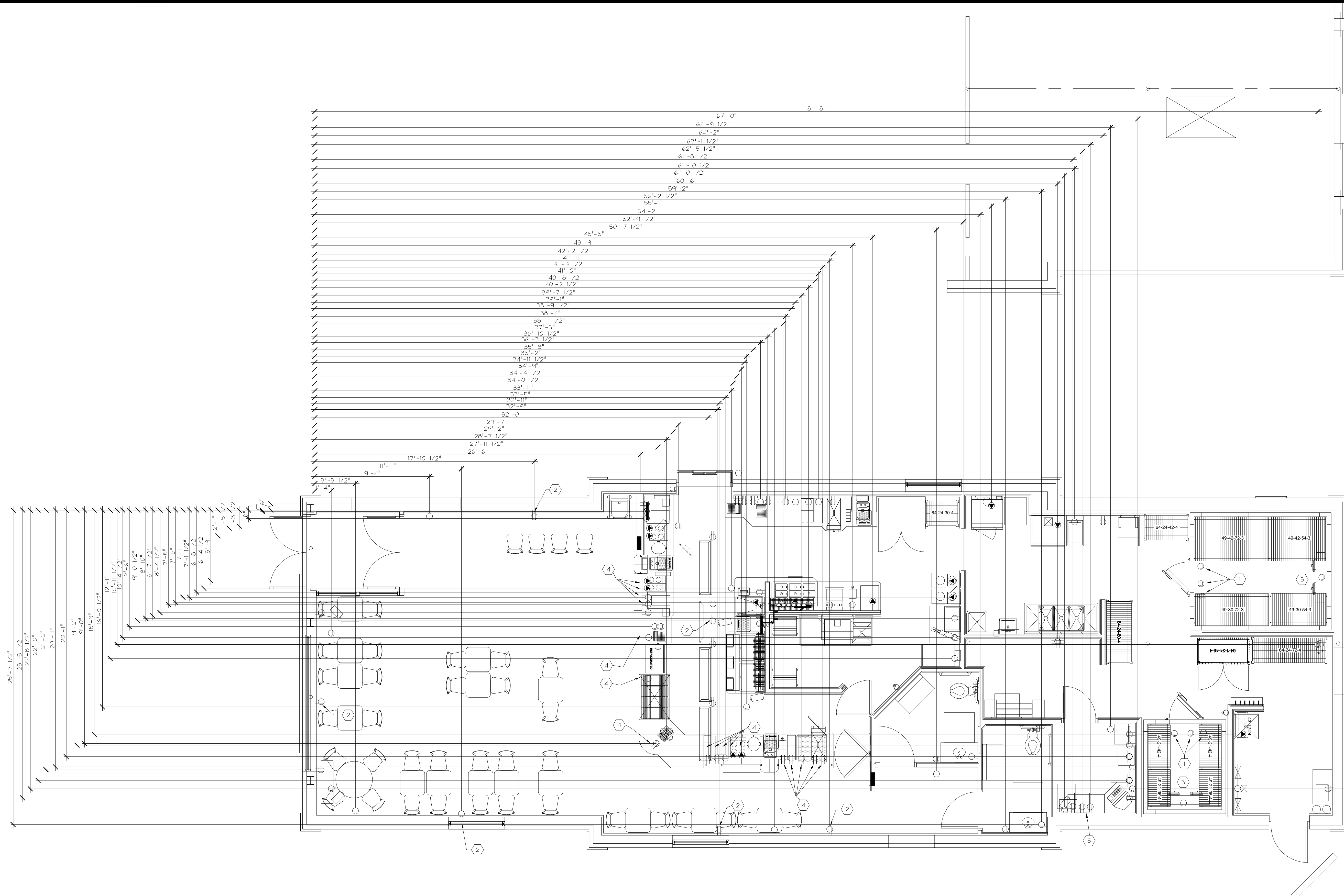
ELECTRICAL OUTLET DIMENSION PLAN 1/4" = 1'-0"
