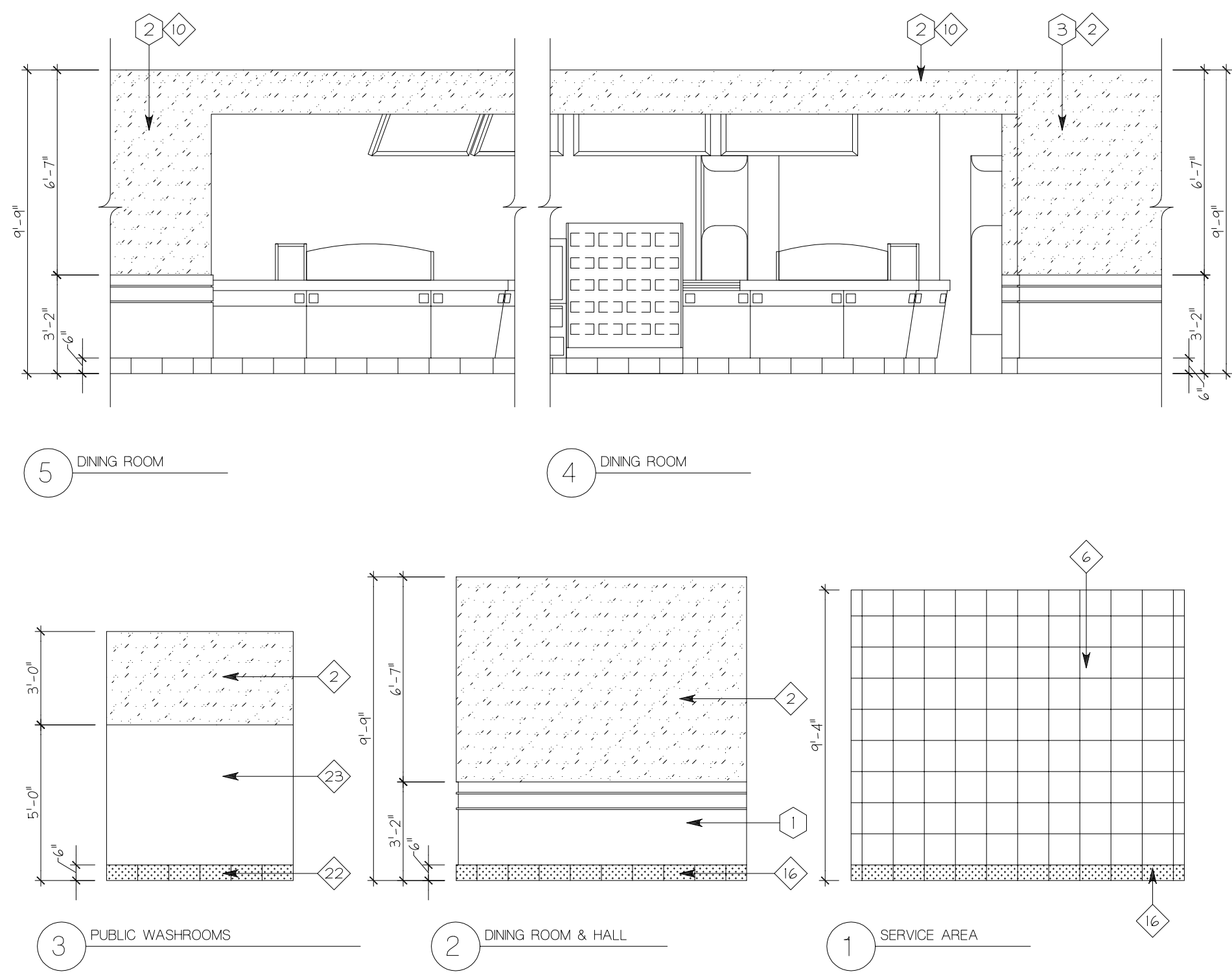
TYPICAL INTERIOR ELEVATIONS (scotch and amber scheme)
