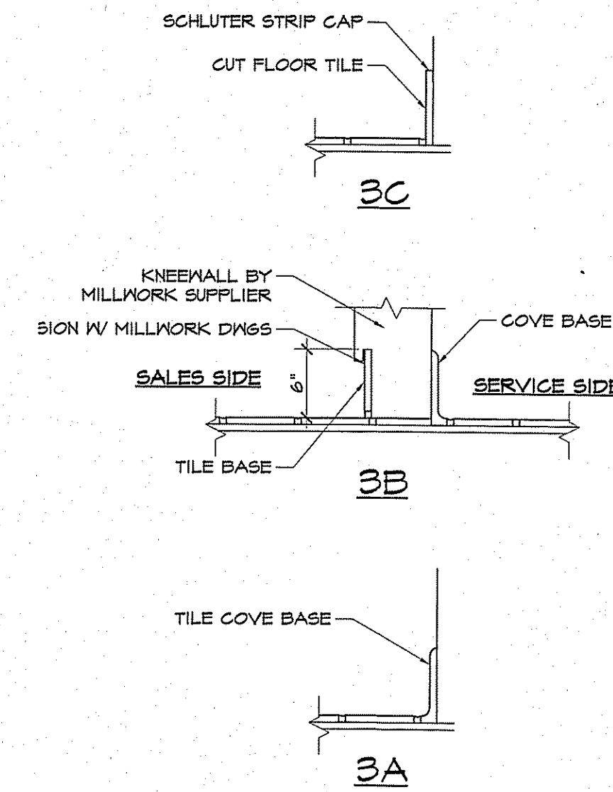
3 TILE BASE DETAILS A1.2 SCALE: NOT TO SCALE
