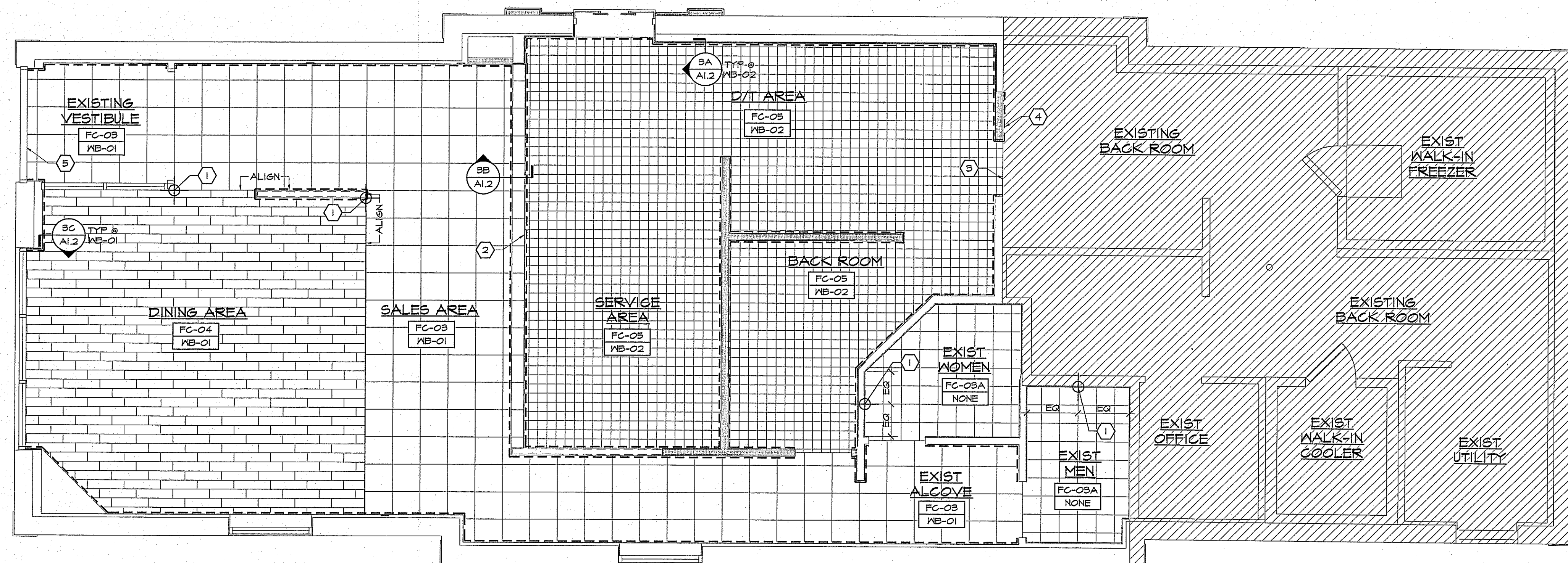
1 FLOOR FINISH PLAN SCALE: 1/4" = 1'-0"
