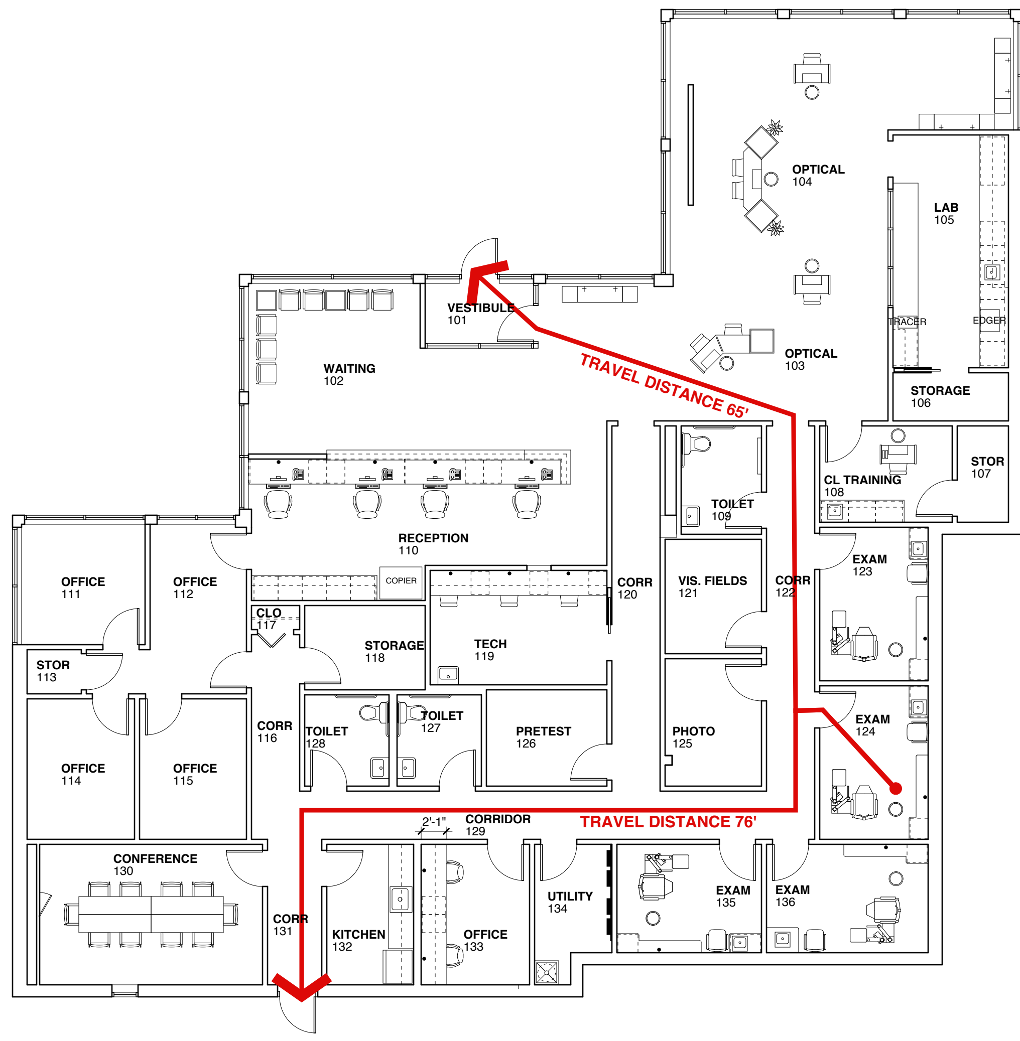
1 LIFE SAFETY PLAN SCALE: 1/8" = 1'-0"
