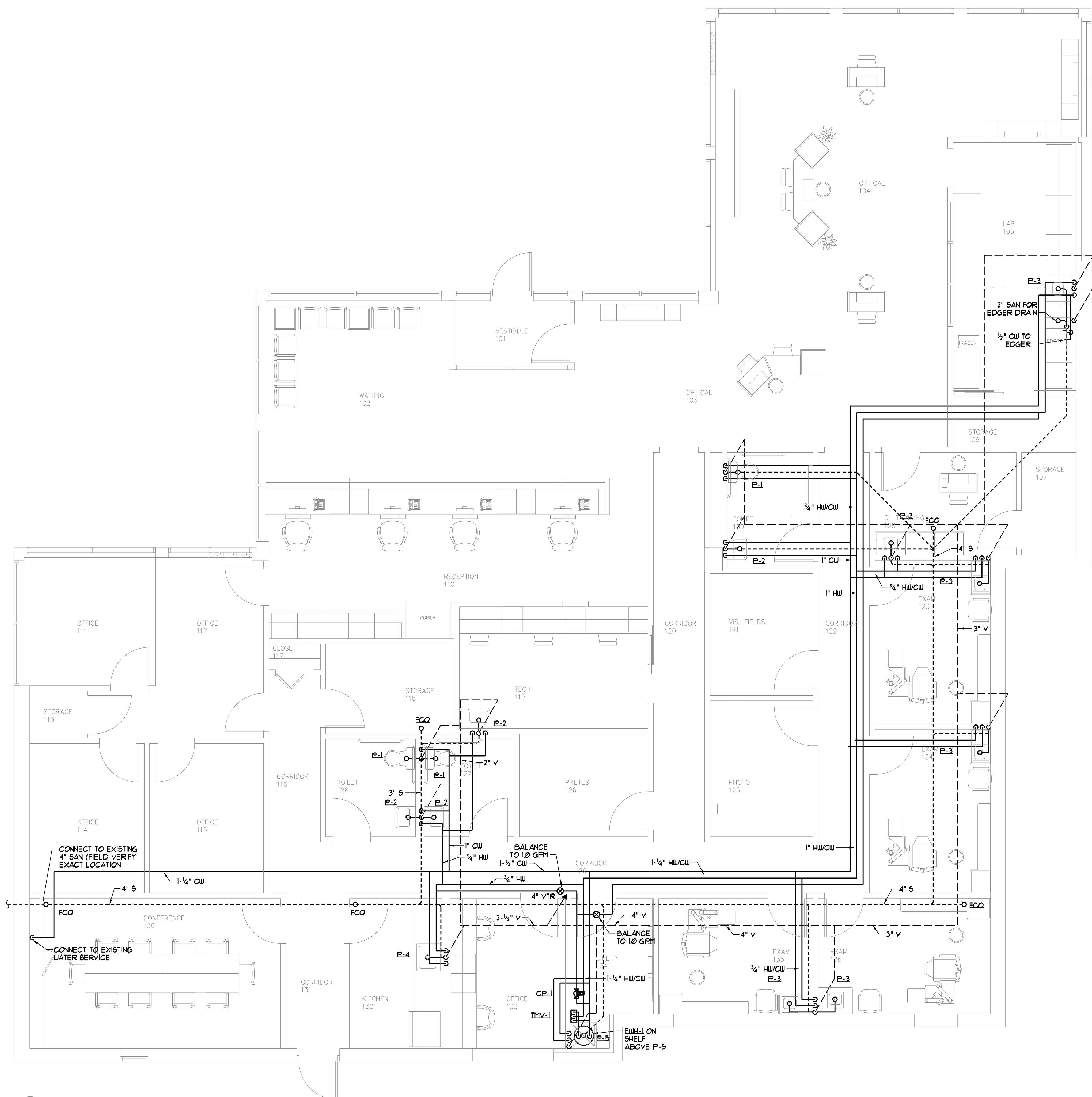
1 FLOOR PLAN SCALE: 1/4" = 1'-0" 2' 4' 8'
