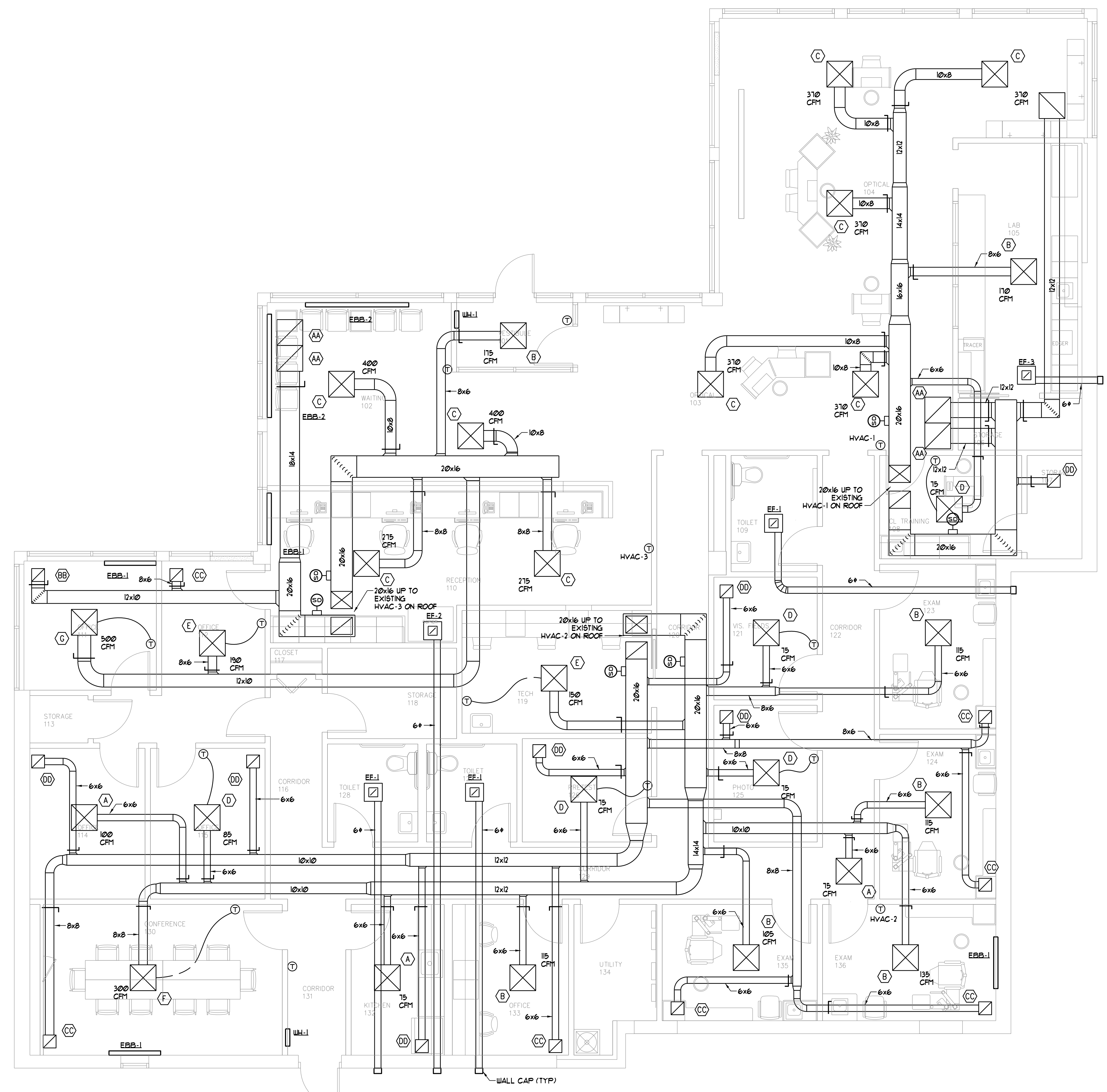
1 FLOOR PLAN SCALE: 1/4" = 1'-0" 1" 2" 4" 8"
