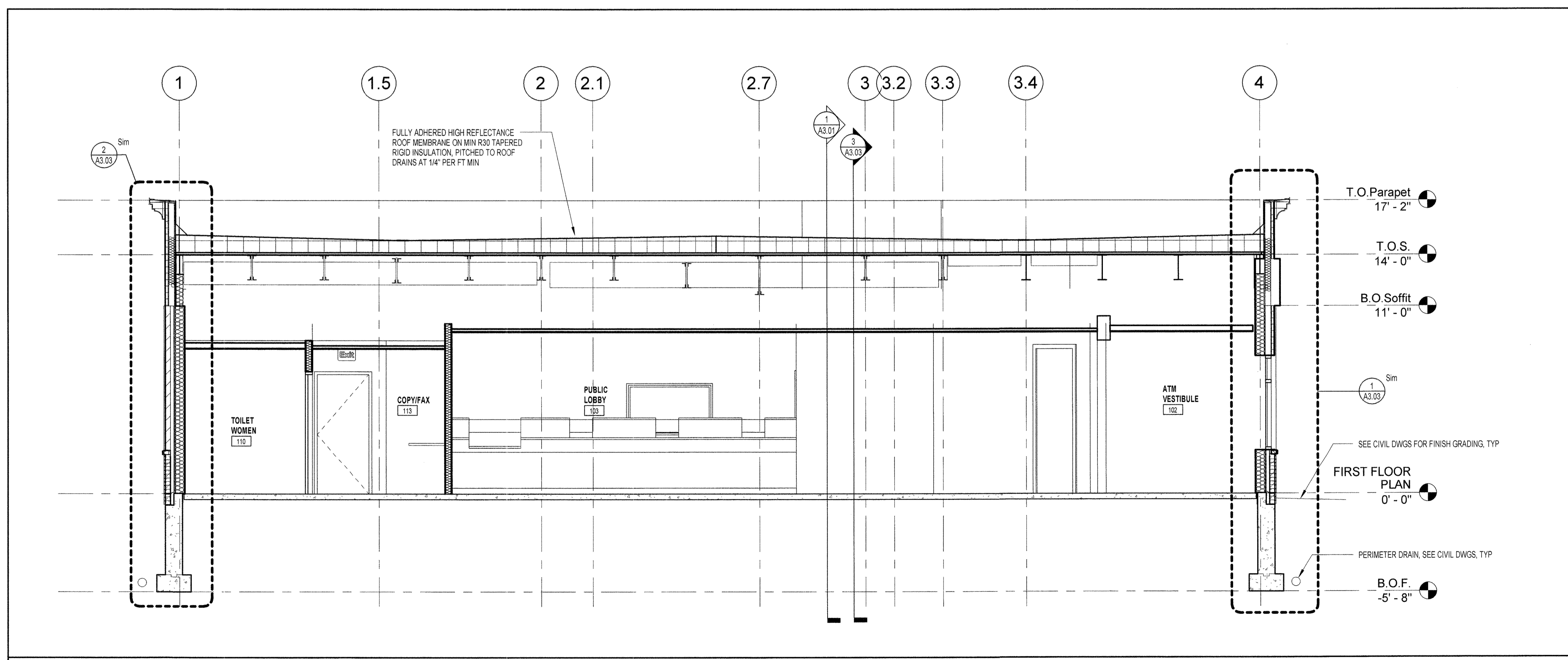
② BUILDING SECTION B 1/4" = 1'-0"
