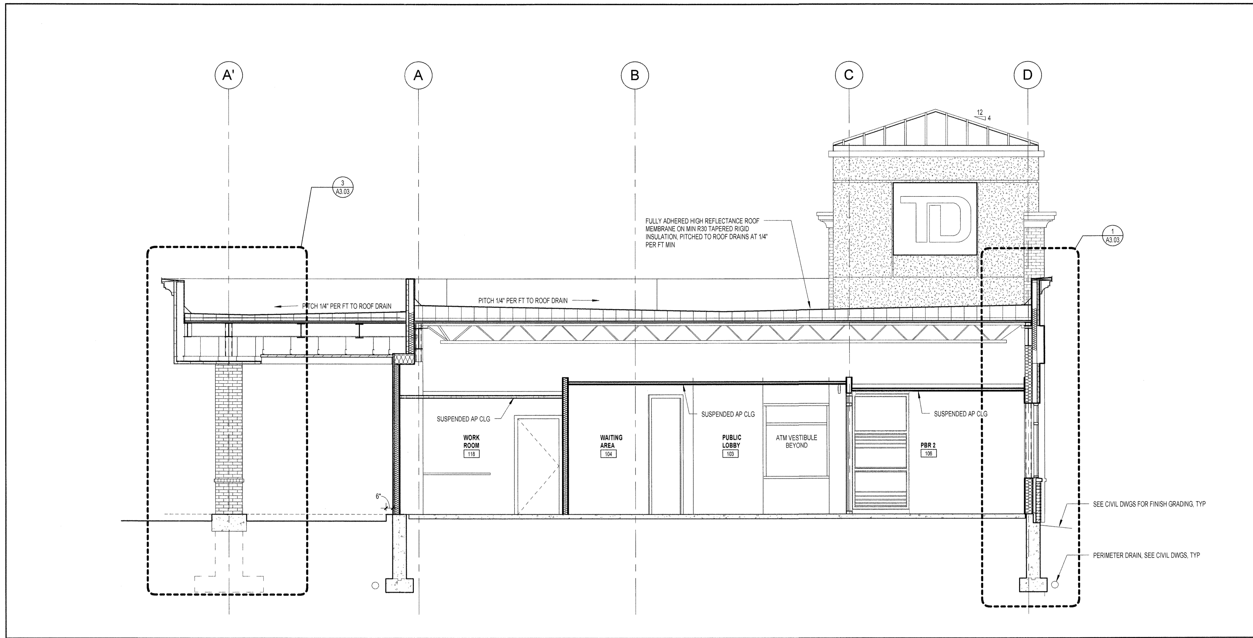
① BUILDING SECTION A 1/4" = 1'-0"
