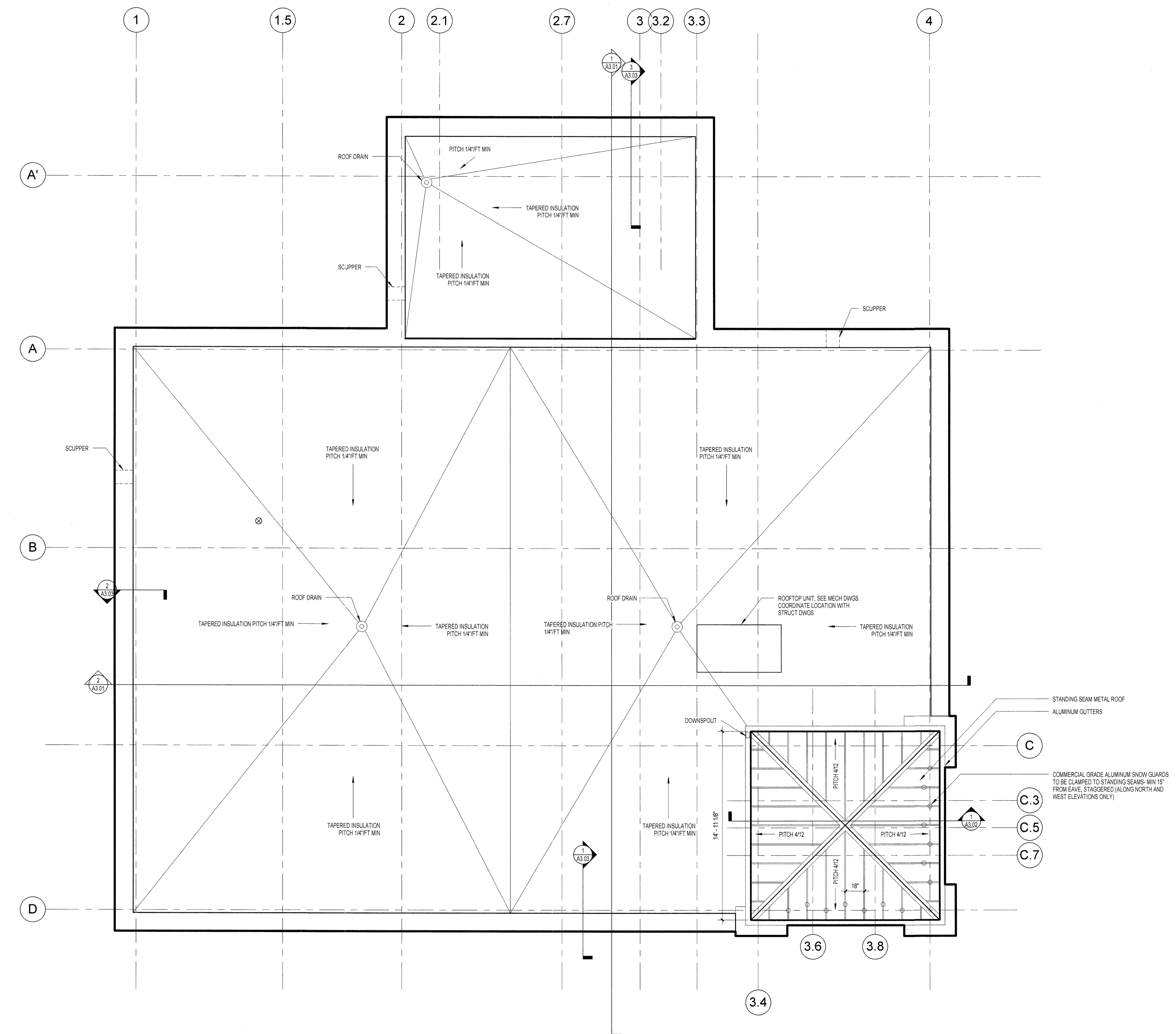
① ROOF PLAN 1/4" = 1'-0"
