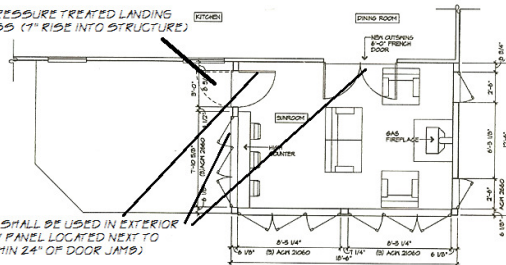
SUNROOM PLAN (ANDERSON A-SERIES) 1/4" x 11'-0"
