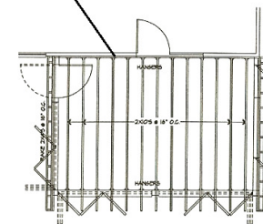
SUNROOM ROOF FRAMING PLAN 1/4" x 11'-0"
