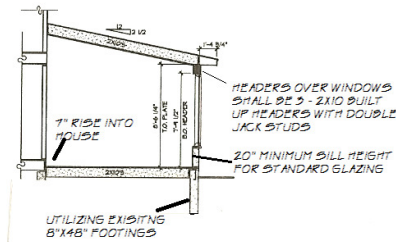
SECTION 1/4" x 11'-0"
