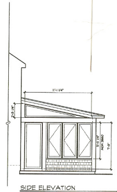
SIDE ELEVATION 1/4" x 11'-0"
