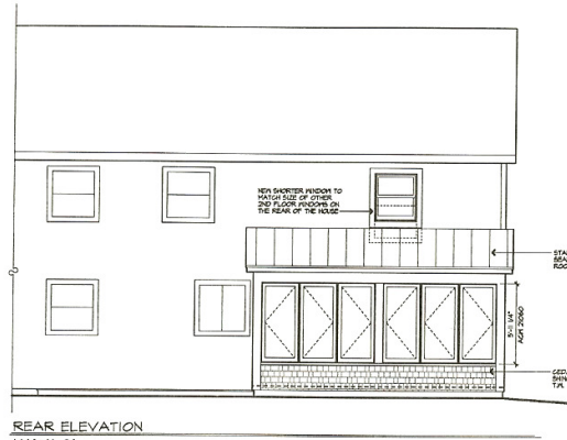
REAR ELEVATION 1/4" x 11'-0"
