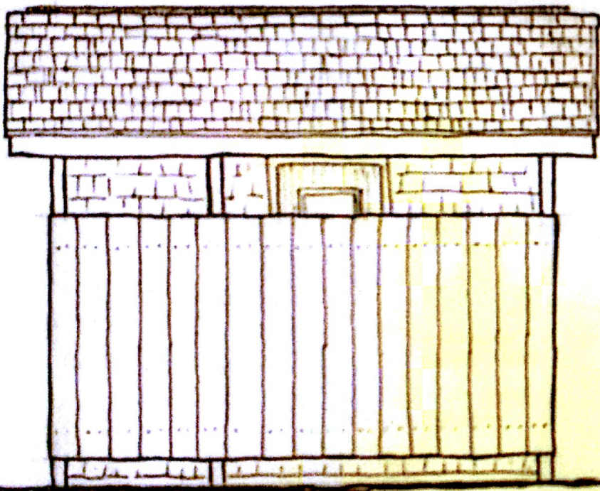
EAST ELEVATION SCALE 1/2" = 1'
