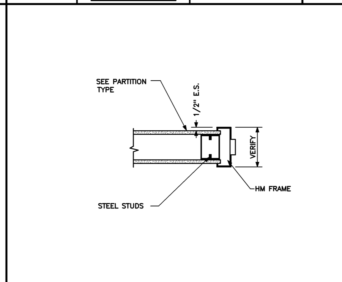
JAMB DETAIL 1 1/2" = 1'-0" 0 4' 8' 1' REF: NA
