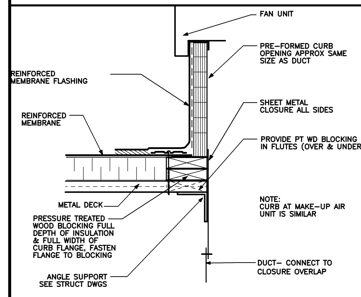
EXHAUST FAN CURB DETAIL 1 1/2" = 1'-0" 0 4' 8' 1' REF: NA
