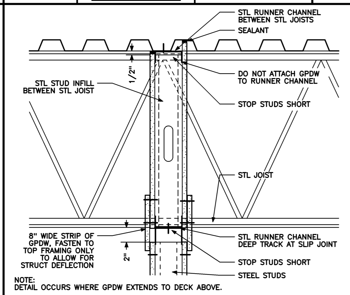
PARTITION PERPENDICULAR TO JOIST 1 1/2" = 1'-0" 0 4' 8' 1' REF: NA
