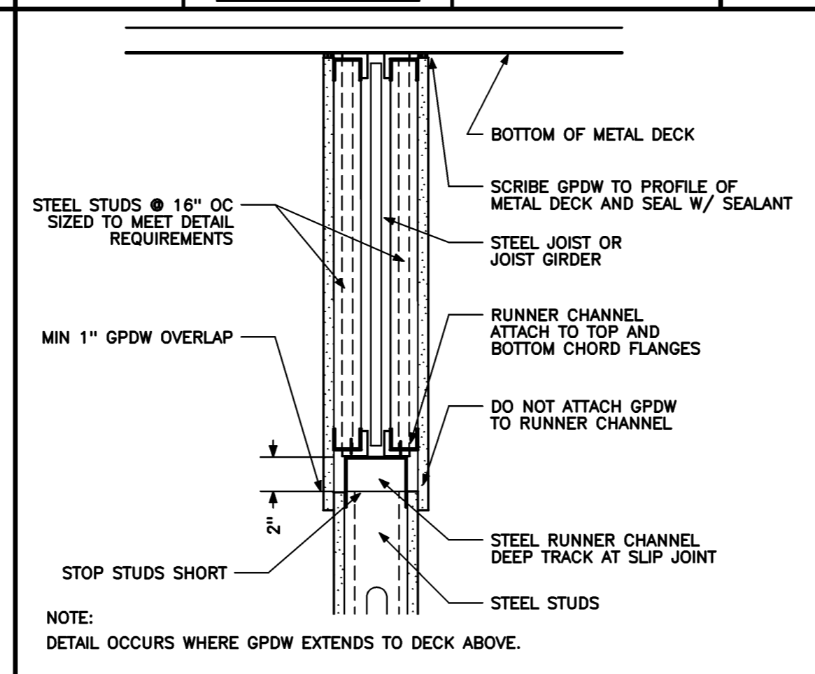
PARTITION TO UNDERSIDE OF JOIST 1 1/2" = 1'-0" 0 4' 8' 1' REF: NA
