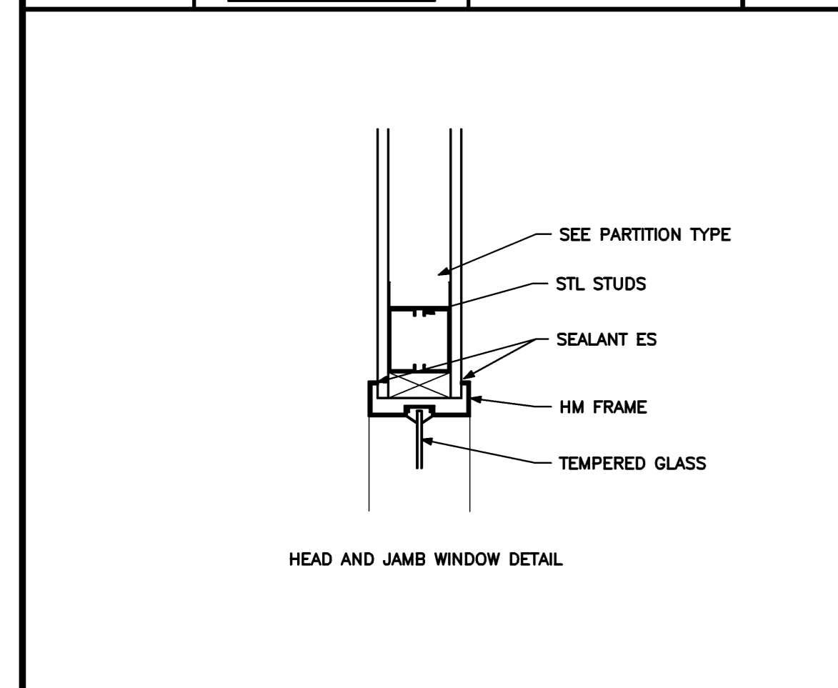
WINDOW DETAIL 1 1/2" = 1'-0" 0 4' 8' 1' REF: A10.1
