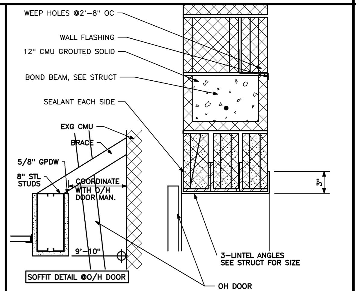
HEAD DETAIL & O/H DOOR SOFFIT DETAIL 1 1/2" = 1'-0" 0 4' 8' 1' REF: NA
