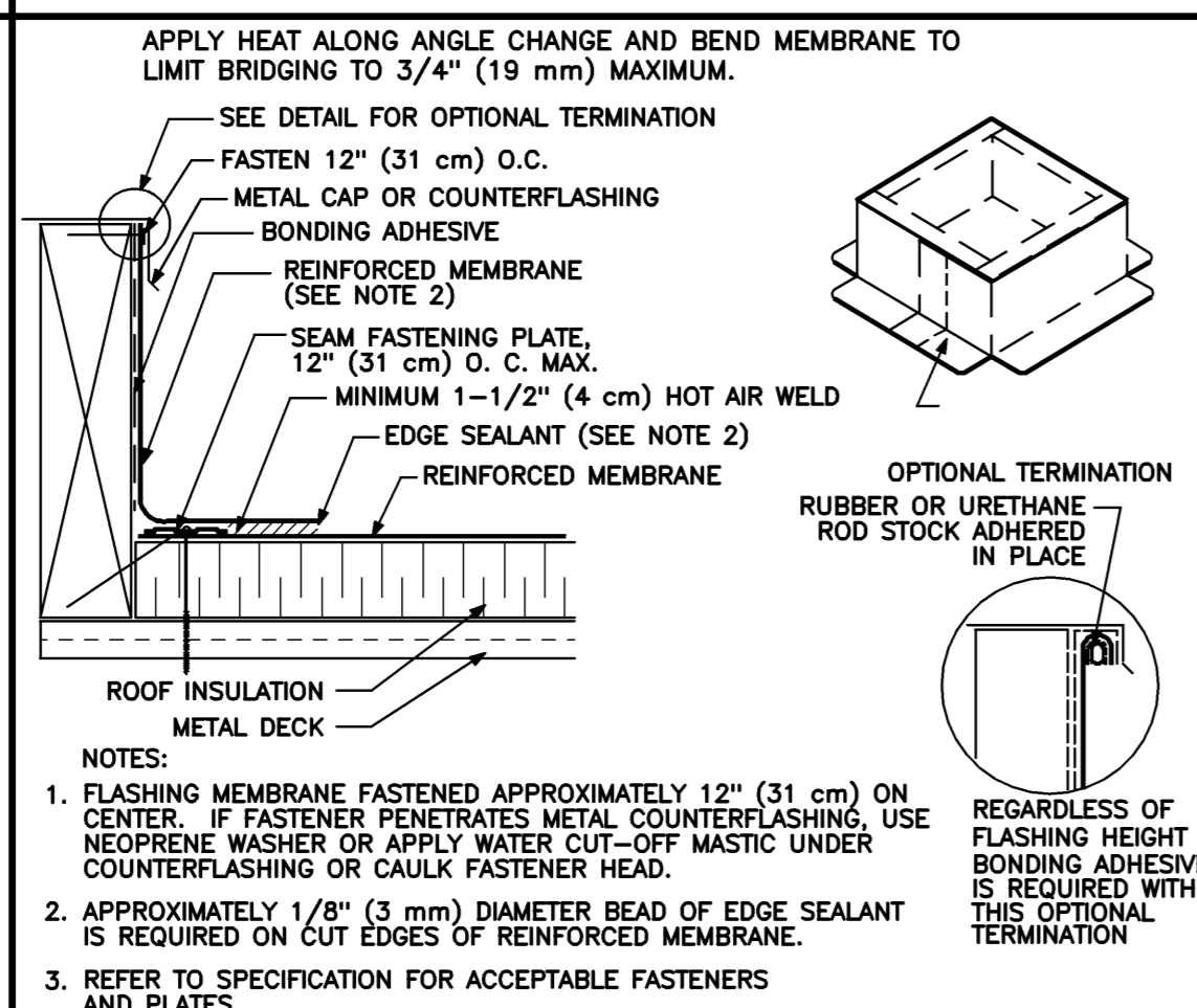
CURB FLASHING DETAIL 1 1/2" = 1'-0" 0 4' 8' 1' REF: NA
