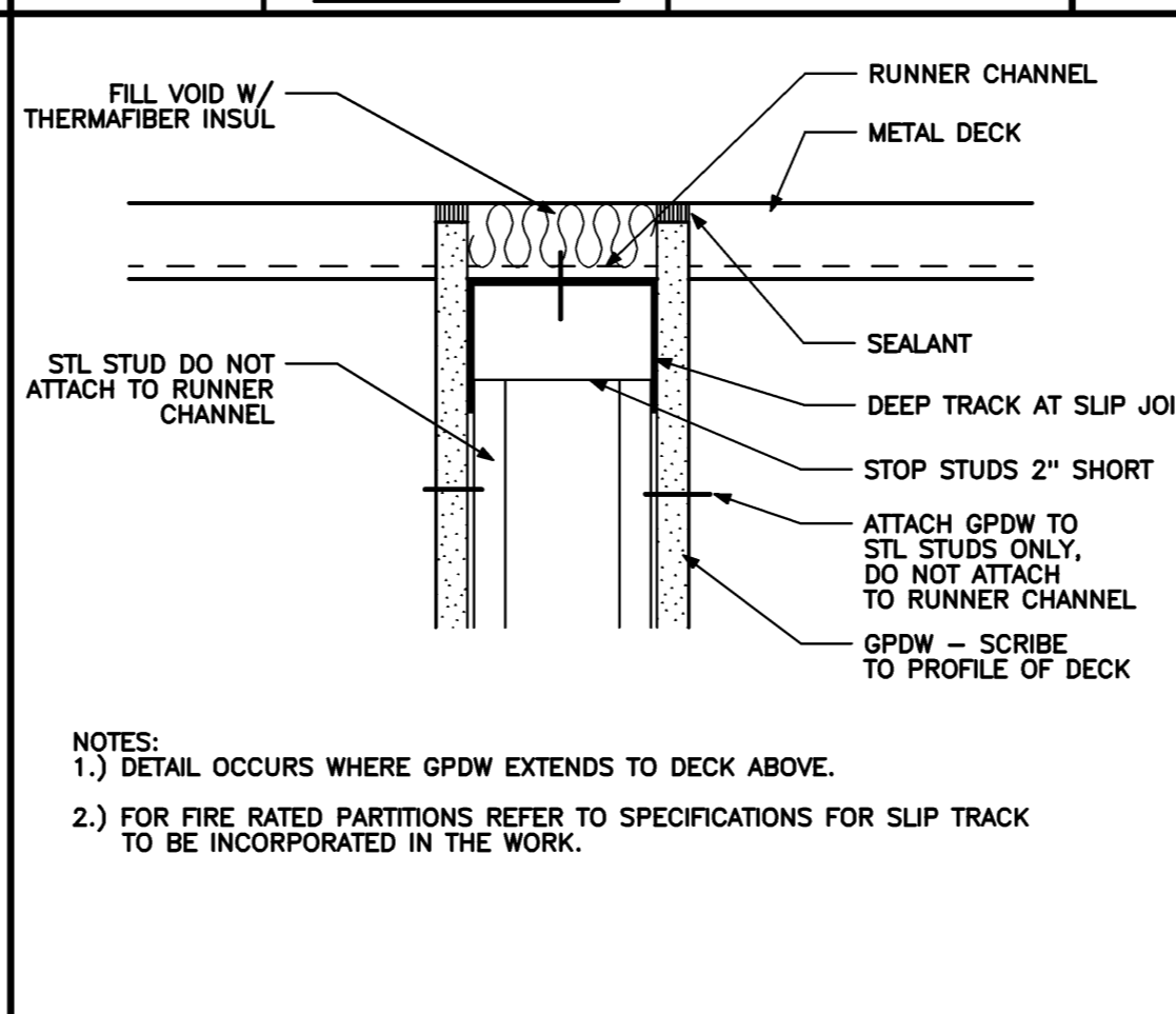
PARTITION PERPENDICULAR TO DECK 3" = 1'-0" 0 2' 4' 8' 1' REF: NA
