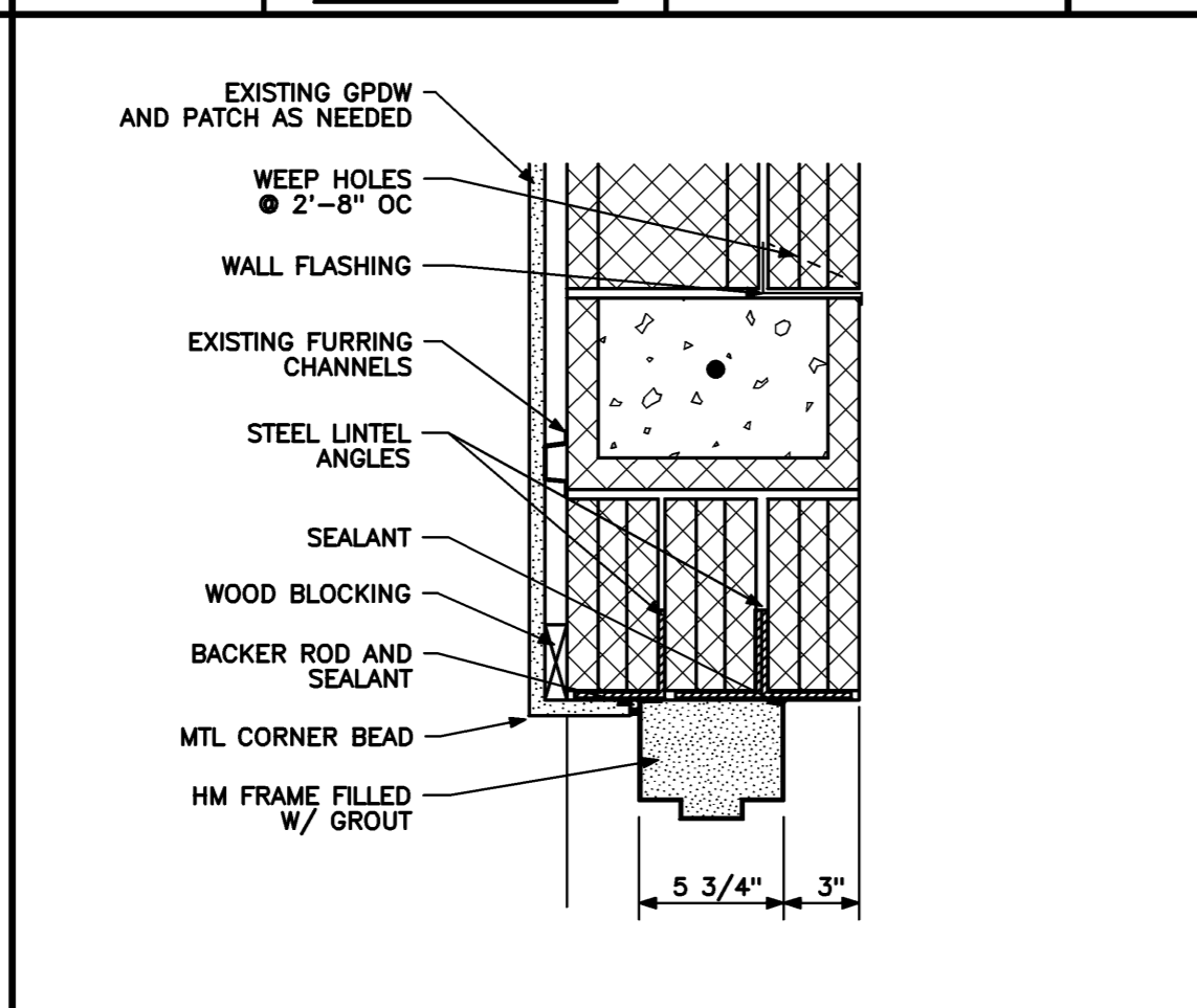
HEAD DETAIL 1 1/2" = 1'-0" 0 4' 8' 1' REF: NA
