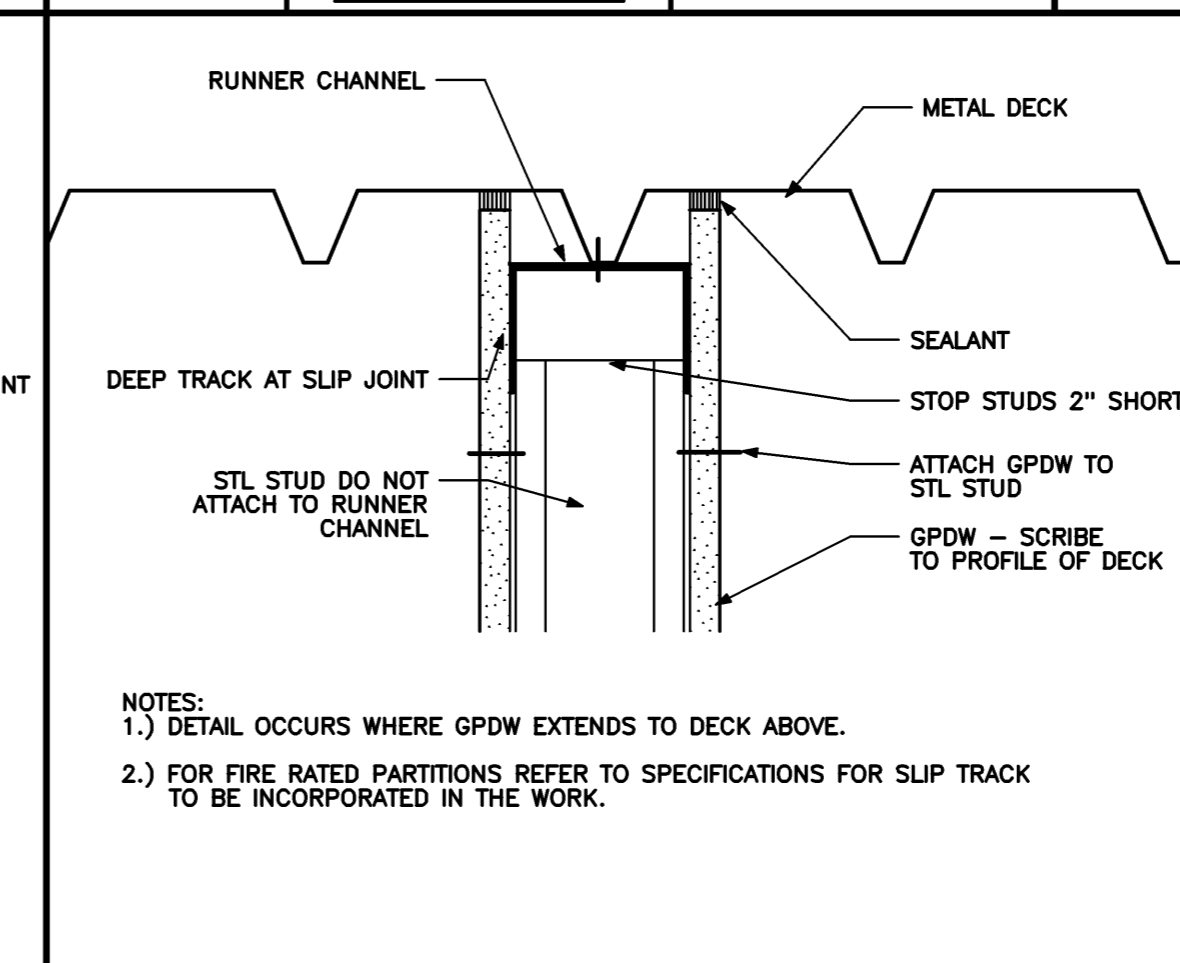
PARTITION PARALLEL TO DECK 3" = 1'-0" 0 2' 4' 8' 1' REF: NA
