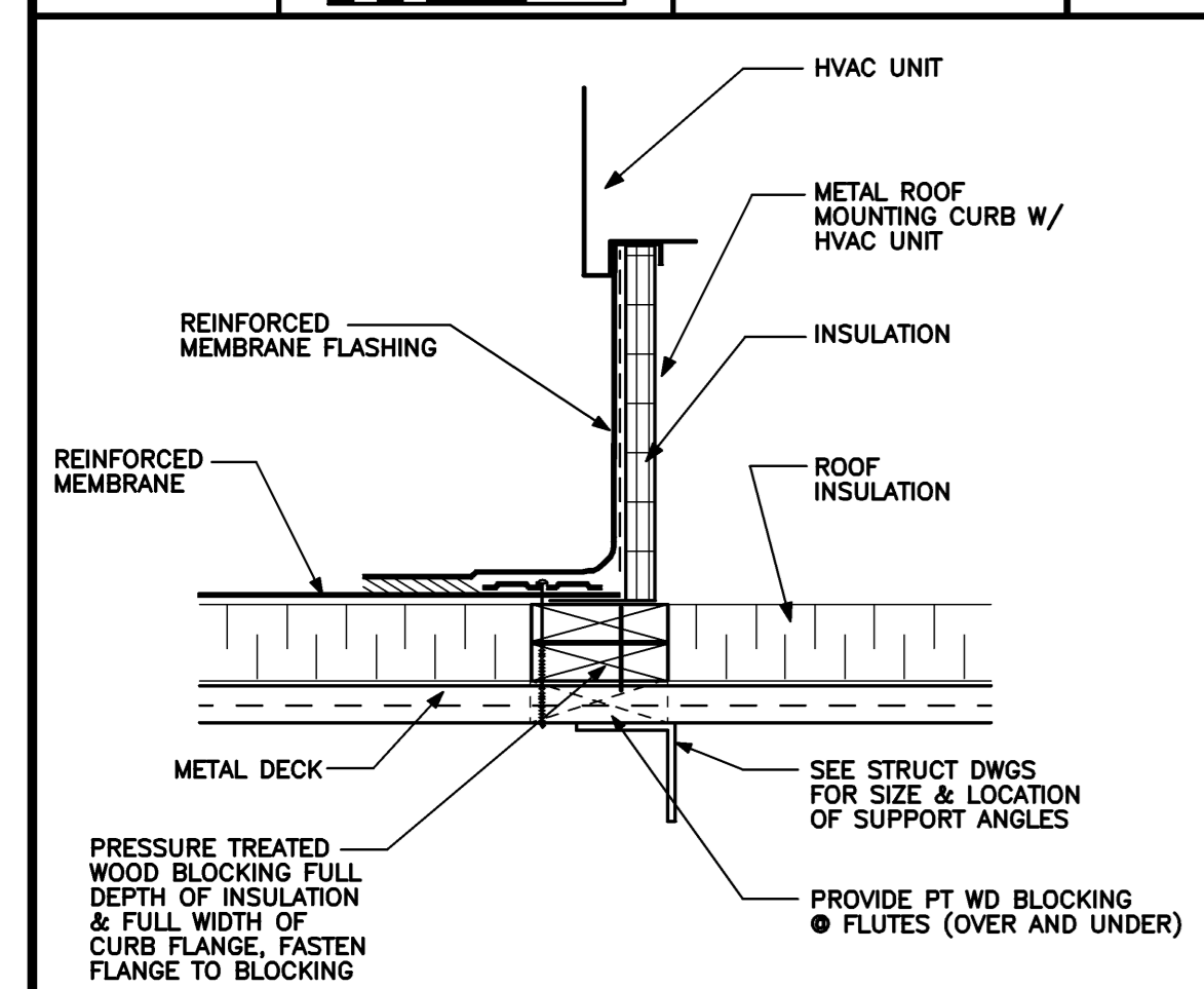
HVAC CURB DETAIL 1 1/2" = 1'-0" 0 4' 8' 1' REF: NA
