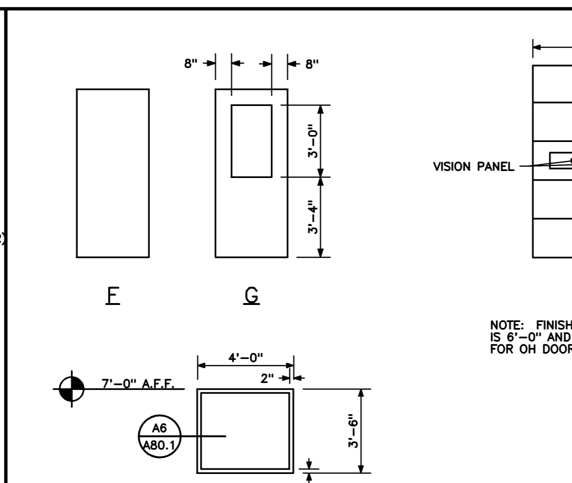
INTERIOR WINDOW AT OFFICE #2 1 1/2" = 1'-0" 0 4' 8' 1' REF: NA
