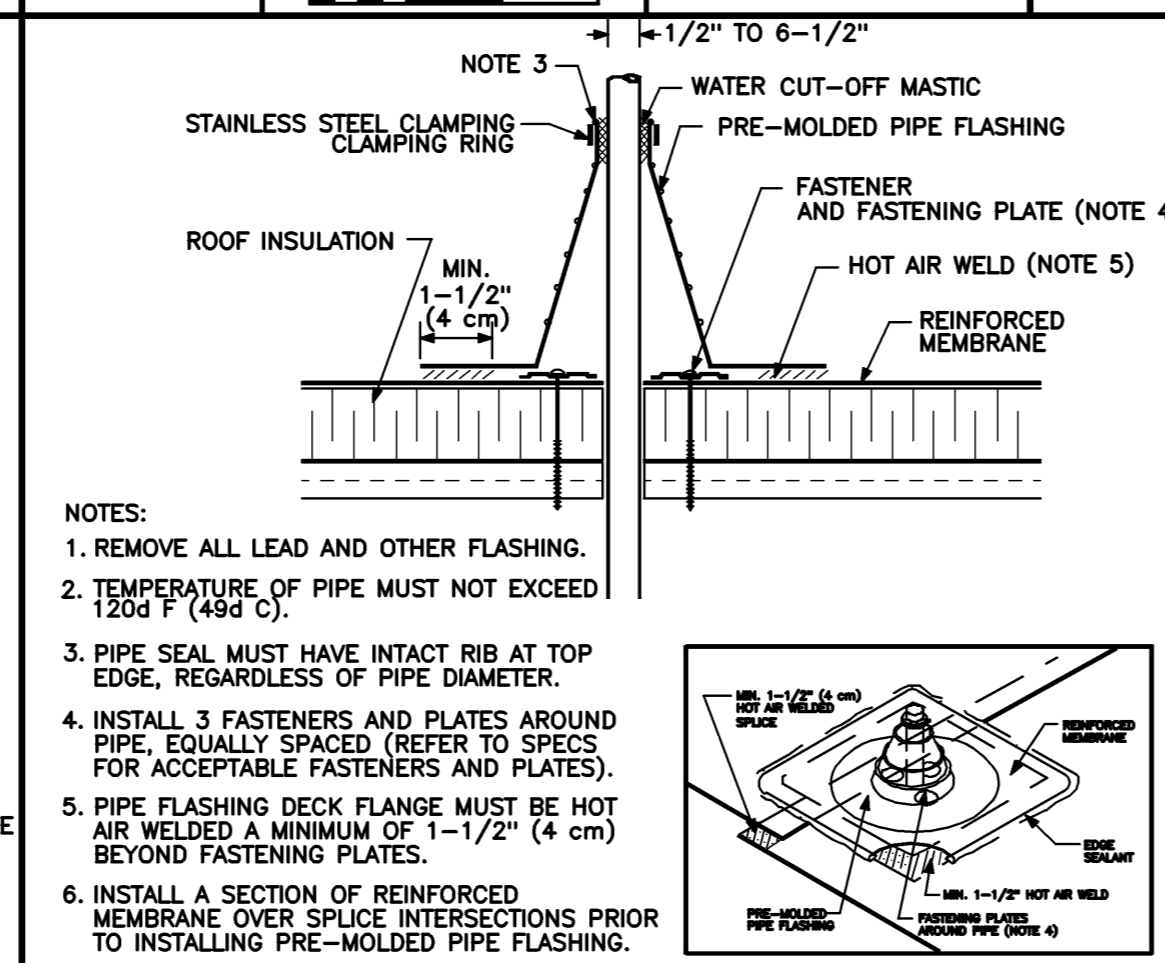
PIPE/VENT FLASHING DETAIL 1 1/2" = 1'-0" 0 4' 8' 1' REF: NA
