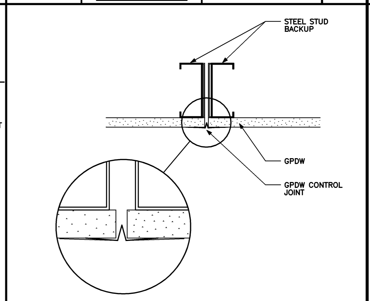
TYPICAL GYP BD CONTROL JOINT DETAIL 3" = 1'-0" 0 2' 4' 8' 1' REF: NA
